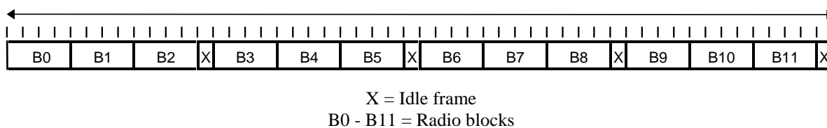
Figure 2a1: 52- multiframe for PDCH/Fs
