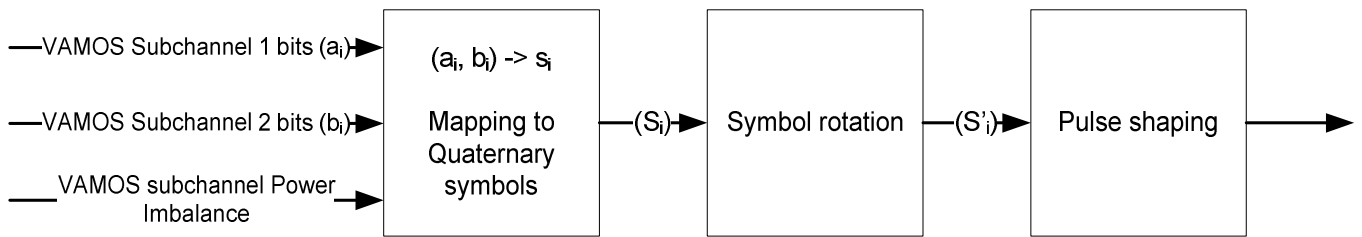
Figure 6: AQPSK Modulation to map bits from a VAMOS pair on a burst in downlink
