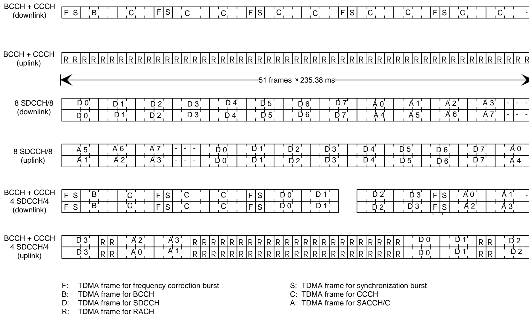
Figure 3: Channel organization in the 51-frame multiframe
