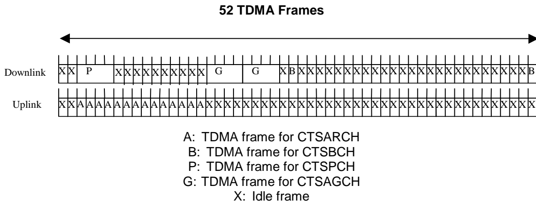
Figure 2b: 52-multiframe for CTS.
