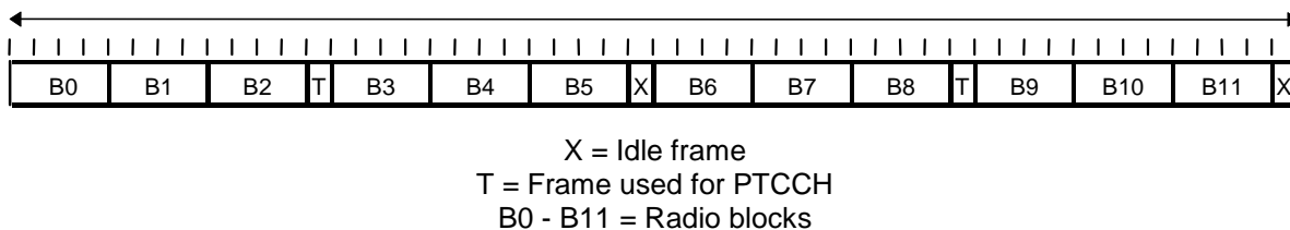
Figure 2a1: 52- multiframe for PDCH/Fs in BTTI configuration.
