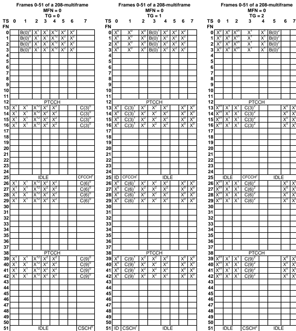
Figure D.4: COMPACT downlink 52-multiframe structure using 3 time groups for large cells (based on an assignment of 1 CPBCC and 3 CPCCs with NIB_CCCH_0 = NIB_CCCH_1 = NIB_CCCH_2 = 4, NIB_CCCH_3 = 0). NIB_CCCH is not broadcast for serving cell time group
