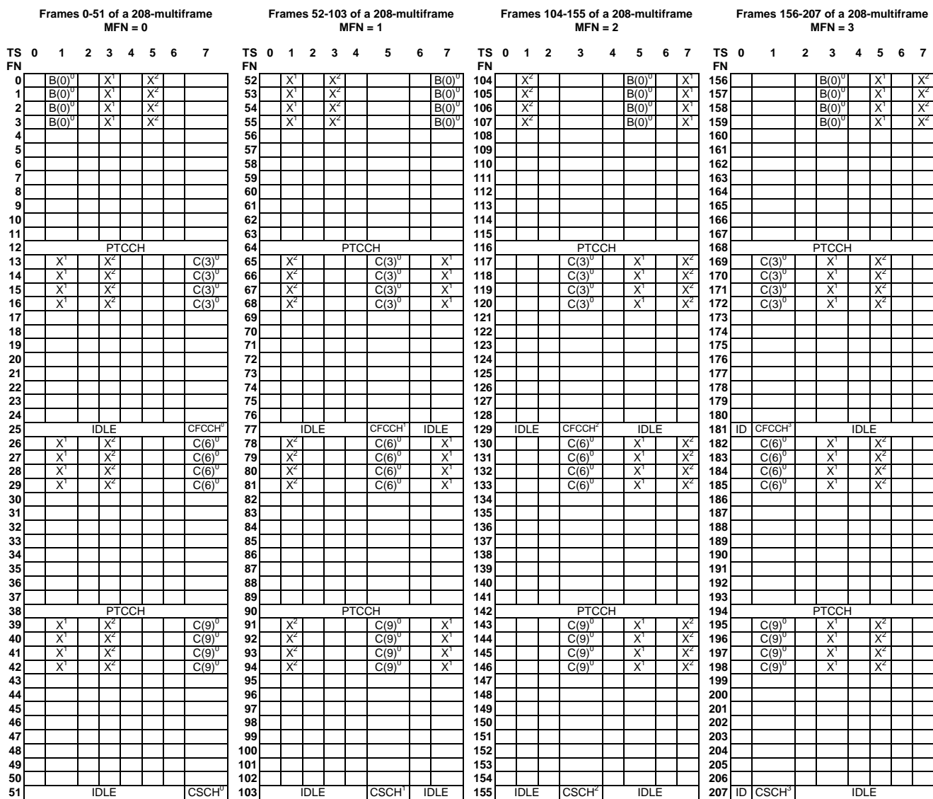
Figure D.6: Example of COMPACT downlink timeslot mapping and rotation of control channels using 3 time groups for nominal cells (based on an assignment of 1 CPBCCCH and 3 CPCCCHs with NIB_CCCH_0 = NIB_CCCH_1 = NIB_CCCH_2 = 4, NIB_CCCH_3 = 0). TG = 0 is illustrated. NIB_CCCH is not broadcast for serving cell time group
