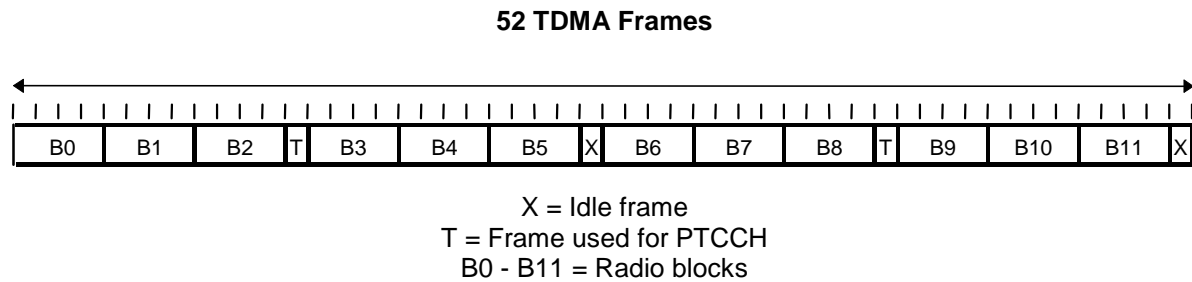
Figure 9: 52- multiframe for PDCHs -
