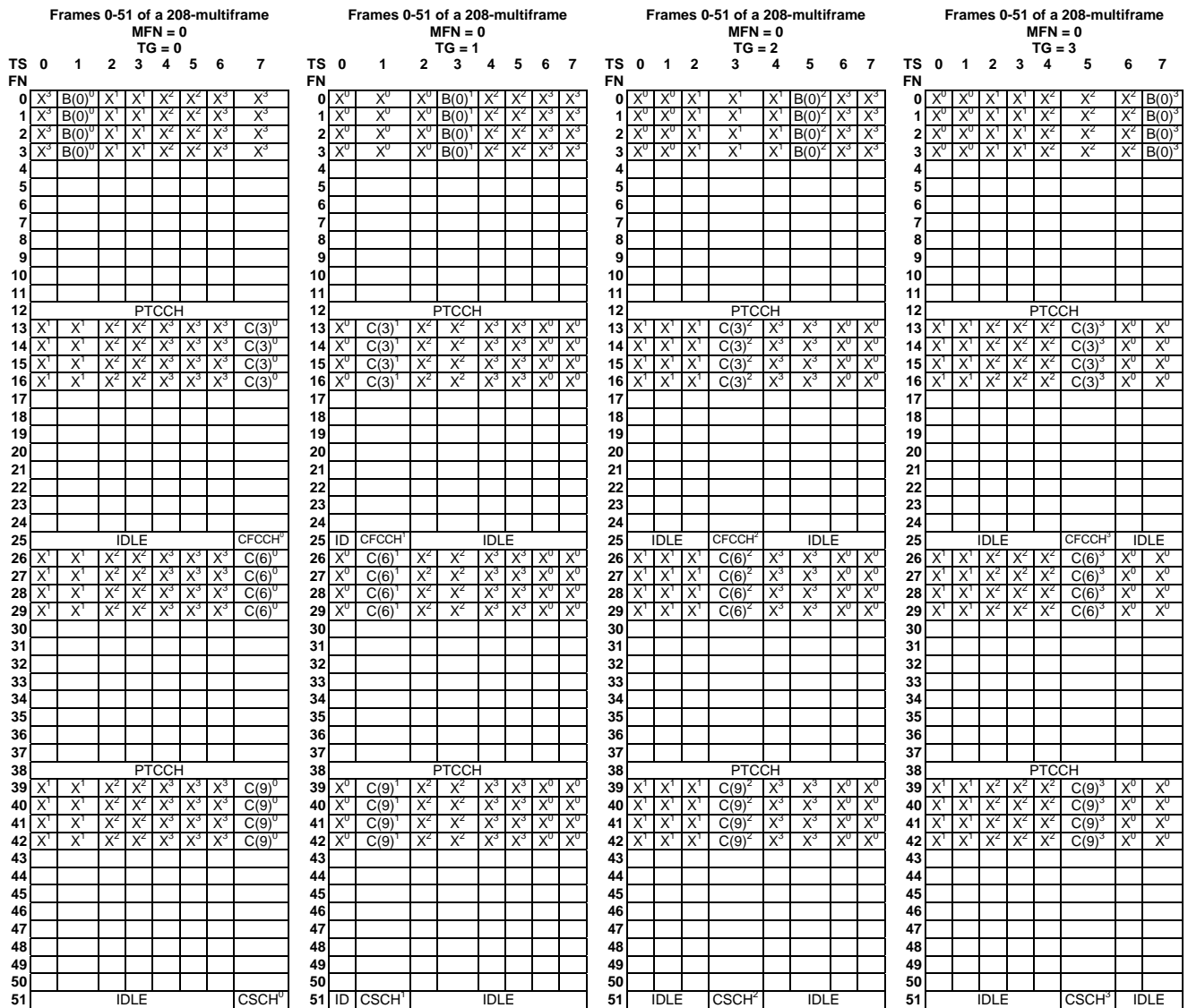
Figure D.3: COMPACT downlink 52-multiframe structure using 4 time groups for large cells (based on an assignment of 1 CPBCH and 3 CPCCCHs with NIB_CCCH_0 = NIB_CCCH_1 = NIB_CCCH_2 = NIB_CCCH_3 = 4). NIB_CCCH is not broadcast for serving cell time group
