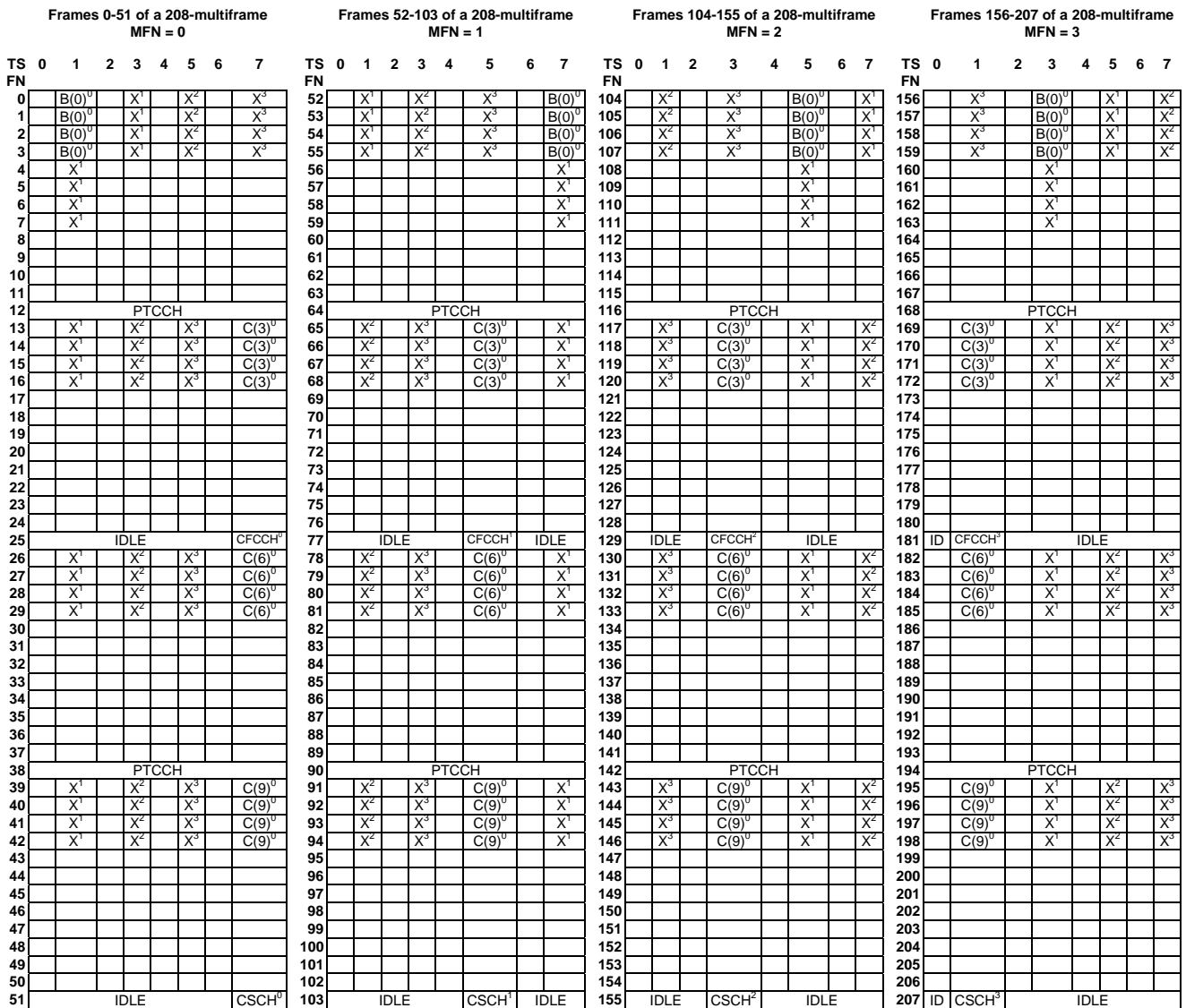
Figure D.7: Example of COMPACT downlink timeslot mapping and rotation of control channels using 4 time groups for nominal cells (based on an assignment of 1 CPBCC and 3 CPCCCHs with NIB_CCCH_0 = NIB_CCCH_2 = NIB_CCCH_3 = 4, NIB_CCCH_1 = 5). TG = 0 is illustrated. NIB_CCCH is not broadcast for serving cell time group
