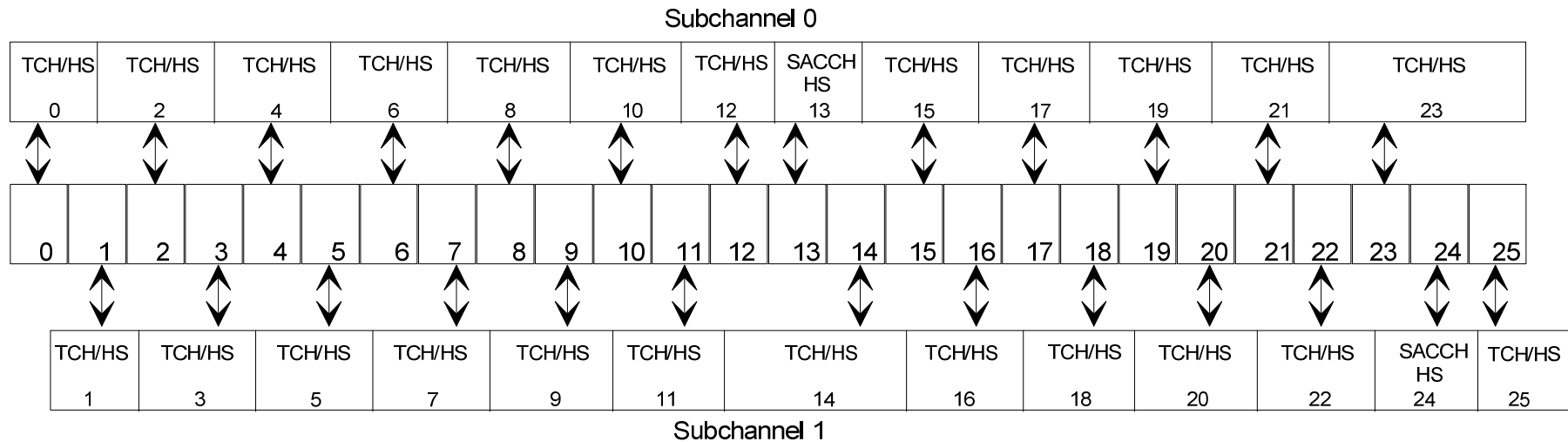
Figure 7d: TDMA frame mapping for TCH/HS + SACCH/HS sub-channels 0 and 1 for VAMOS II and VAMOS III MS when assigned a training sequence in TSC Set 2
