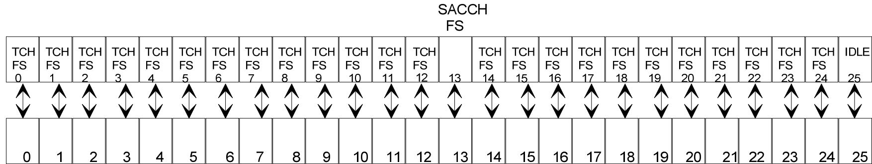
Figure 7c: TDMA frame mapping for TCH/FS + SACCH/FS for VAMOS II and VAMOS III MS when assigned a training sequence in TSC Set 2
