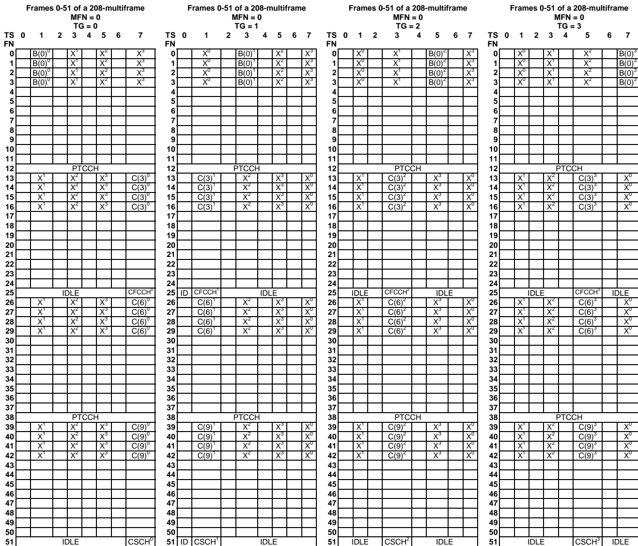
Figure D.1: COMPACT downlink 52-multiframe structure using 4 time groups for nominal cells (based on an assignment of 1 CPBCH and 3 CPCCCHs with NIB\_CCCH\_0 = NIB\_CCCH\_1 = NIB\_CCCH\_2 = NIB\_CCCH\_3 = 4 ). NIB\_CCCH is not broadcast for serving cell time group
