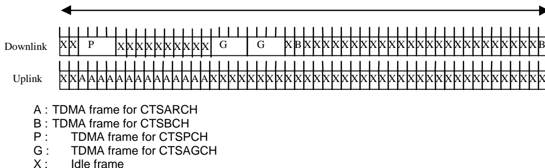
Figure 10: 52-multiframe for CTS
