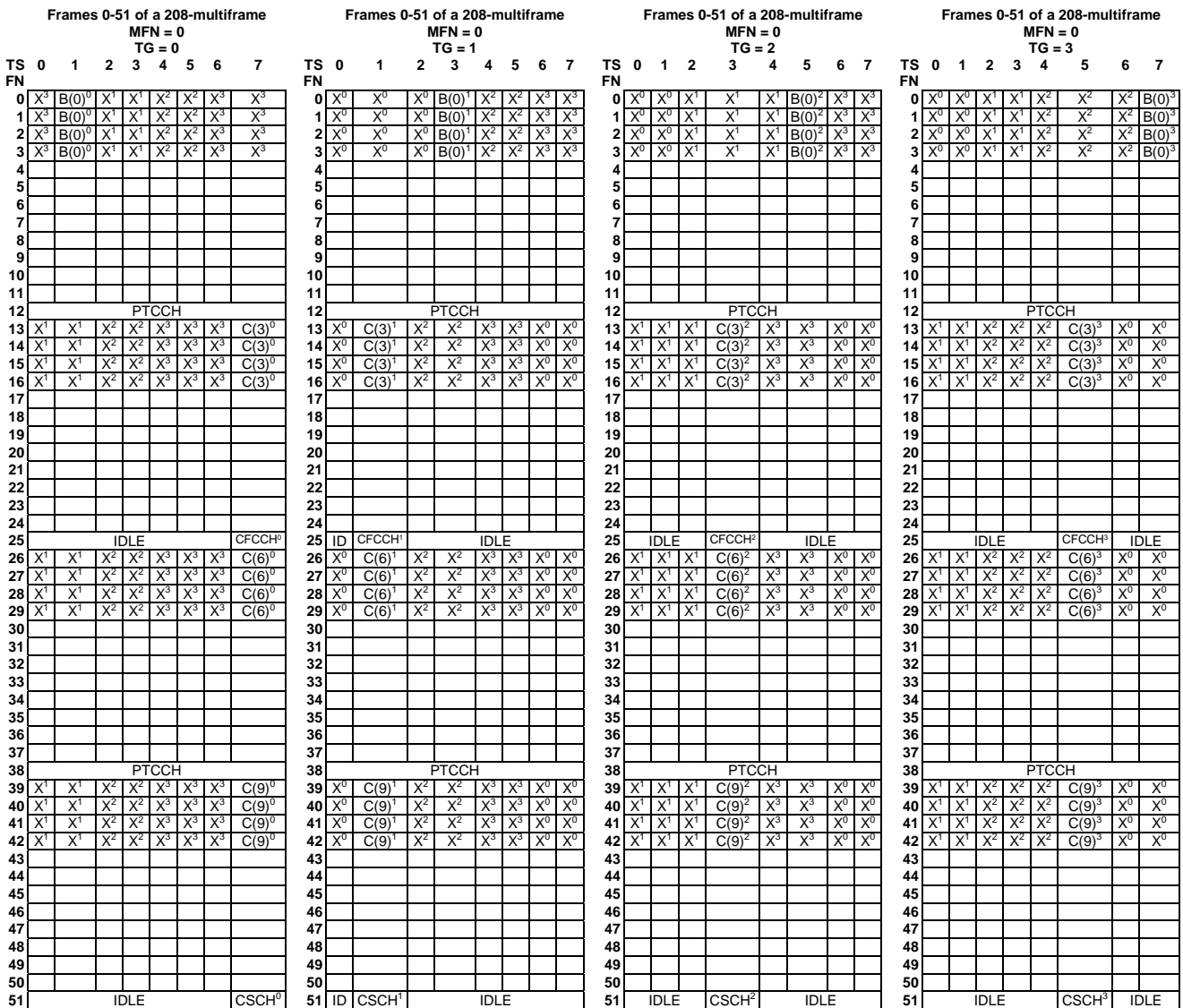
Figure D.3: COMPACT downlink 52-multiframe structure using 4 time groups for large cells (based on an assignment of 1 CPBCC and 3 CPCCCHs with NIB_CCCH_0 = NIB_CCCH_1 = NIB_CCCH_2 = NIB_CCCH_3 = 4). NIB_CCCH is not broadcast for serving cell time group
