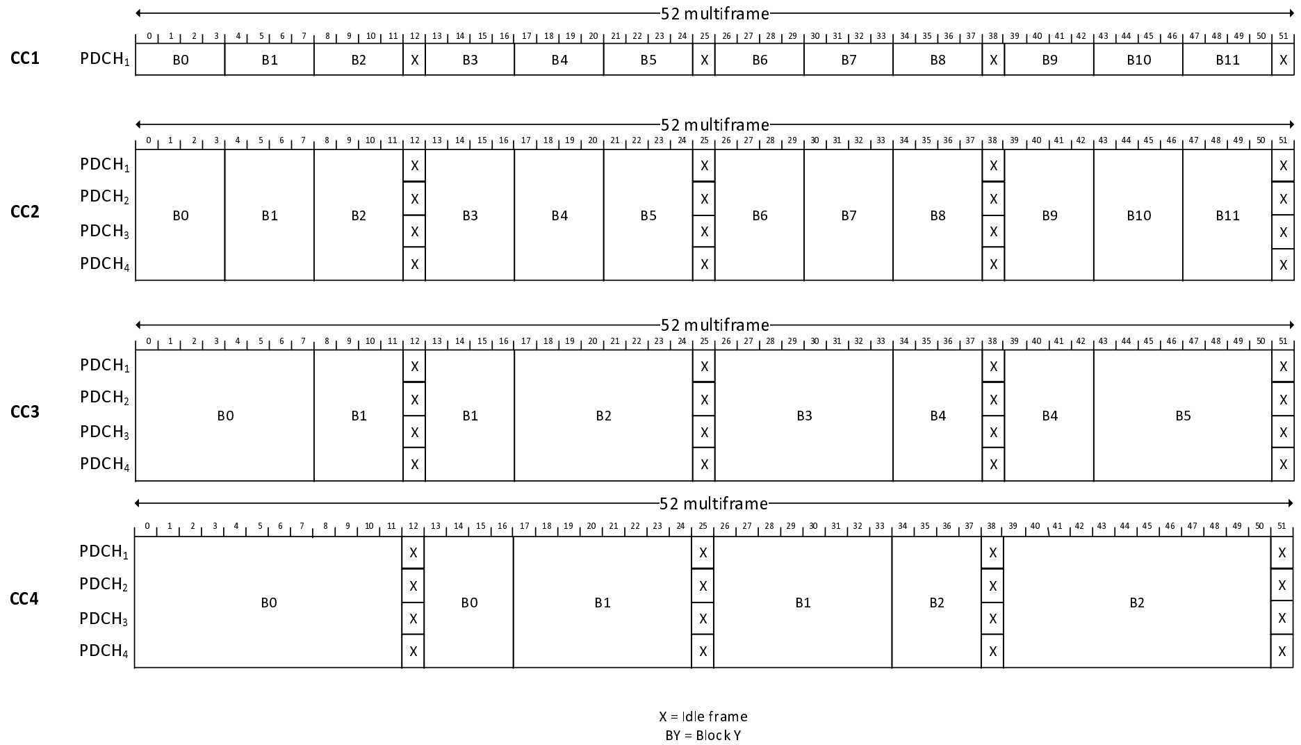
Figure 9b: 52-multiframe for EC-GSM-IoT for different Coverage Classes (CC)
