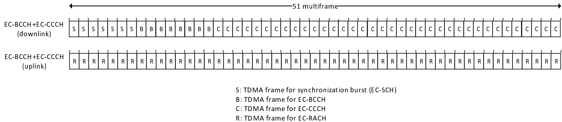
Figure 8c: TDMA Frame mapping for EC-SCH+EC-BCCH+EC-CCCH
