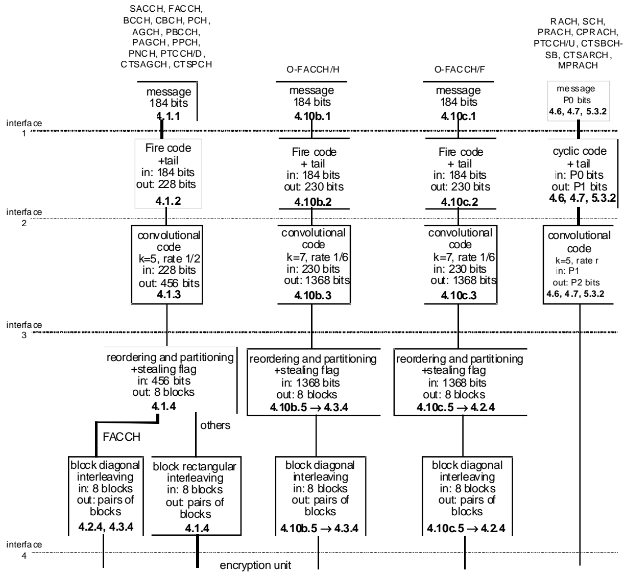
Figure 2: Channel Coding and Interleaving Organization for control channels except PACCH
