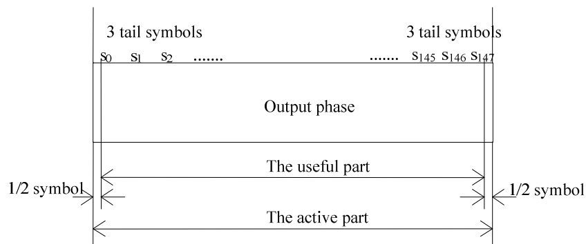
Figure 4: Relation between active part of burst and tail symbols. For the normal burst the useful part lasts for 147 modulating symbols.
