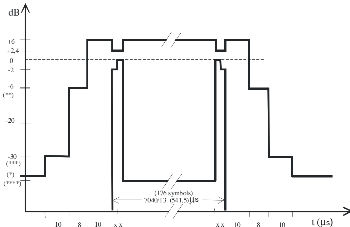
Figure B.7: Time mask for normal duration bursts (NB) at 16-QAM and 32-QAM modulation at higher symbol rate
