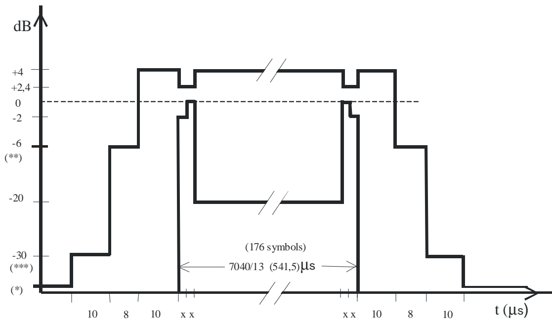
Figure B.6: Time mask for normal duration bursts (NB) at QPSK modulation at higher symbol rate
