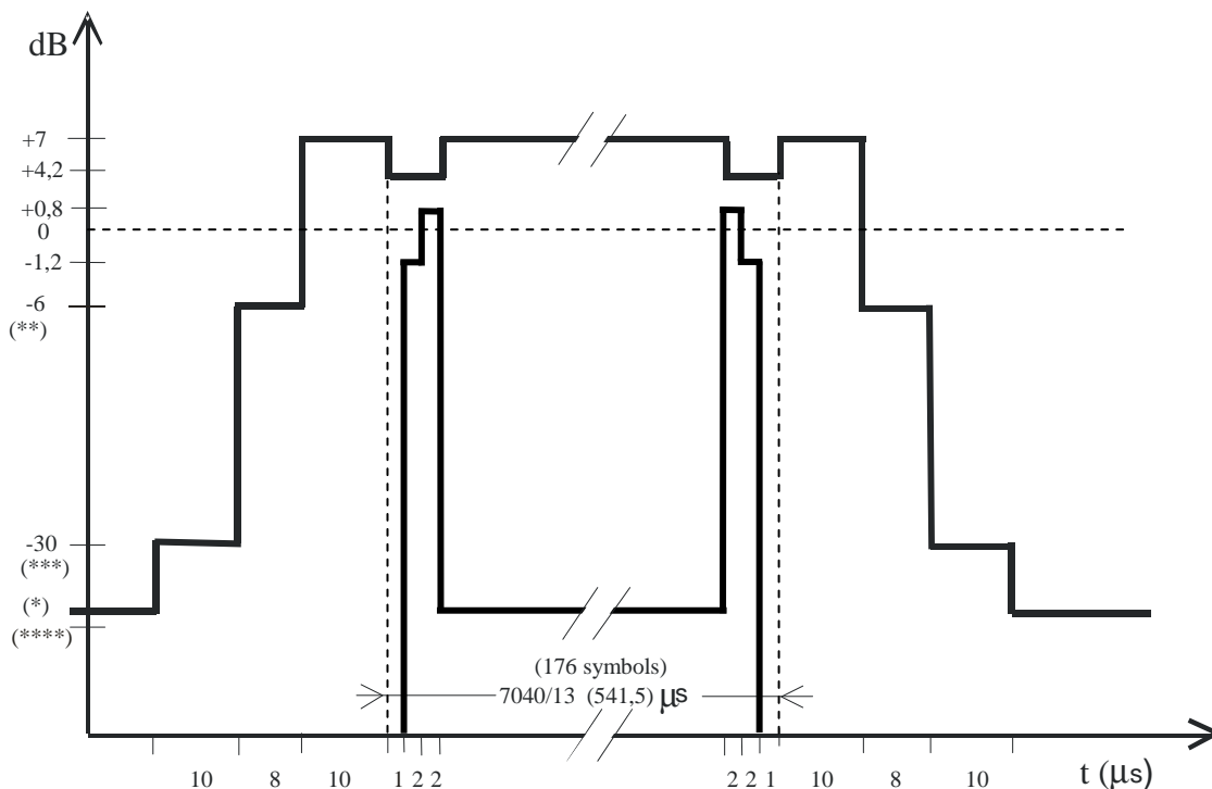
Figure B.7: Time mask for higher symbol rate bursts (HB) at 16-QAM and 32-QAM modulation with narrow pulse shaping filter
