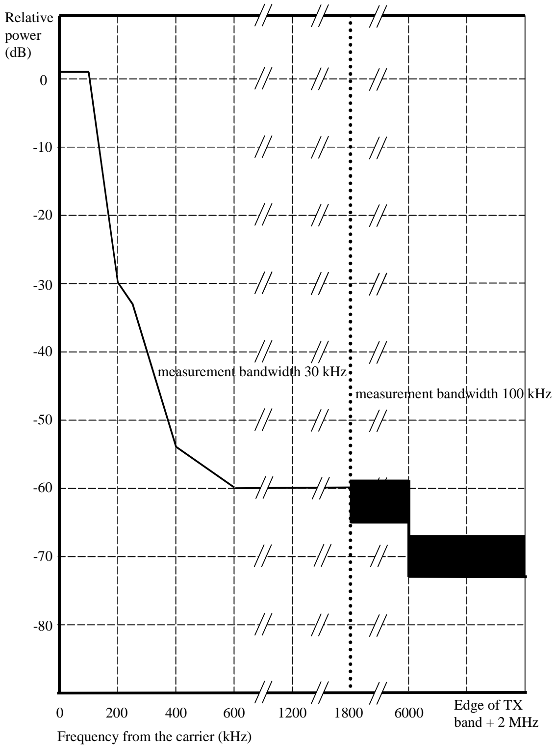
Figure A.3b: DCS 1 800 and PCS 1900 MS spectrum due to 8-PSK and 16-QAM modulation with normal symbol rate and QPSK, 16-QAM and 32-QAM with higher symbol rate modulation using narrow pulse shaping filter
