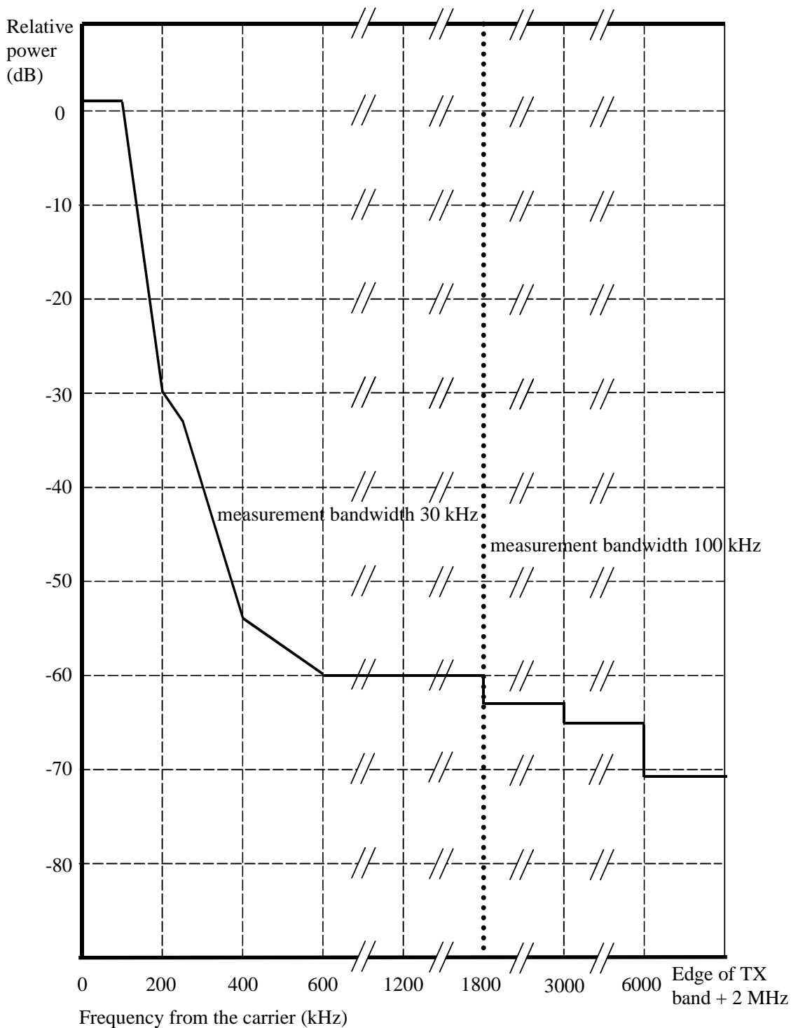
Figure A.1b: GSM 400, GSM 900, GSM 850 and GSM 700 MS spectrum due to 8-PSK and 16-QAM modulation with normal symbol rate and QPSK, 16-QAM and 32-QAM modulation with higher symbol rate using narrow pulse shaping filter
