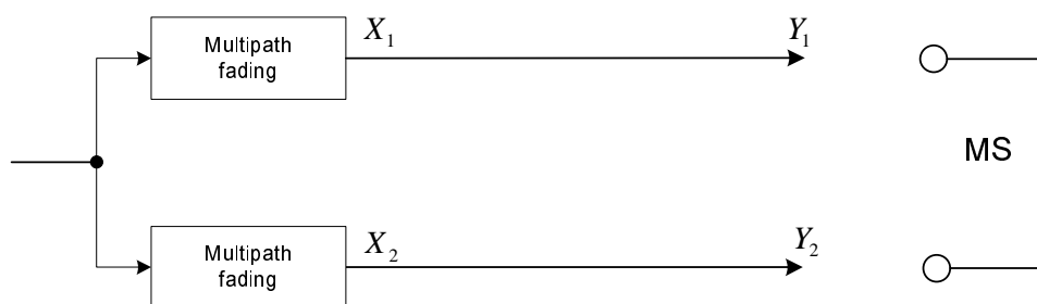
Figure N.3.1: Test setup when testing conformance to legacy requirements for MS having MSRD always enabled.
