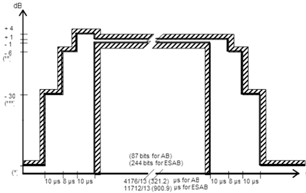
Figure B.3: Time mask for access bursts (AB) and extended synchronization access burst (ESAB)
