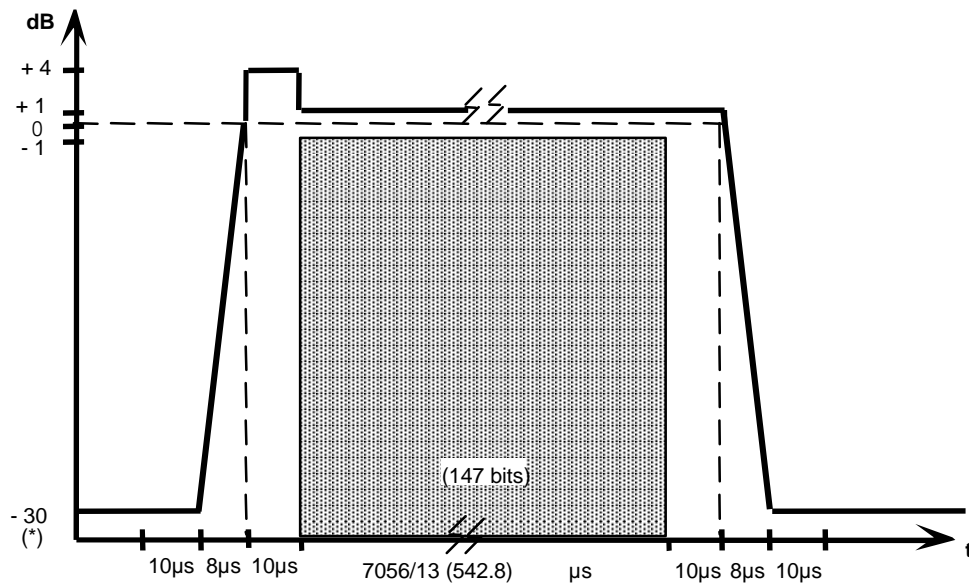
Figure B.3: Time mask for access bursts (AB) and extended synchronization access burst (ESAB)
