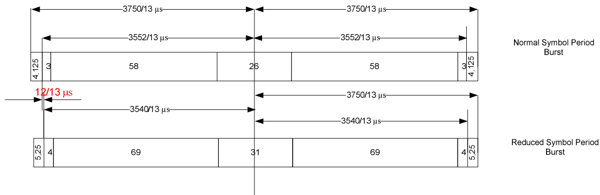
Figure 5.7.3: Timing alignment between normal symbol period and reduced symbol period bursts
