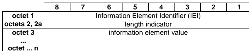
Figure 10.1.1/3GPP TS 48.016: Information element structure, TLV format
