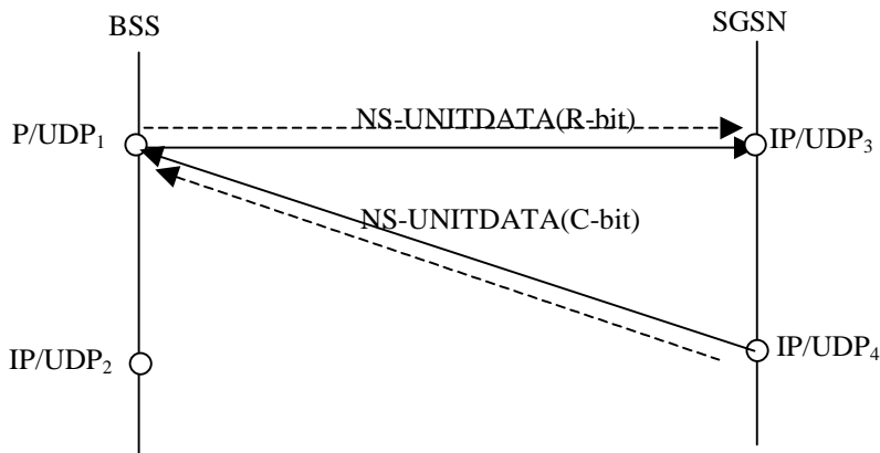
Figure B.2/3GPP TS 48.016: Example 2 of only one NS entity requesting change flow
