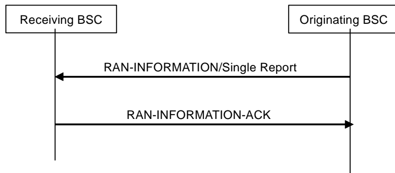
Fig 8c.2.3: Acknowledged Autonomous RAN Information Send procedure
