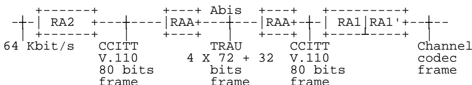
Figure 3GPP TS 48.060/4.3: Rate adaption when 16 kbit/s traffic channels are used
