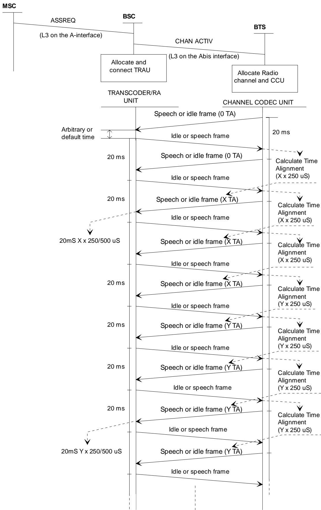
Figure 6.1: Initial Time Alignment Procedure
