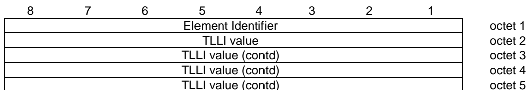
Figure 5.30.1: TLLI IE
