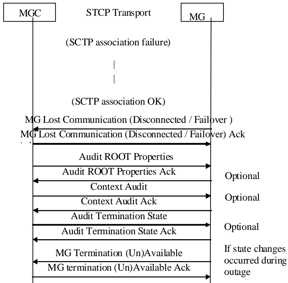
Figure 16: Control Association Failure and Recovery Procedures (SCTP)
