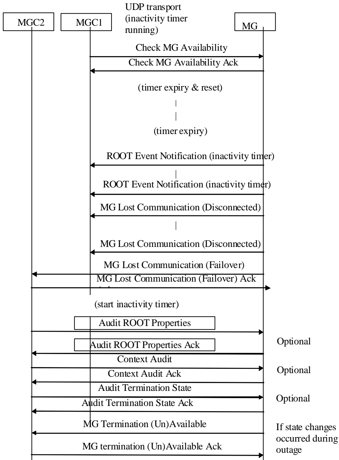
Figure 15: Control Association Failure and Recovery Procedures (UDP)
