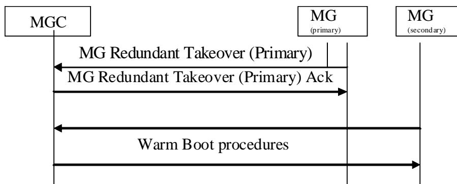
Figure 21: MG REDUNDANT TAKEOVER (PRIMARY) Procedure
