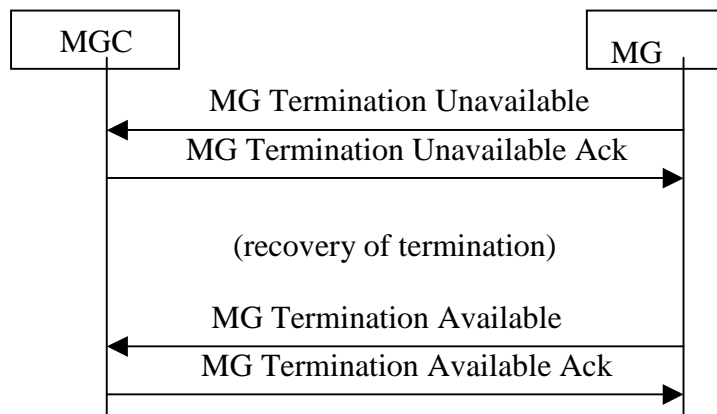
Figure 13: MG Termination Failure and Recovery Procedures
