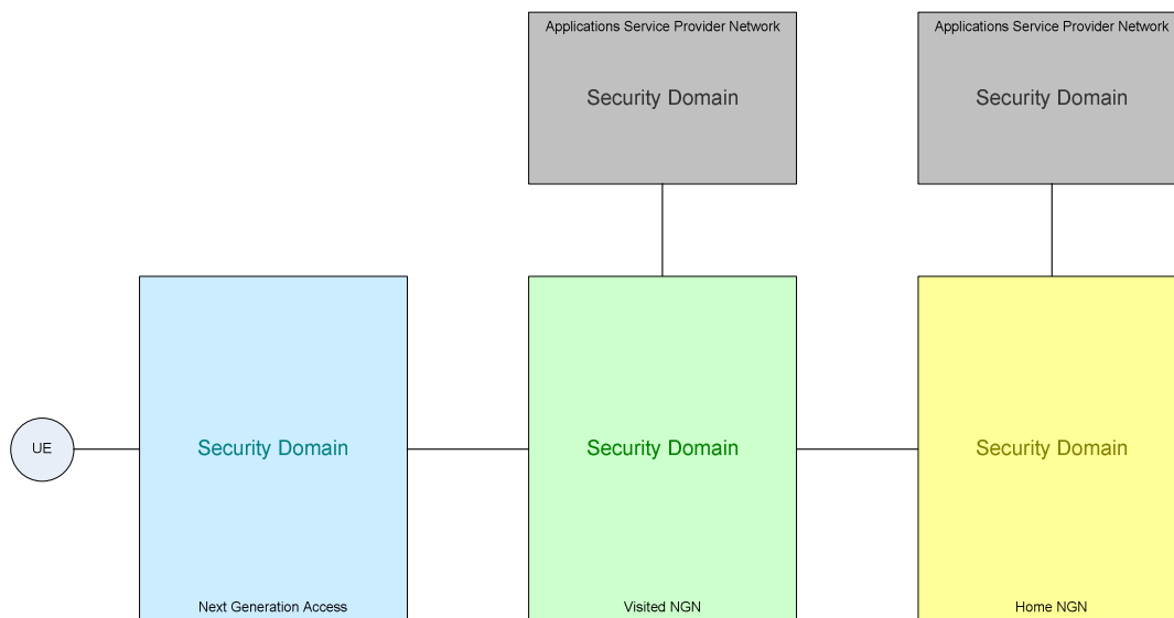
Figure 3: NGN security domains
