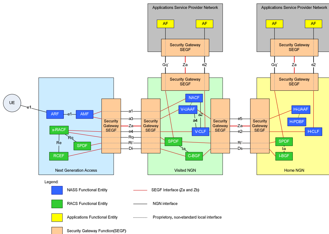
Figure 6: NGN security architecture with FEs and security gateway functional components around inter-domain interfaces in access, visited, home and other operator's networks
