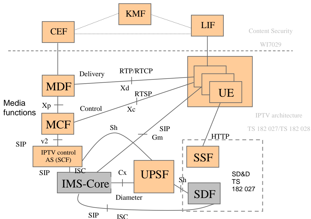
Figure F.4: Mapping Content Security to IPTV architecture
