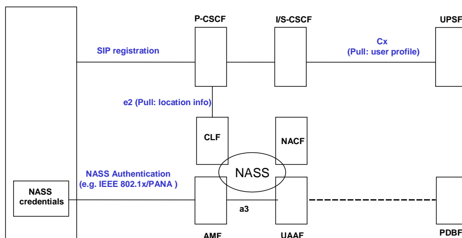
Figure 10: Formal mapping of NASS Bundled Authentication
