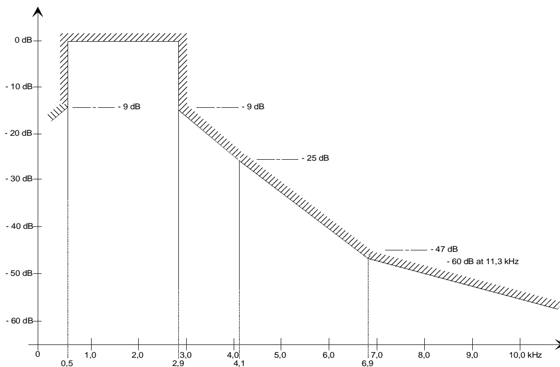
Figure A.1: Unwanted spectral components (VHF DSC encoder)
