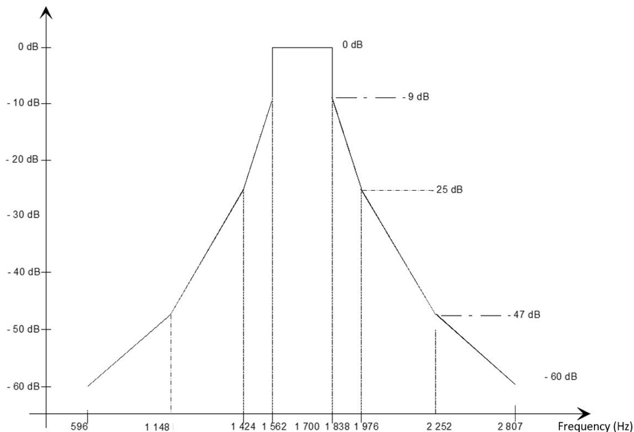
Figure A.2: Unwanted spectral components (MF/HF DSC encoder)
