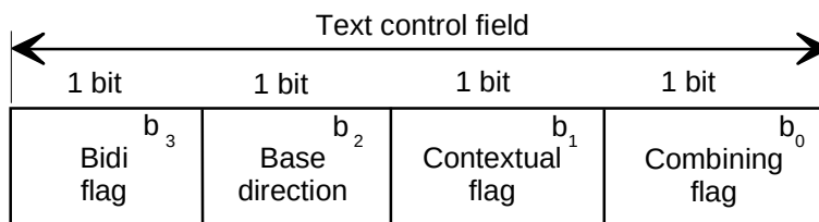
Figure 10a: Structure of the text control field
