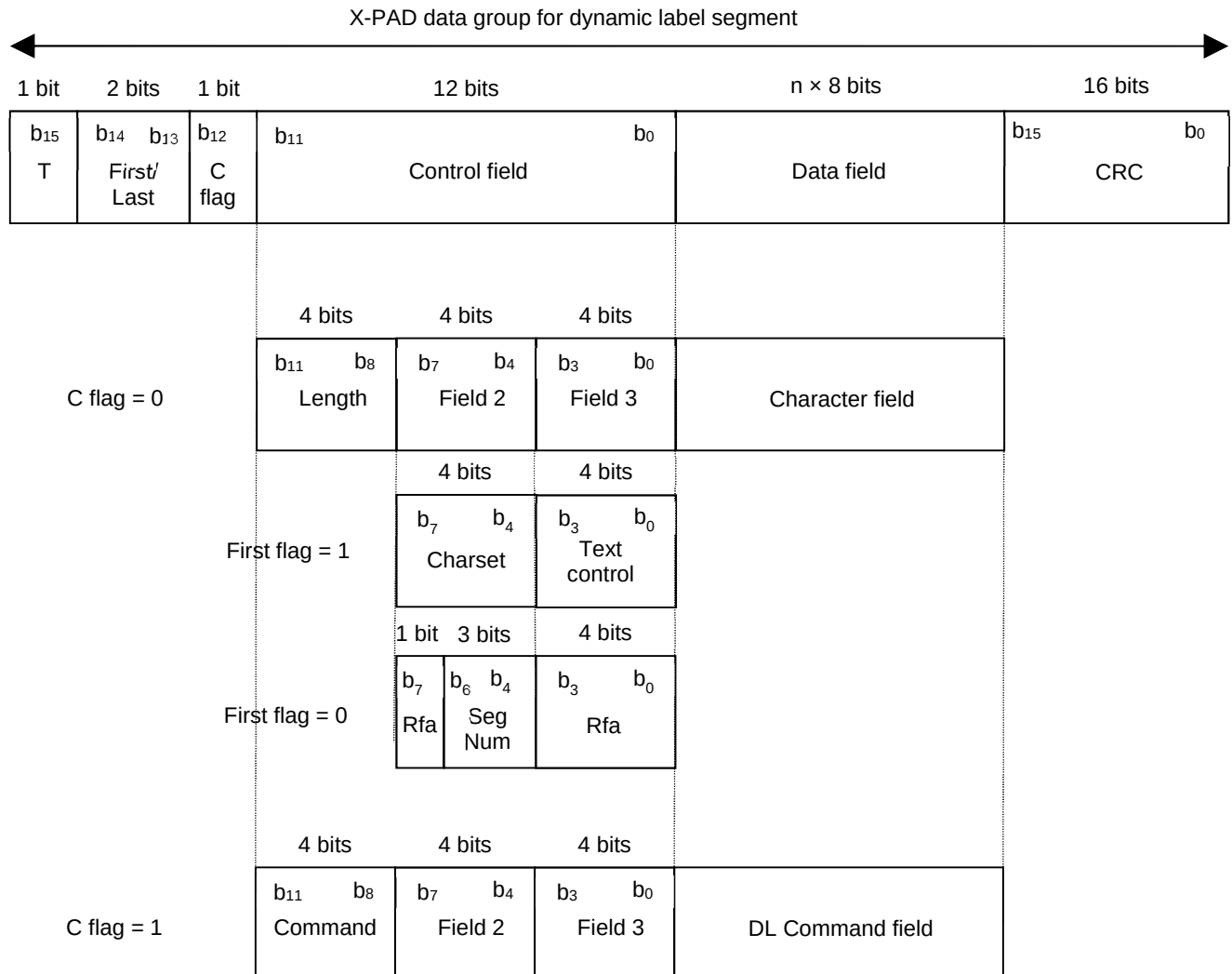
Figure 36: Structure of the X-PAD data group for each dynamic label segment
