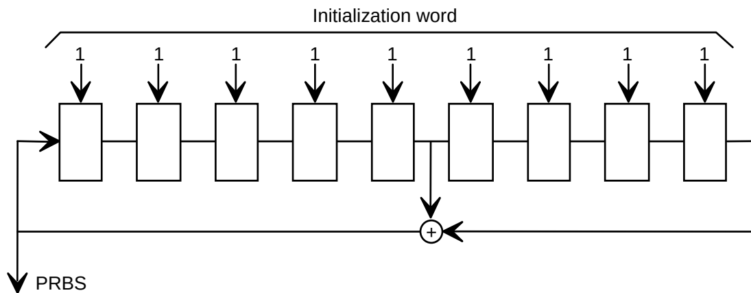
Figure 54: PRBS generator
