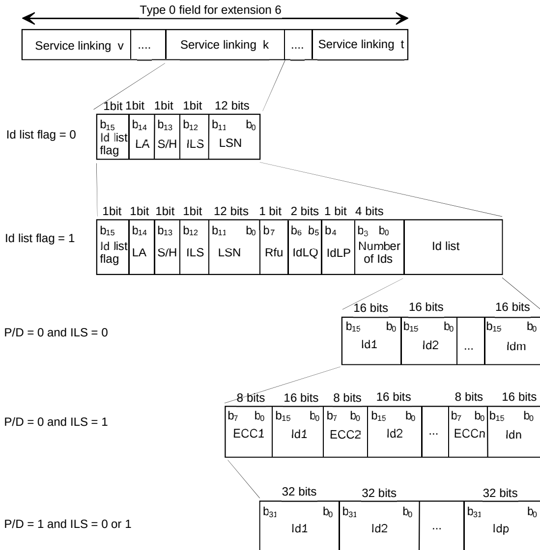
Figure 53: Structure of the Service linking field
