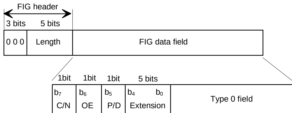
Figure 7: Structure of the FIG type 0 data field
