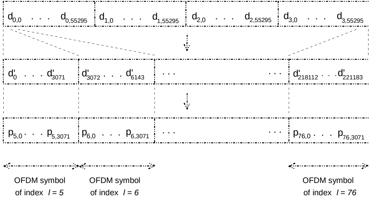
Figure 63: Block partitioning in the MSC for transmission mode I
