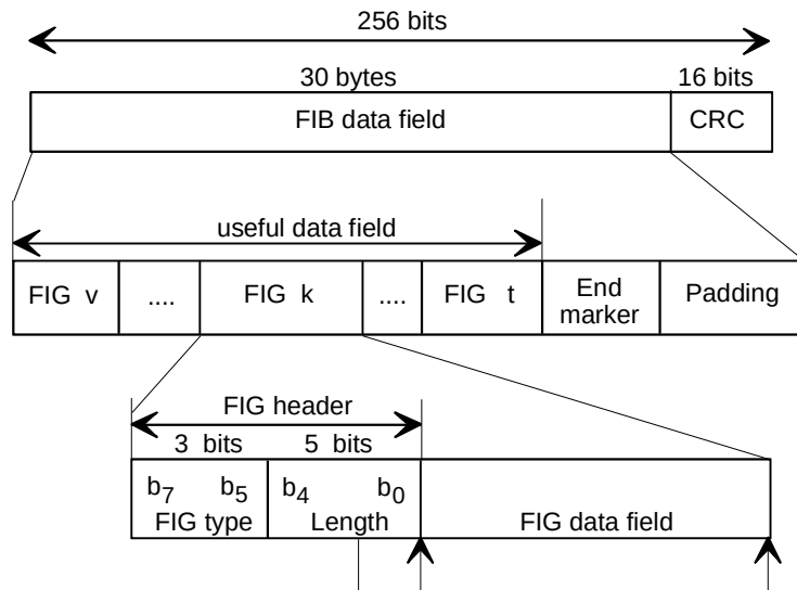
Figure 6: Structure of the FIB
