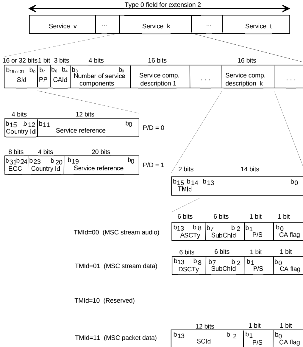
Figure 21: Structure of the service organization field
