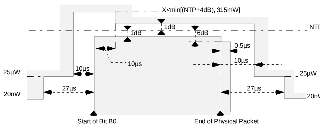
Figure 1a: GFSK modulated physical packet power-time template
