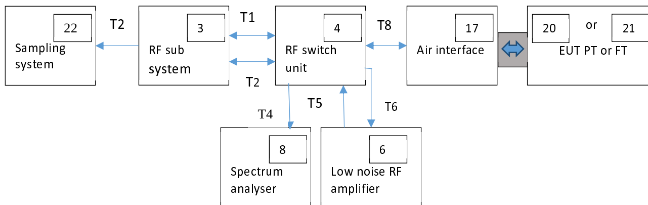
Figure 21: Test setup 4
