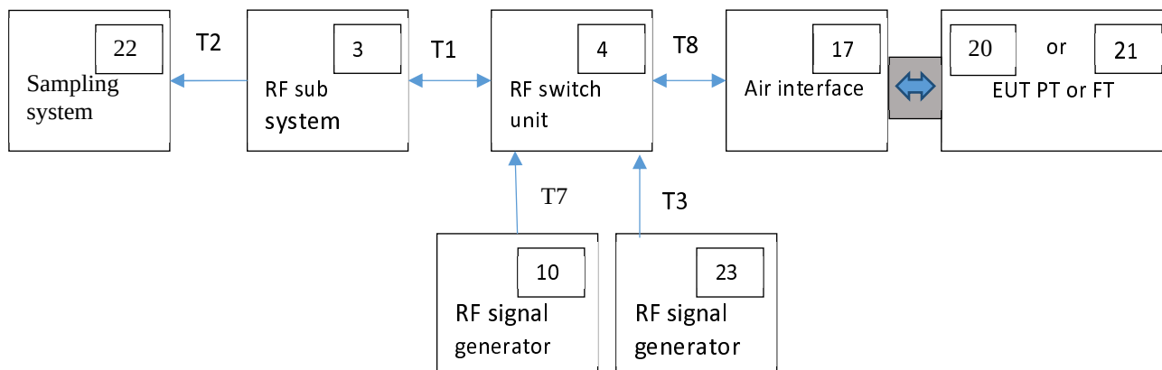
Figure 20: Test setup 3
