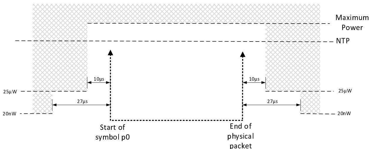
Figure 33b: Power-time template for non-constant envelope modulated packet
