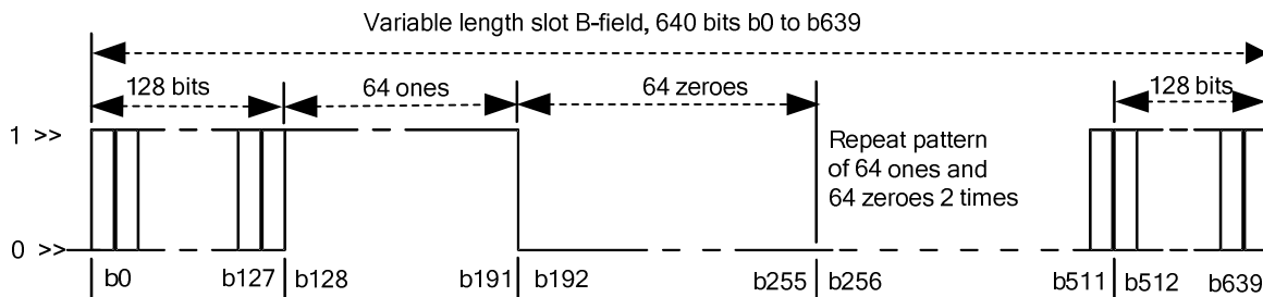
Figure 36: Test packet transmission for case 2, full-slot
