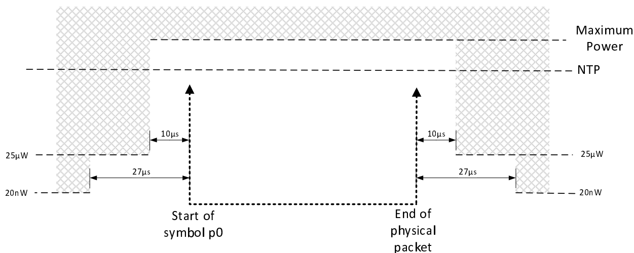
Figure 1b: Non-constant envelope modulated physical packet power-time template
