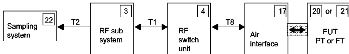
Figure 18: Test setup 1
