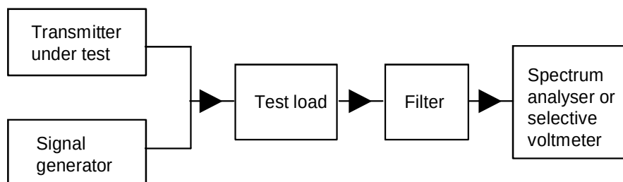
Figure E.1: Test set up
