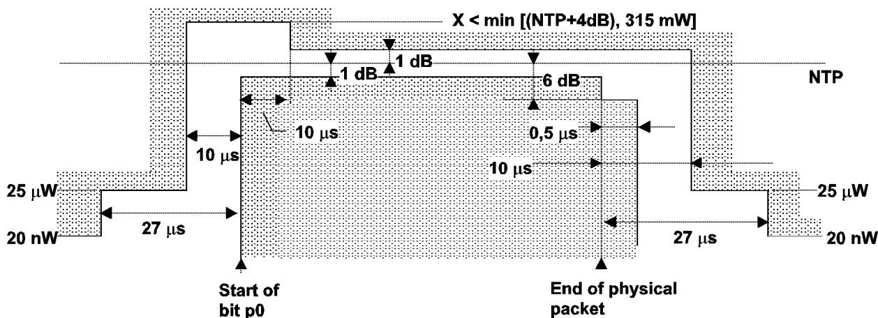
Figure 33a: Power-time template for GFSK modulated packet
