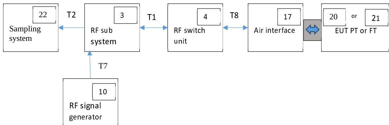
Figure 19: Test setup 2
