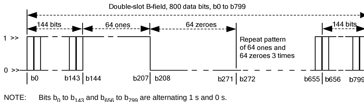
Figure 38: Test packet transmission for case 2, double-slot
