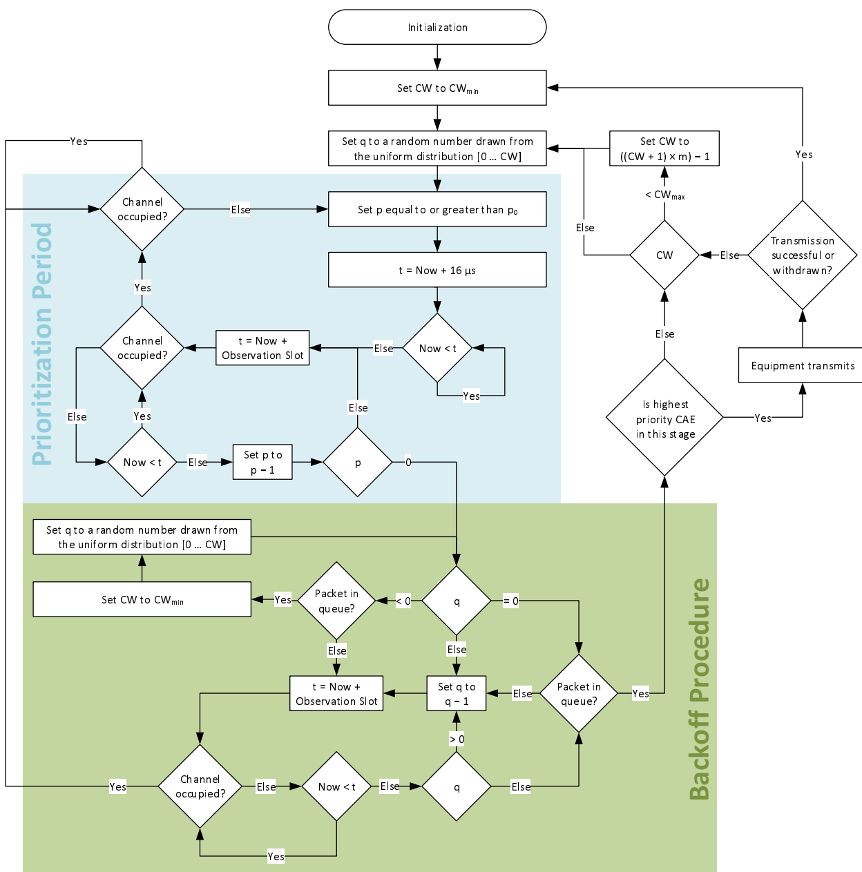
Figure G.1: Flowchart for adaptivity of LBE (initiating device)
