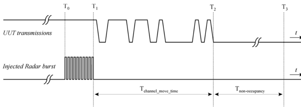
Figure 16: Channel closing transmission time, channel move time and non-occupancy period
