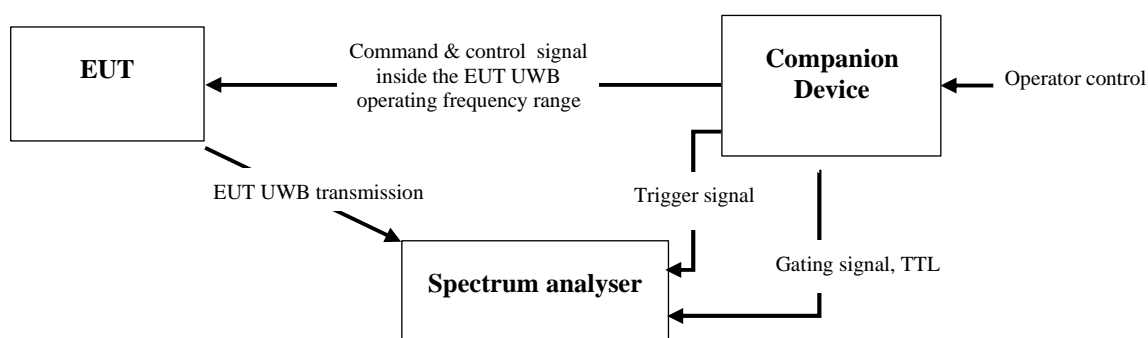
Figure 4: Gating signal setup for indoor indicator signal inside EUT operating frequency range
