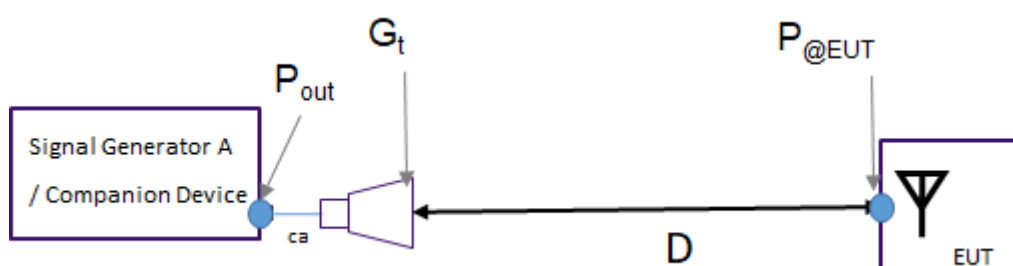
Figure 7: Setup for RBS measurement
