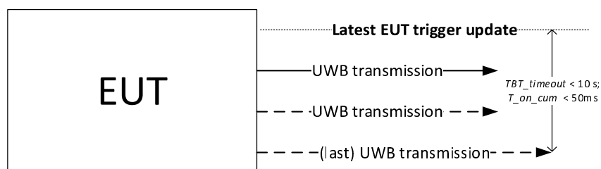
Figure 4: Trigger-before-transmit limits
