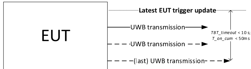
Figure 4: Trigger-before-transmit limits
