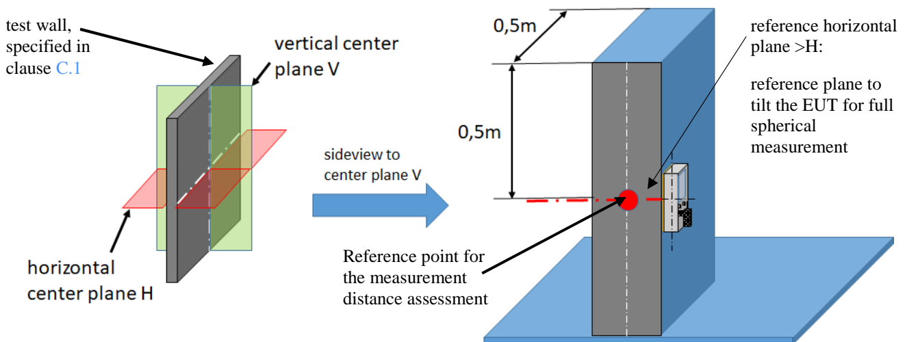
Figure 5: Reference point and horizontal plane for transmitter requirement measurements for EUT covered by EUT categories BMA2, BMA3, BMA4 and BMA5
