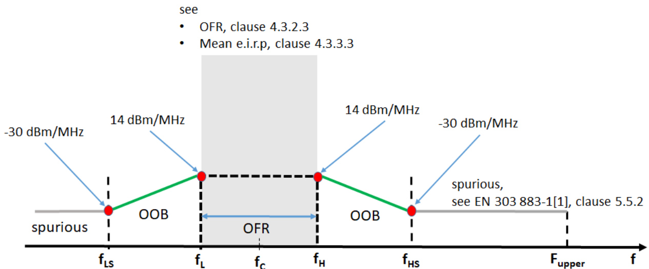
Figure 1: Overview limits for OOB and spurious domain for EUT category BMA1
