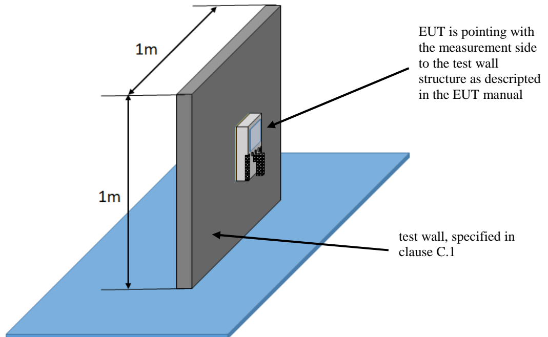
Figure 4: Test set-up for EUT covered by EUT categories BMA2, BMA3, BMA4 and BMA5
