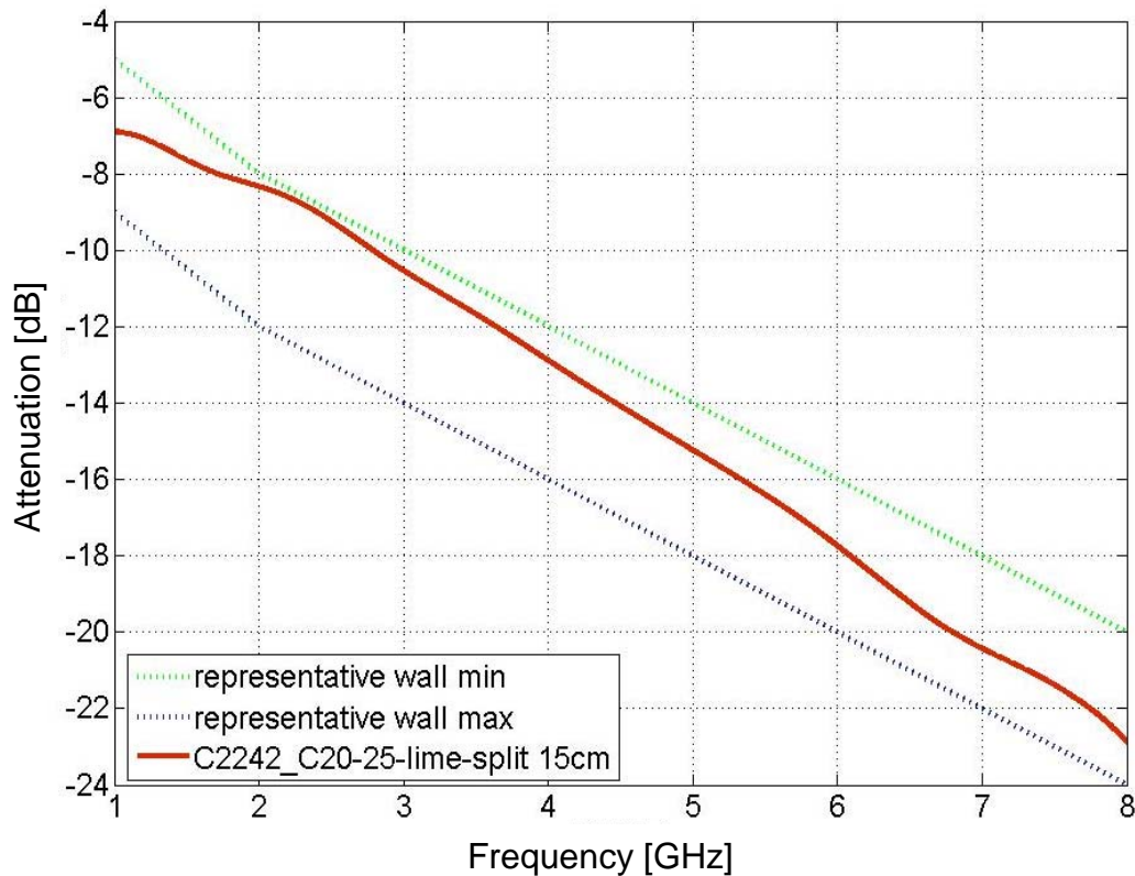
Figure E.4: Typical result for a typical absorbing material, here as example: concrete as specified in EN 206 [i.11] with a thickness d_{TXW} of 15 cm
