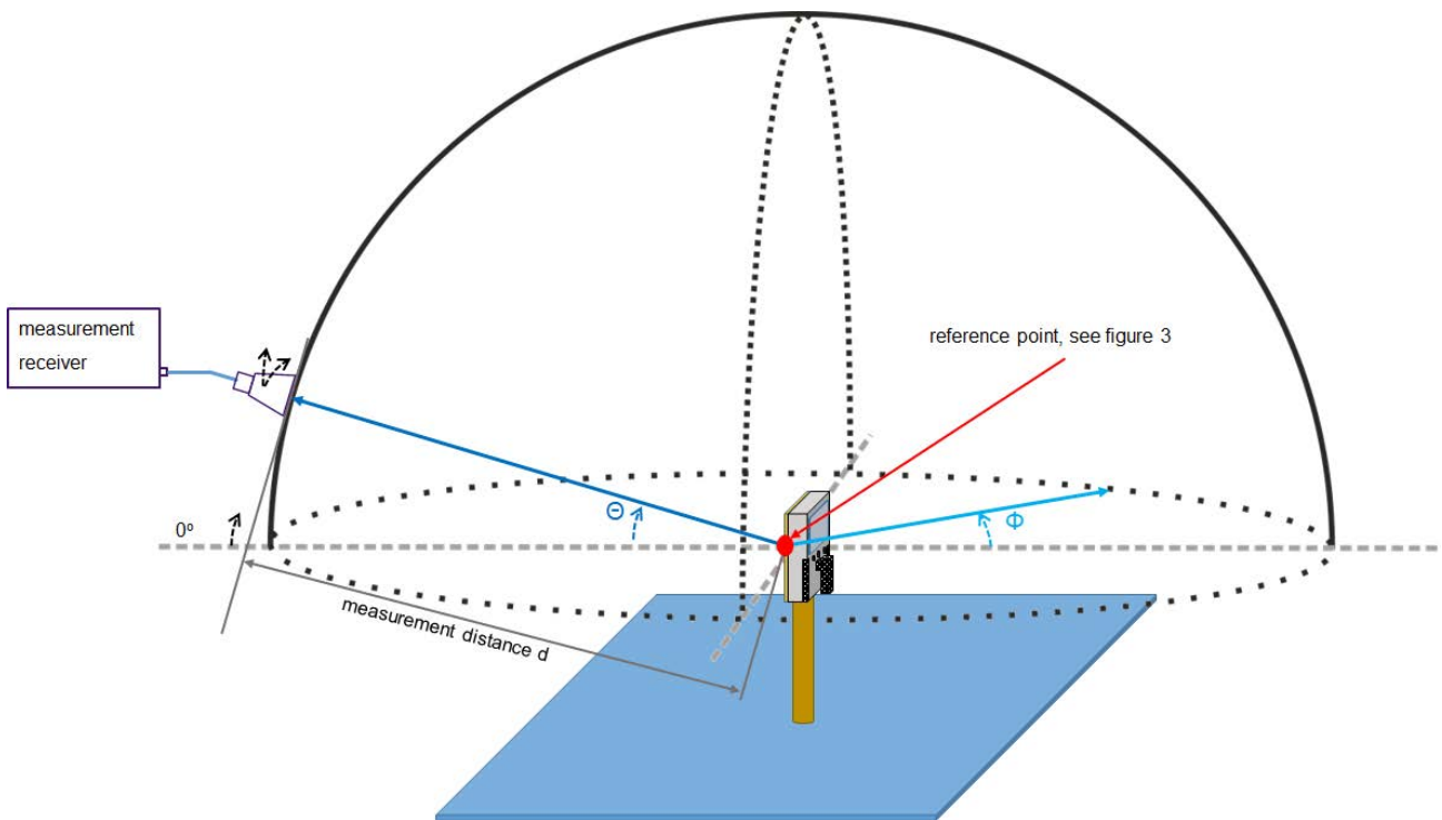
Figure 7: Mean e.i.r.p. conformance test assessment
