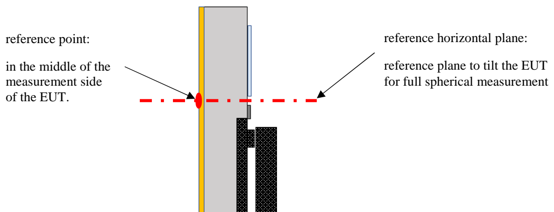
Figure 3: Reference point and horizontal plane for transmitter requirement measurements for EUT covered by EUT category BMA1
