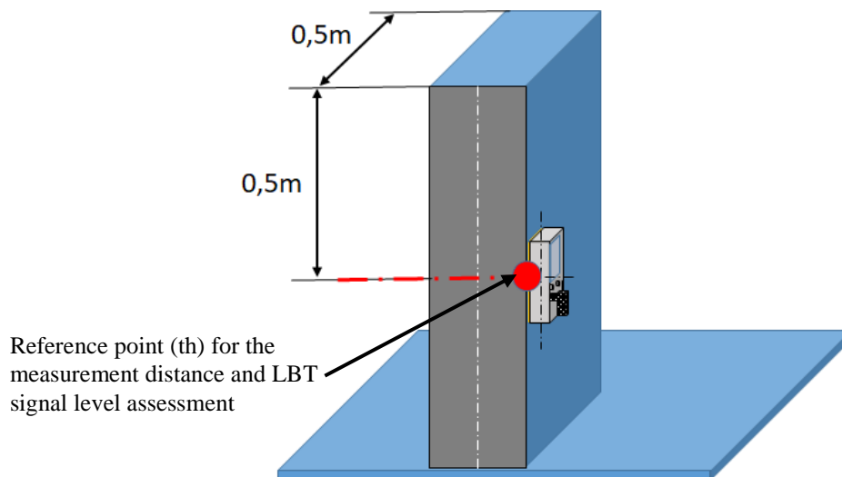
Figure 10: Reference point (th) for the LBT measurement and for the assessment of the LBT test signal level (th)
