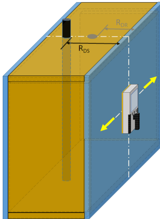
Figure 12: RBS conformance set-up for EUT designed to detect the location of objects within a building structure
