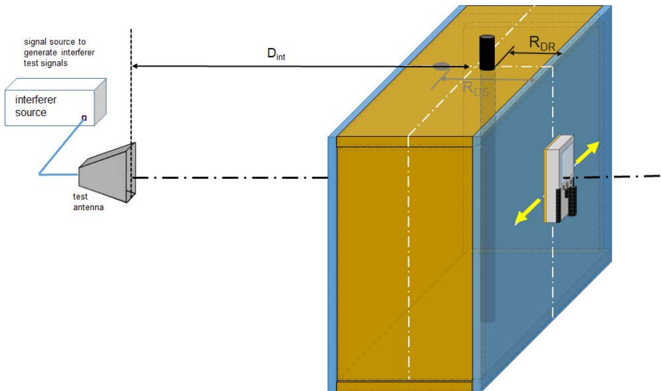
Figure 13: RBR conformance set-up for EUT designed to detect the location of objects within a building structure
