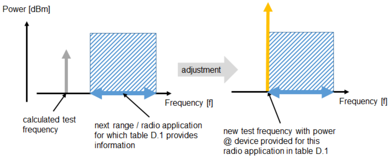
Figure D.3: Interferer test signal adjustment for the case "next interferer higher than the calculated frequency"
