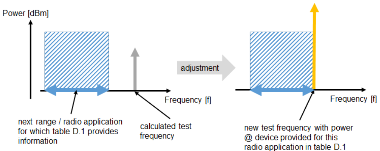
Figure D.4: Interferer test signal adjustment for the case "next interferer lower than the calculated frequency"
