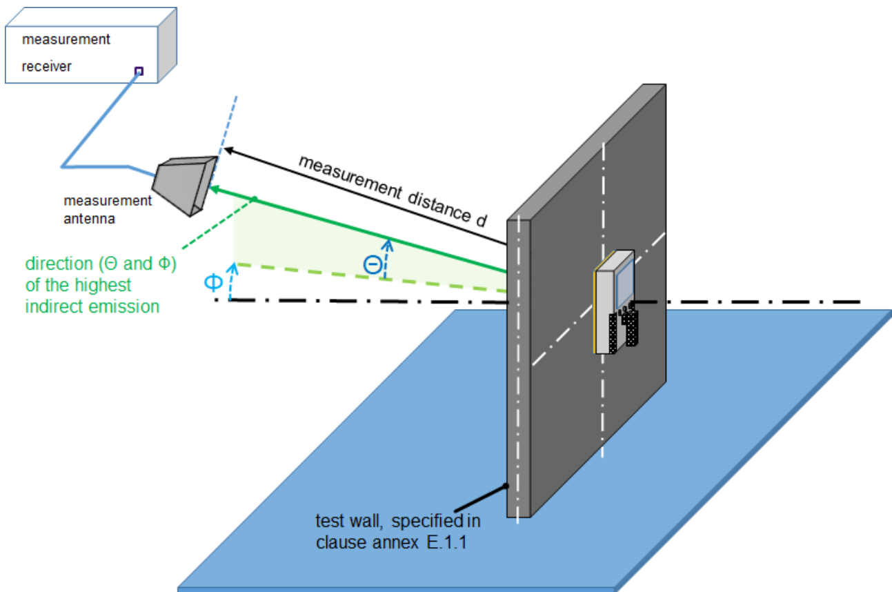
Figure 6: OFR conformance test assessment
