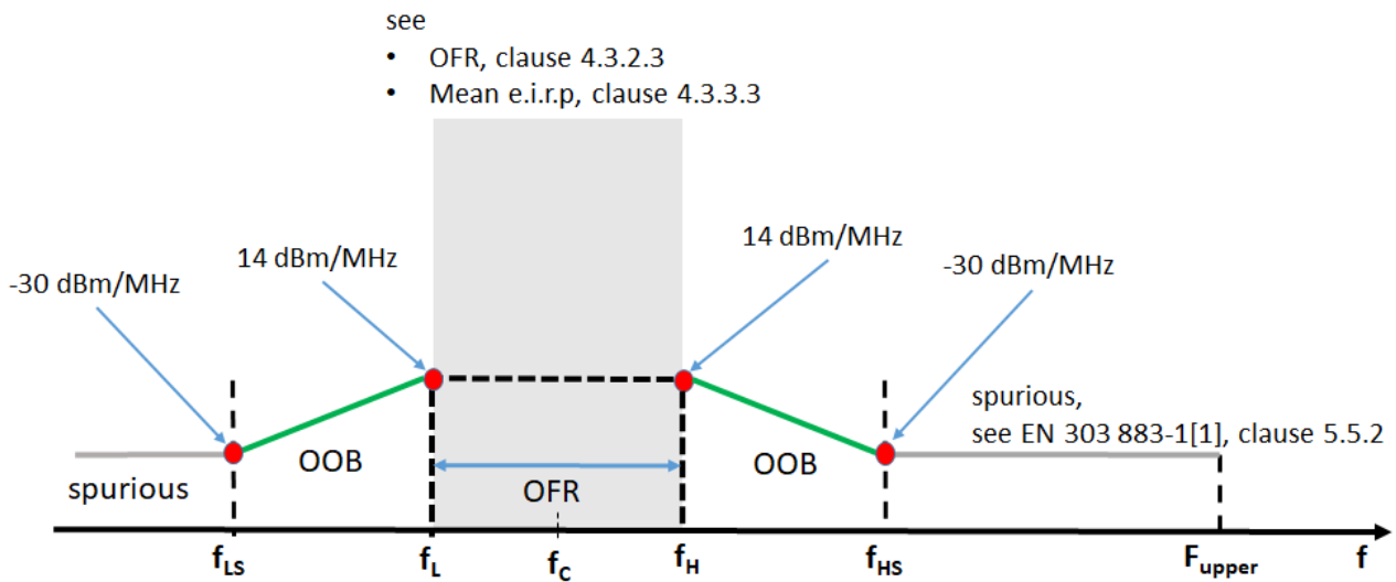
Figure 1: Overview limits for OOB and spurious domain for EUT category BMA1
