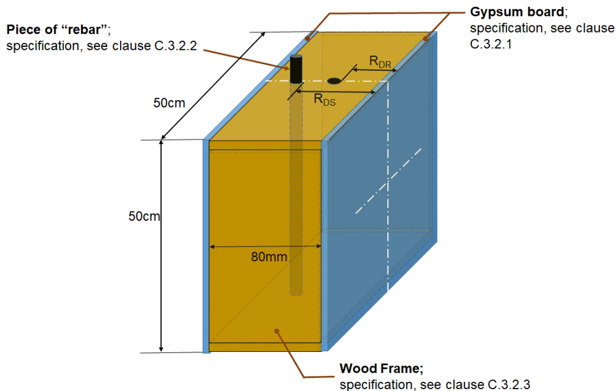
Figure C.1: Test-wall for RX-assessment
