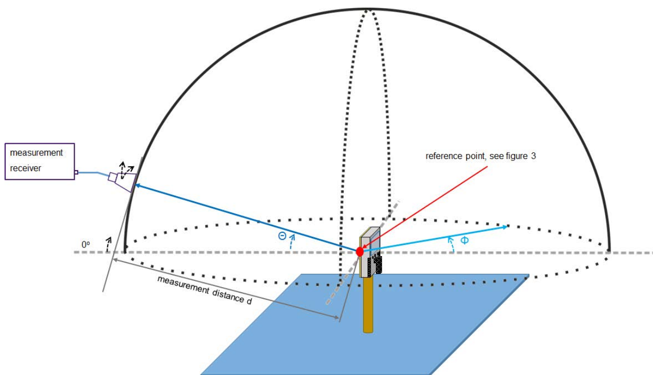
Figure 7: Mean e.i.r.p. conformance test assessment
