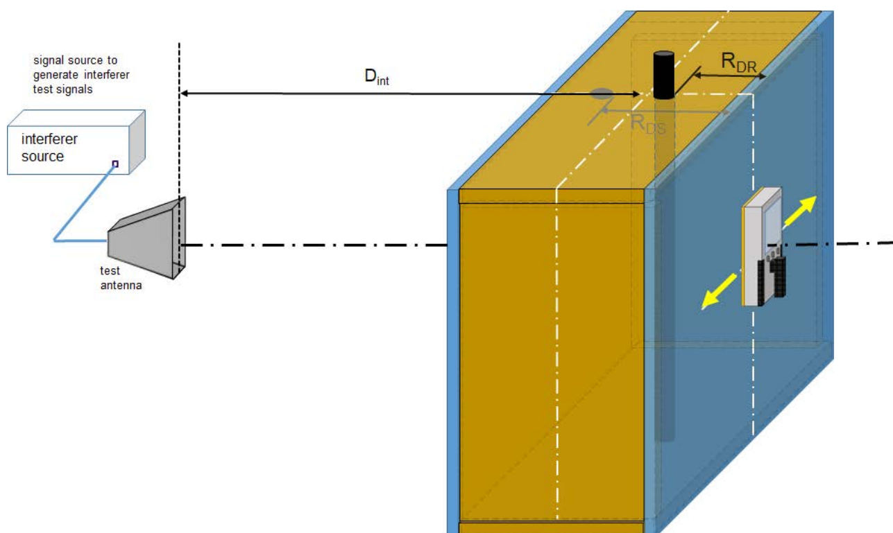
Figure 13: RBR conformance set-up for EUT designed to detect the location of objects within a building structure
