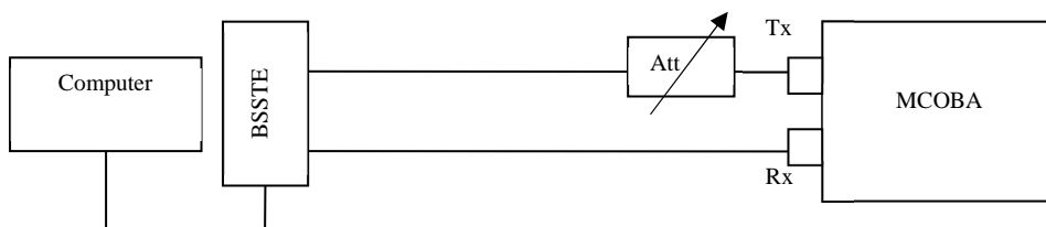
Figure 5.2.6.1.2-1: Test setup
