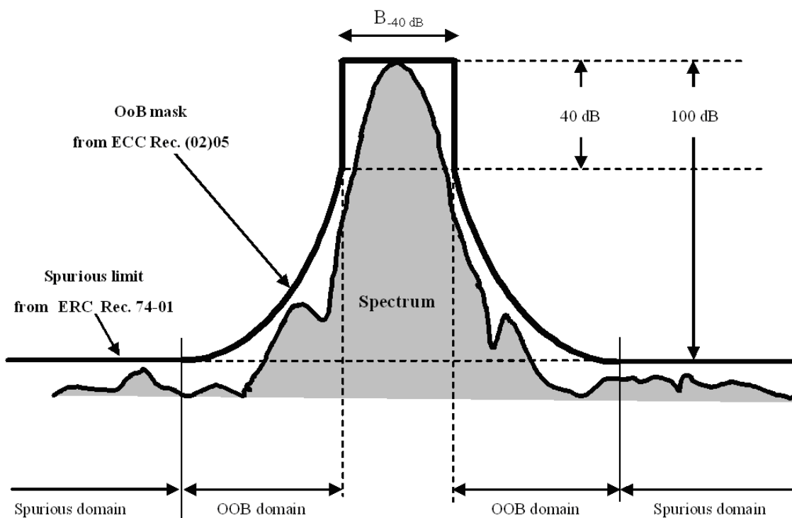
Figure 3: Definition of OoB and spurious emission domains (Not to scale)
