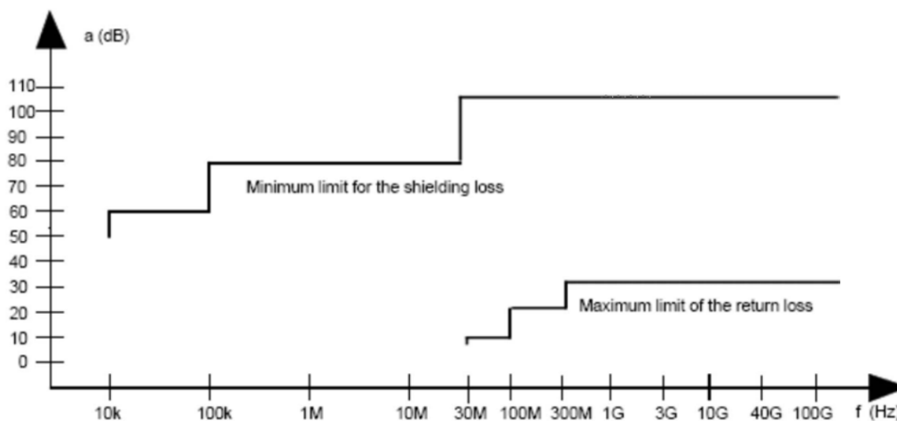
Figure C.2: Specification for shielding and reflections
