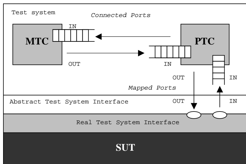
Figure 10: Illustration of the connect and map operations
