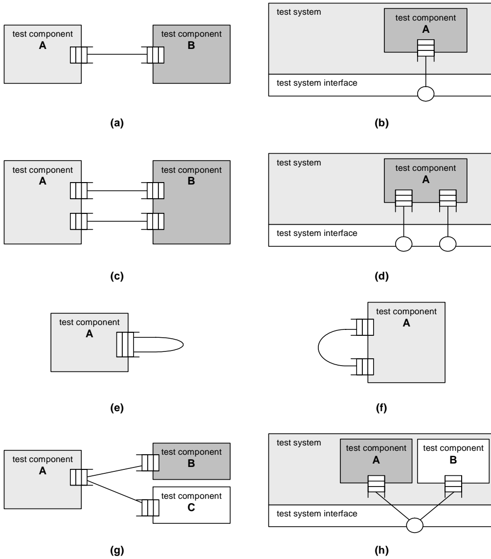
Figure 6: Allowed connections
