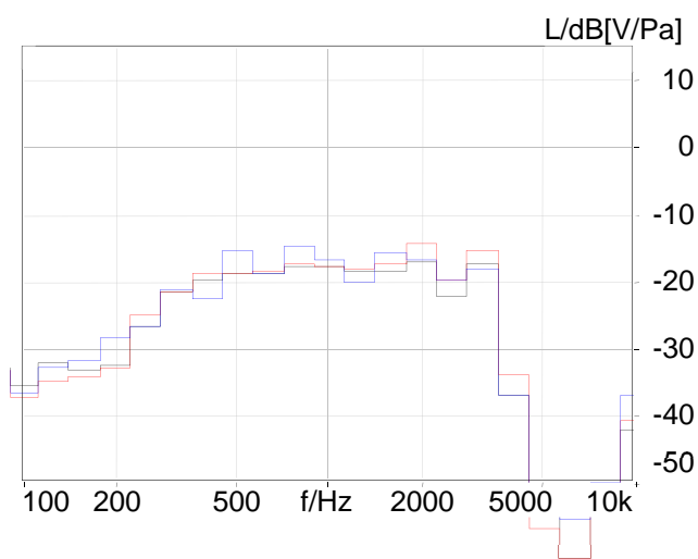
Figure B.8: Measurements of phone 8: black - fully anechoic; red - office type room; blue - semi anechoic
