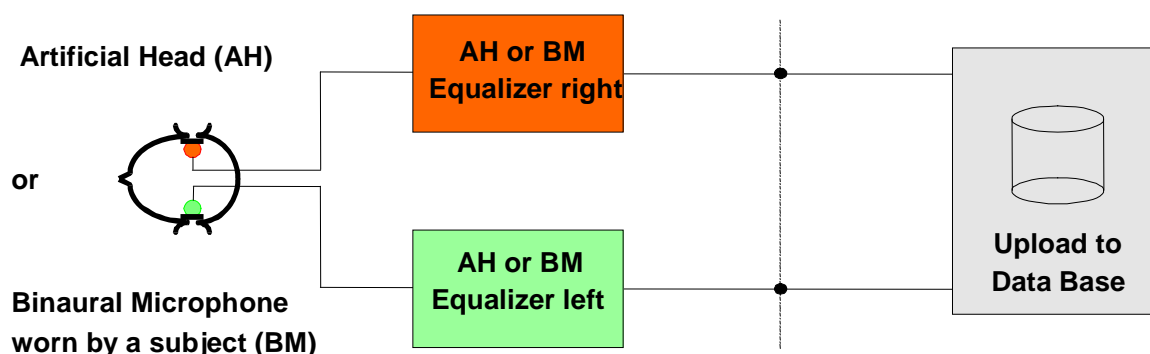
Figure 1: Recording setup
