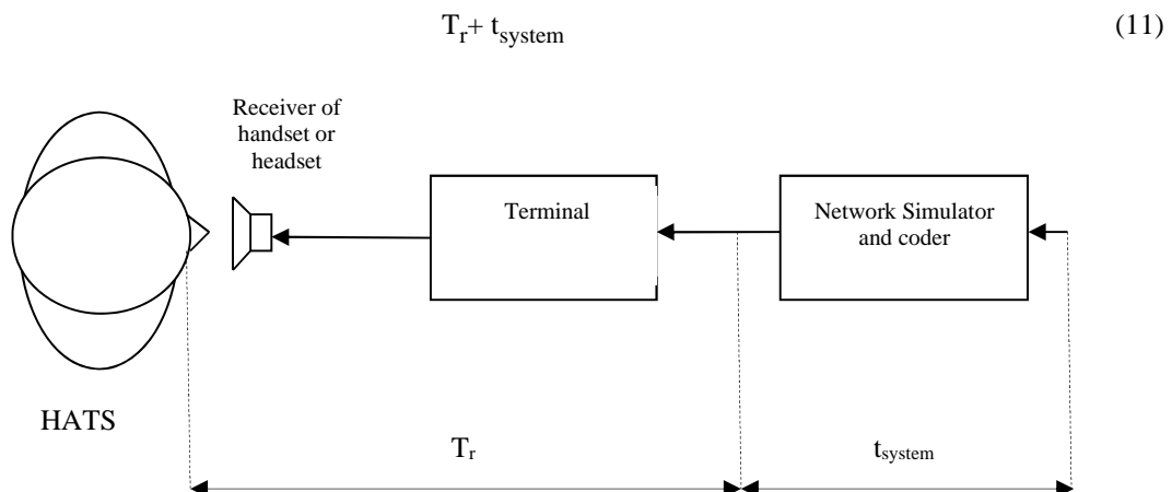
Figure 12: Different blocks contributing to the delay in receive direction
