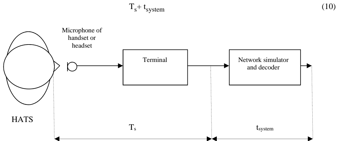
Figure 11: Different blocks contributing to the delay in send direction
