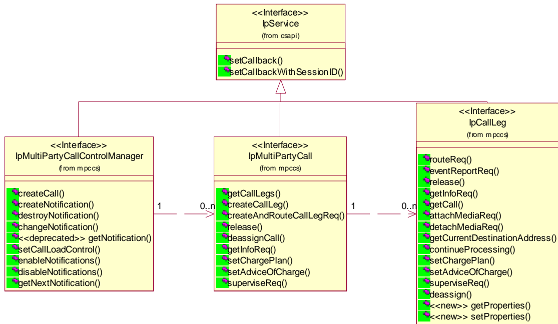
Figure 2: Service Interfaces
