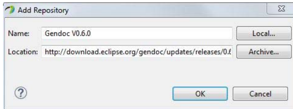
Figure 5.4-2: Installing Gendoc (2)
