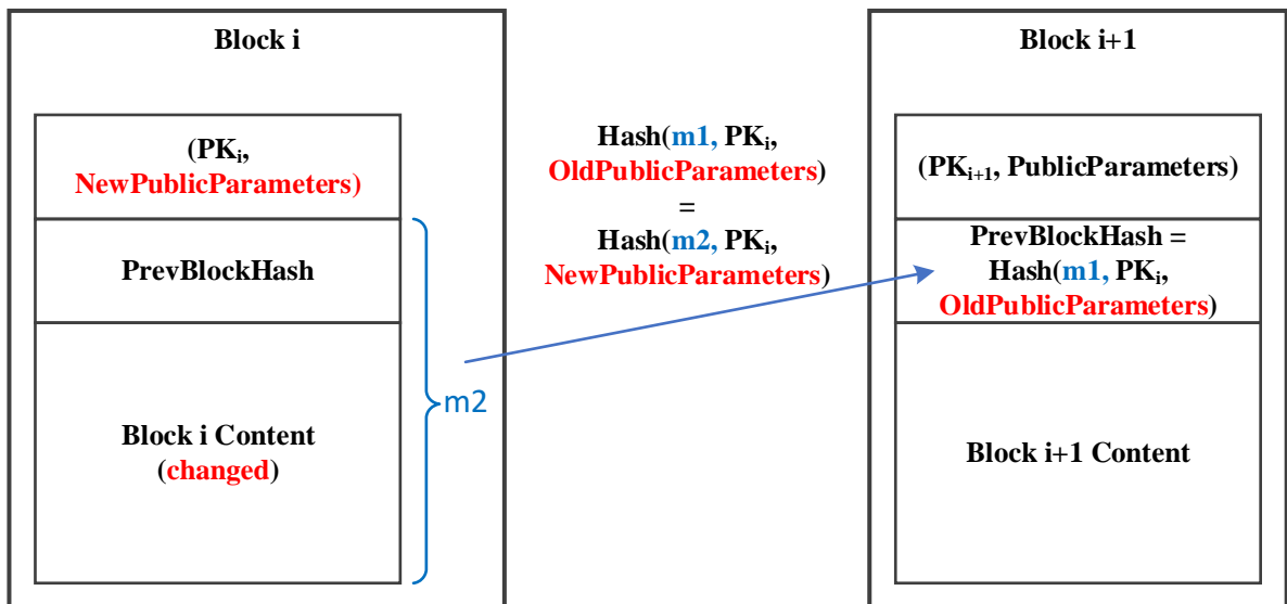
Figure 6.2.2-2: Blockchain after a Redaction Operation (i.e. change the content of Block i from m1 to m2)
