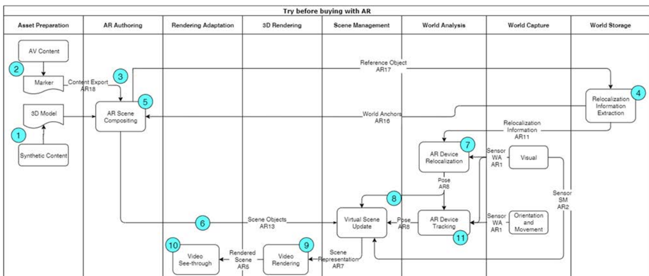
Figure 4: Workflow diagram of the subfunctions implemented for the use case "Try before buying with AR"
