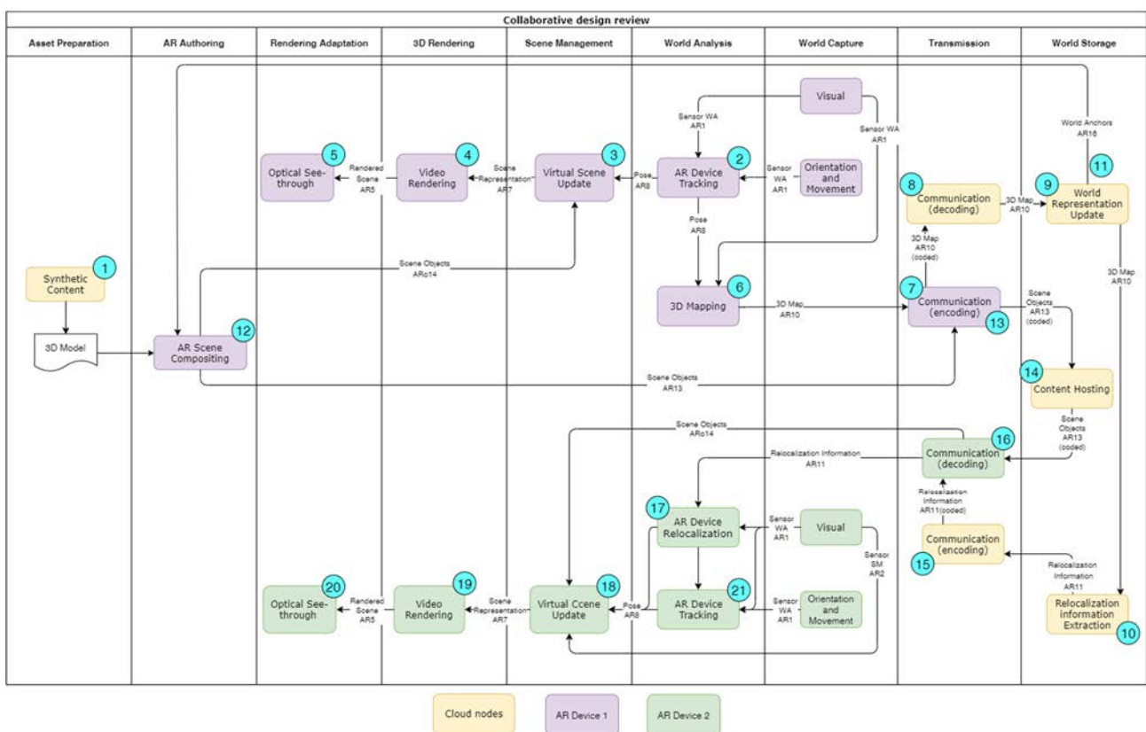
Figure 10: Workflow diagram of the subfunctions implemented for the use case "Collaborative design review"
