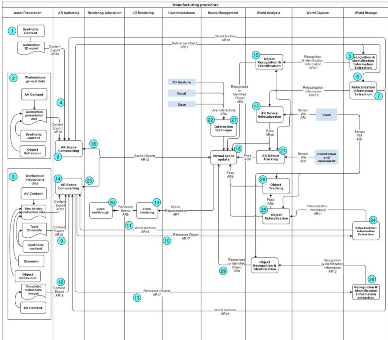
Figure 9: Workflow diagram of the subfunctions implemented for the use case "Manufacturing procedure"
