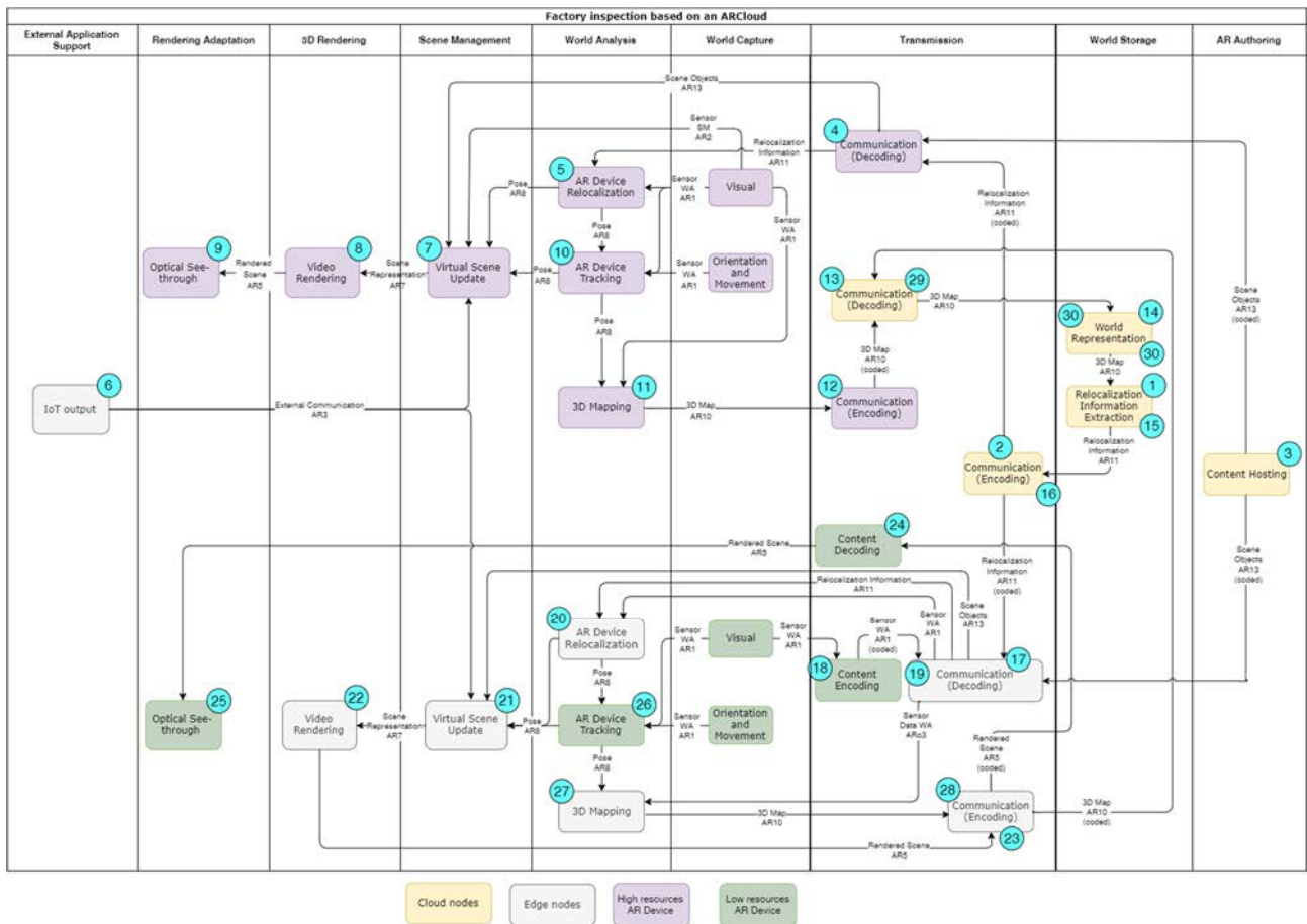
Figure 11: Workflow diagram of the subfunctions implemented for the use case "Factory inspection based on an ARCloud"
