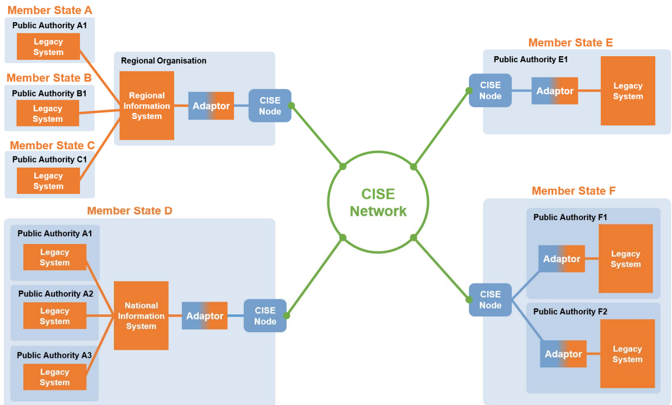
Figure 3: CISE top level architecture
