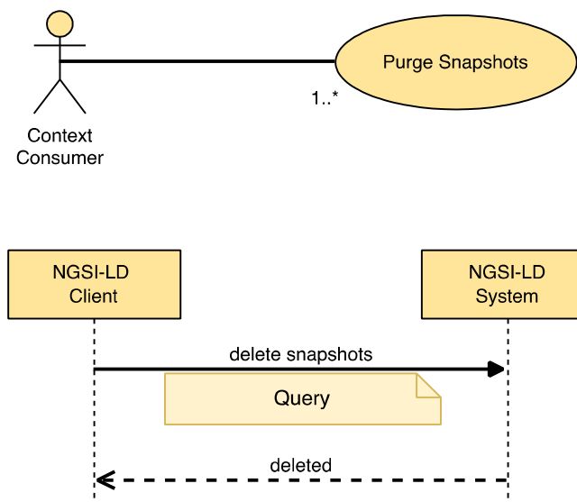
Figure 5.16.7.2-1: Purge Snapshots use case
