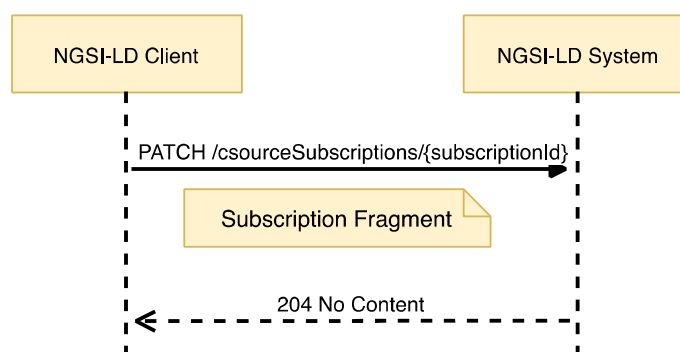
Figure 6.13.3.2-1: Update Context Source Registration Subscription interaction
