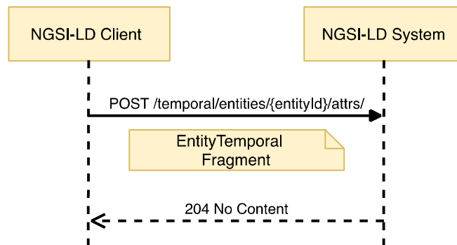
Figure 6.20.3.1-1: Add Attributes to Temporal Evolution of an Entity interaction
