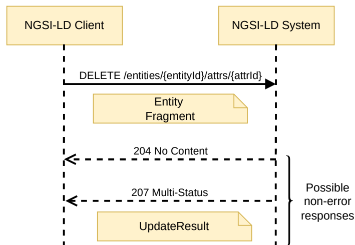
Figure 6.7.3.2-1: Delete Attribute interaction
