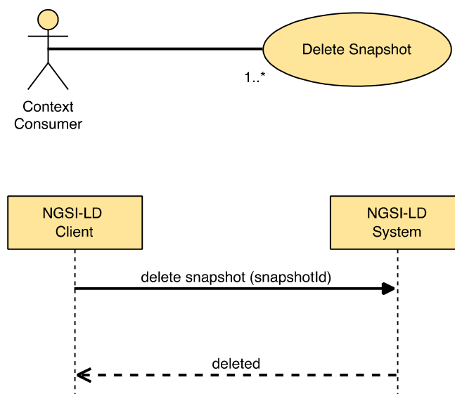
Figure 5.16.5.2-1: Delete Snapshot use case
