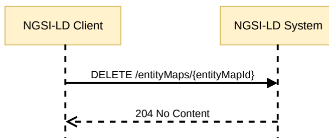
Figure 6.32.3.3-1: Delete and Reload @context interaction
