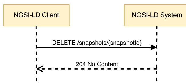
Figure 6.37.3.3-1: Delete Snapshot interaction
