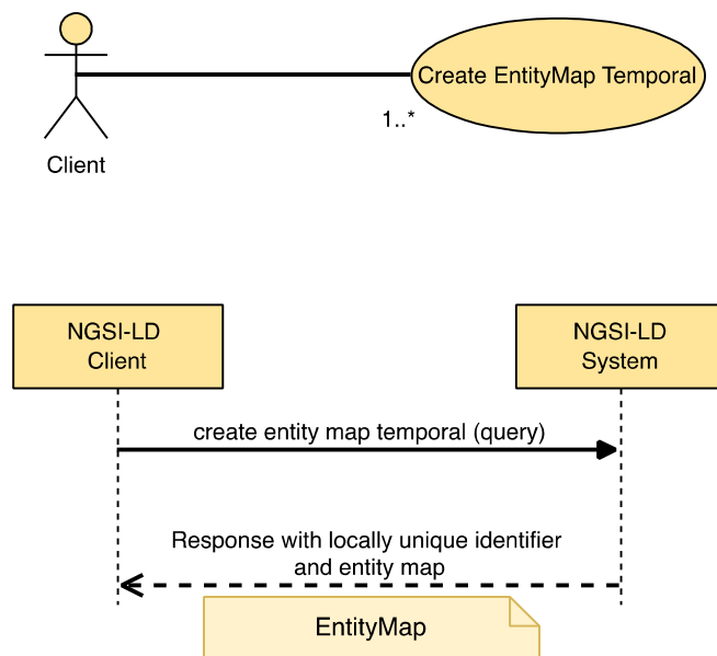
Figure 5.14.5.2-1: Query Temporal Evolution for creating EntityMap use case
