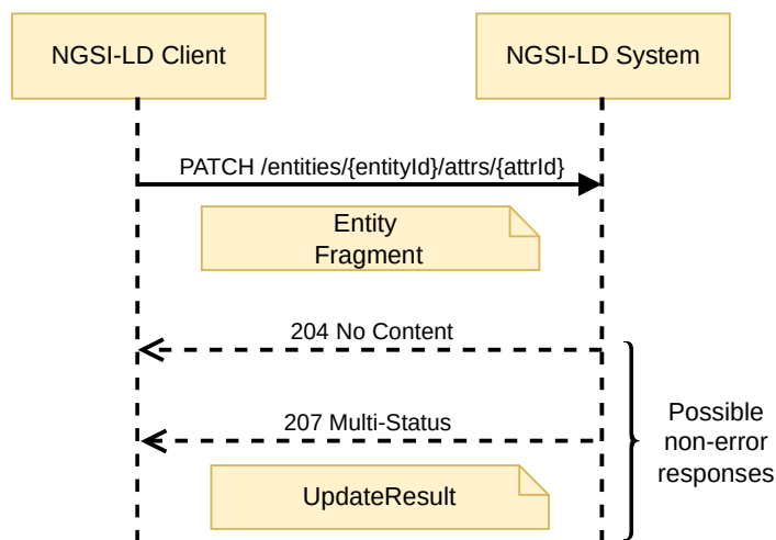
Figure 6.7.3.1-1: Partial Attribute Update interaction
