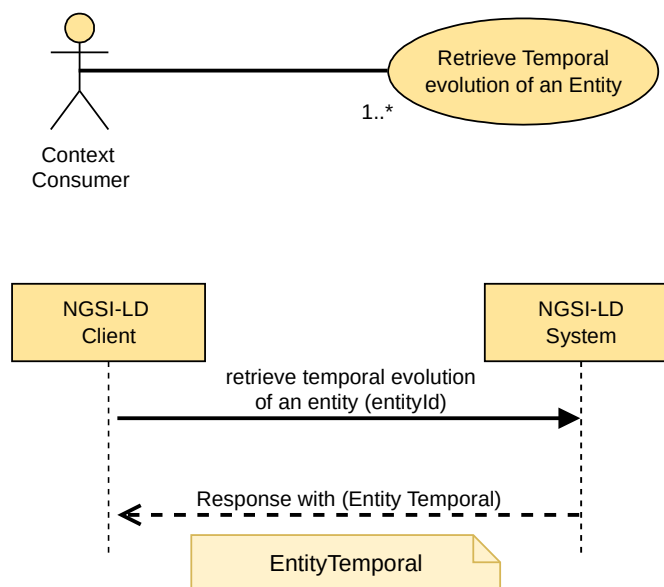
Figure 5.7.3.2-1: Retrieve Temporal Evolution of an Entity use case
