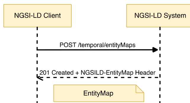
Figure 6.35.3.2-1: Create EntityMap for Query Temporal Evolution of Entities via POST interaction
