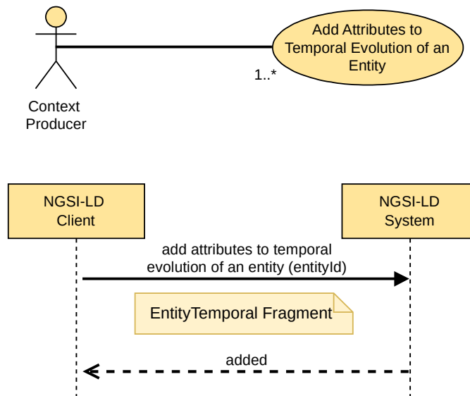
Figure 5.6.12.2-1: Add Attributes to Temporal Evolution of an Entity use case
