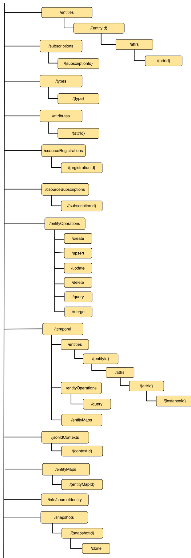
Figure 6.2-1: Resource URI structure of the NGSI-LD API
