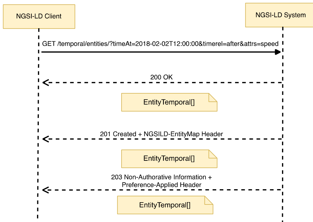
Figure 6.18.3.2-1: Query Temporal Evolution of Entities interaction
