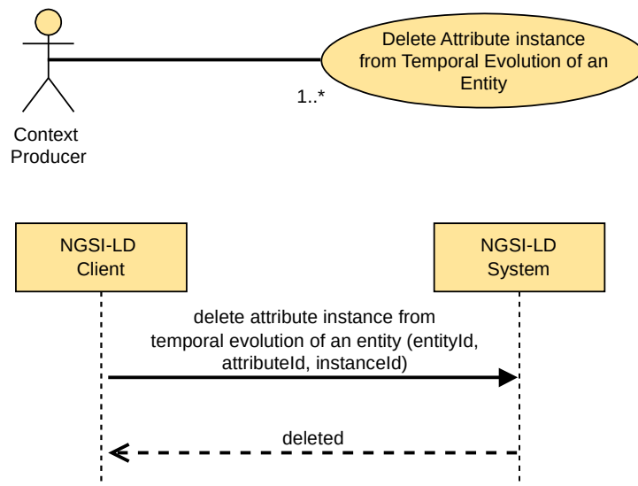
Figure 5.6.15.2-1: Delete Attribute Instance from Temporal Evolution of an Entity use case
