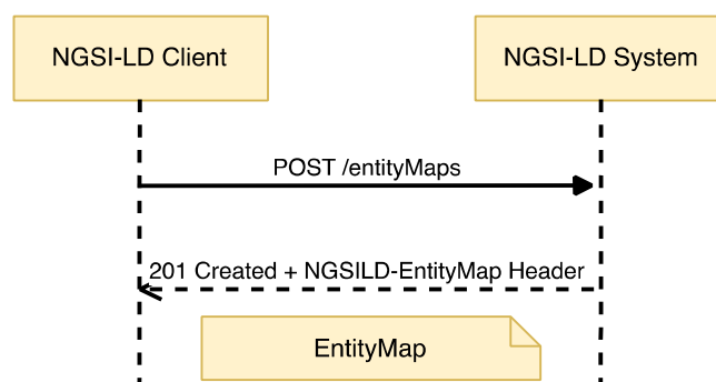
Figure 6.34.3.2-1: Create EntityMap for Query Entities via POST interaction
