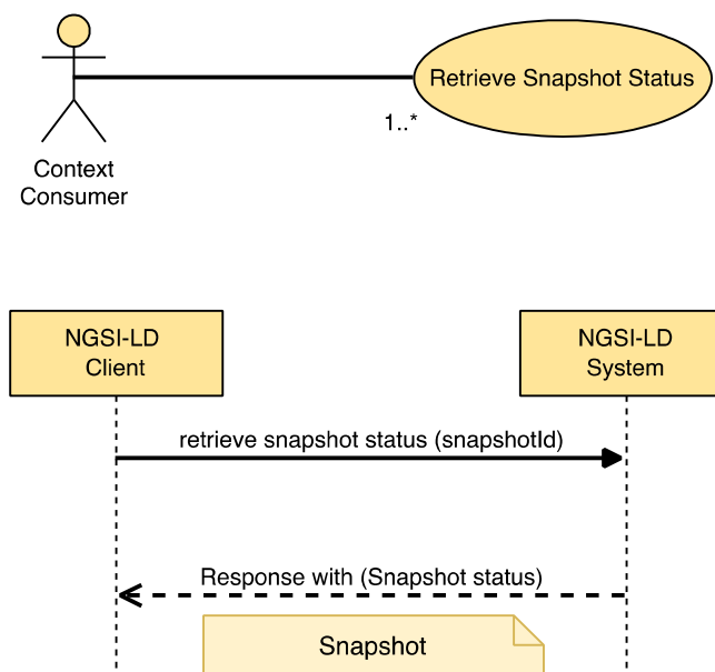
Figure 5.16.3.2-1: Retrieve Snapshot Status use case
