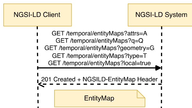
Figure 6.35.3.1-1: Create EntityMap for Query Temporal Evolution of Entities interaction
