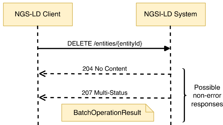
Figure 6.5.3.2-1: Delete Entity interaction
