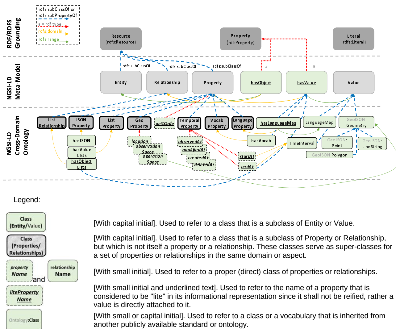
Figure 4.2.3-1: NGSi-LD Core Meta-Model plus the Cross-Domain Ontology
