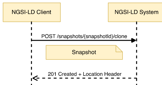
Figure 6.38.3.1-1: Clone Snapshot interaction
