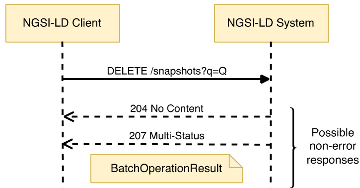
Figure 6.36.3.2-1: Purge Snapshots interaction
