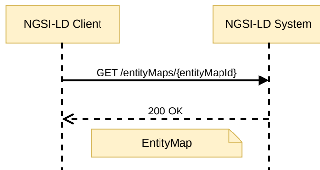
Figure 6.32.3.1-1: Retrieve EntityMap
