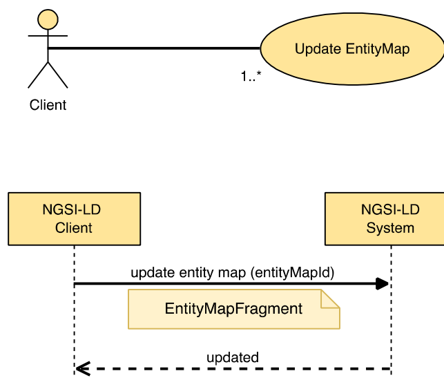
Figure 5.14.2.2-1: Update EntityMap
