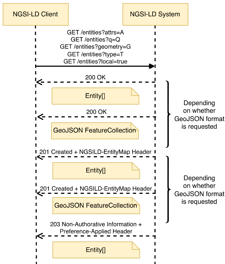
Figure 6.4.3.2-1: Query Entities interaction
