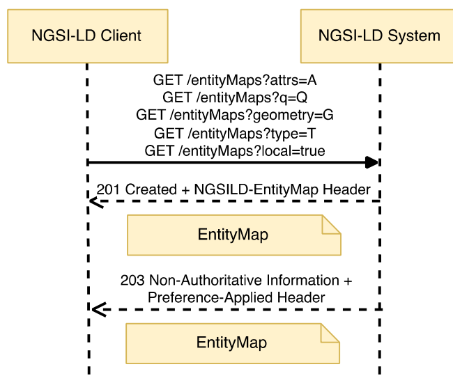
Figure 6.34.3.1-1: Create EntityMap for Query Entities interaction
