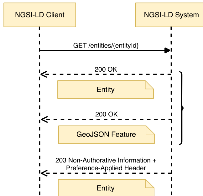
Figure 6.5.3.1-1: Retrieve Entity interaction
