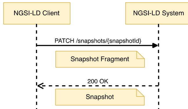
Figure 6.37.3.2-1: Update Snapshot Status interaction
