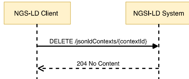
Figure 6.30.3.2-1: Delete and Reload @context interaction
