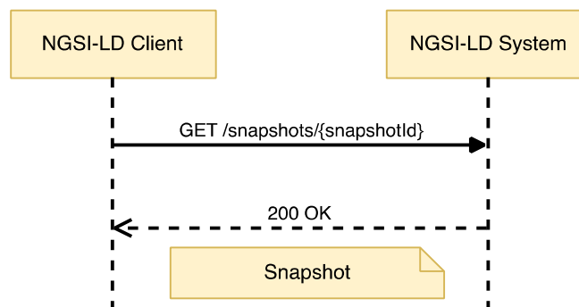
Figure 6.37.3.1-1: Retrieve Snapshot Status interaction
