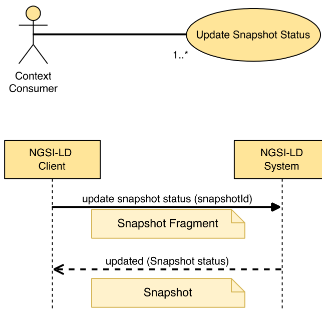
Figure 5.16.4.2-1: Update Snapshot Status use case
