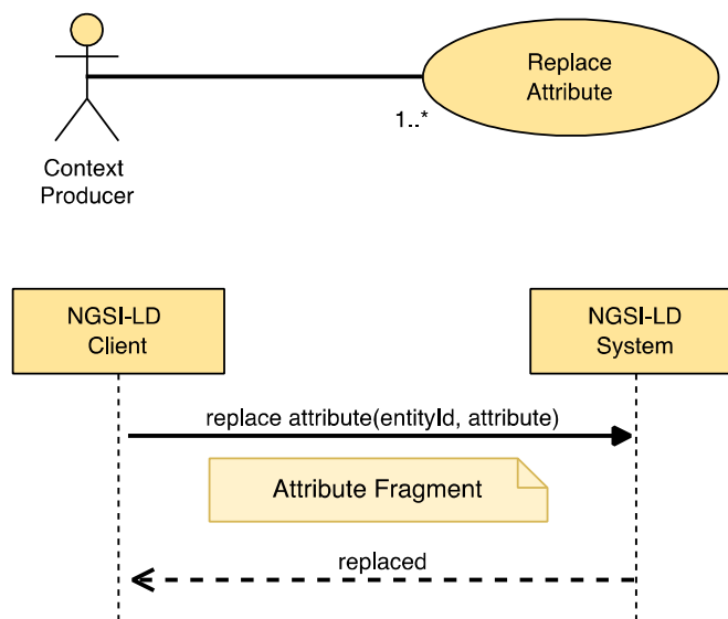
Figure 5.6.19.2-1: Replace Attribute use case
