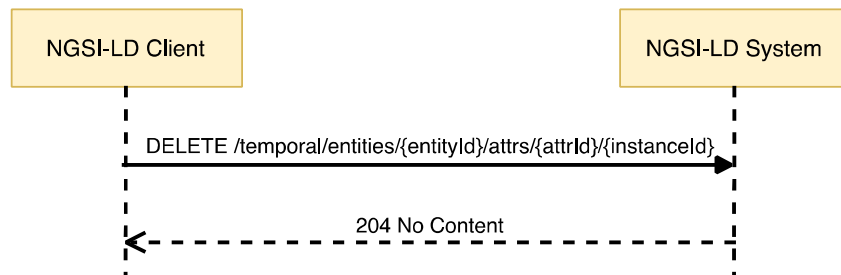
Figure 6.22.3.2-1: Delete Attribute instance from Temporal Evolution of an Entity interaction
