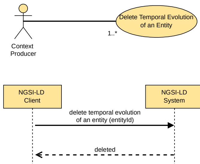
Figure 5.6.16.2-1: Delete Temporal Evolution of an Entity use case
