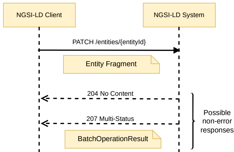
Figure 6.5.3.4-1: Merge Entity interaction
