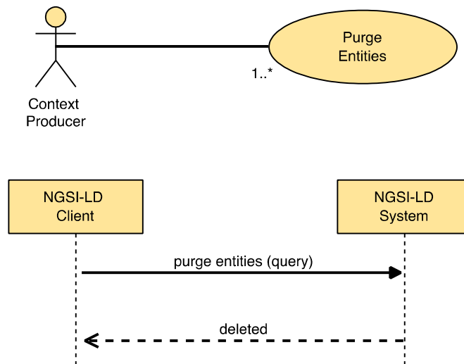
Figure 5.6.21.2-1: Purge Entities use case
