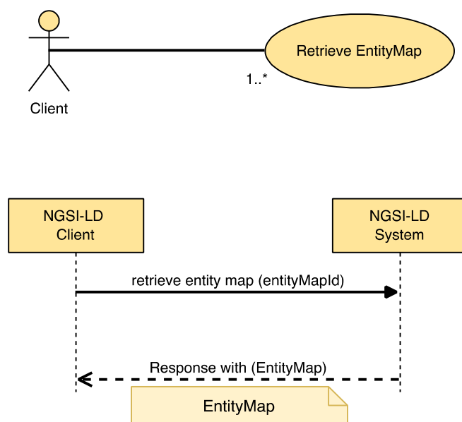
Figure 5.14.1.2-1: Retrieve EntityMap
