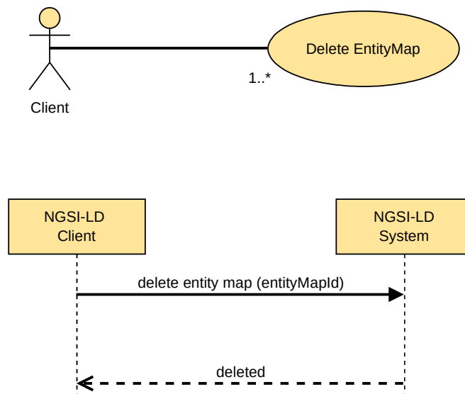
Figure 5.14.3.2-1: Delete EntityMap
