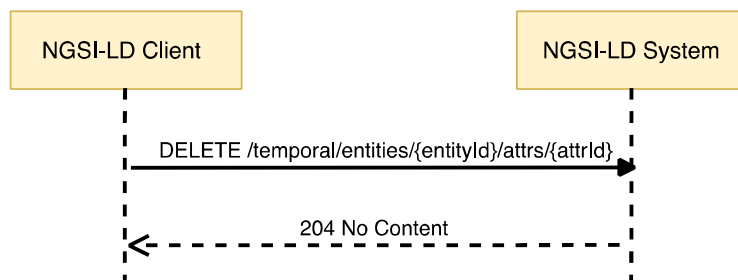
Figure 6.21.3.1-1: Delete Attribute from Temporal Evolution of an Entity interaction
