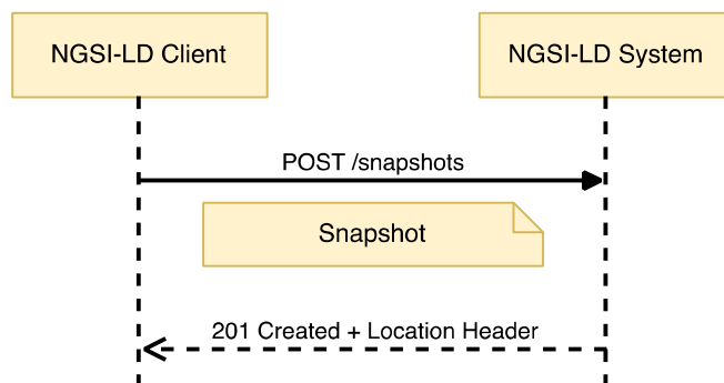
Figure 6.36.3.1-1: Create Snapshot interaction
