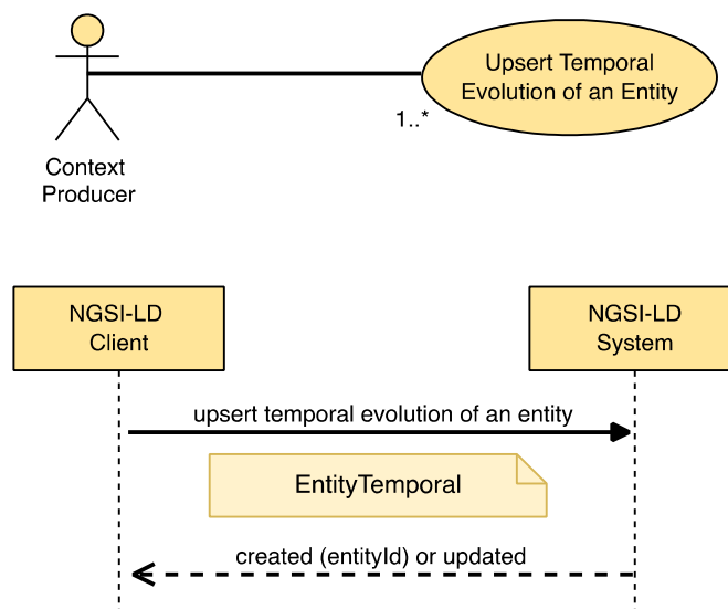
Figure 5.6.11.2-1: Create or Update (Upsert) Temporal Evolution of an Entity use case
