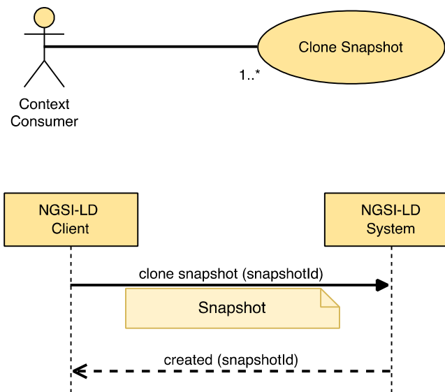
Figure 5.16.2.2-1: Clone Snapshot use case
