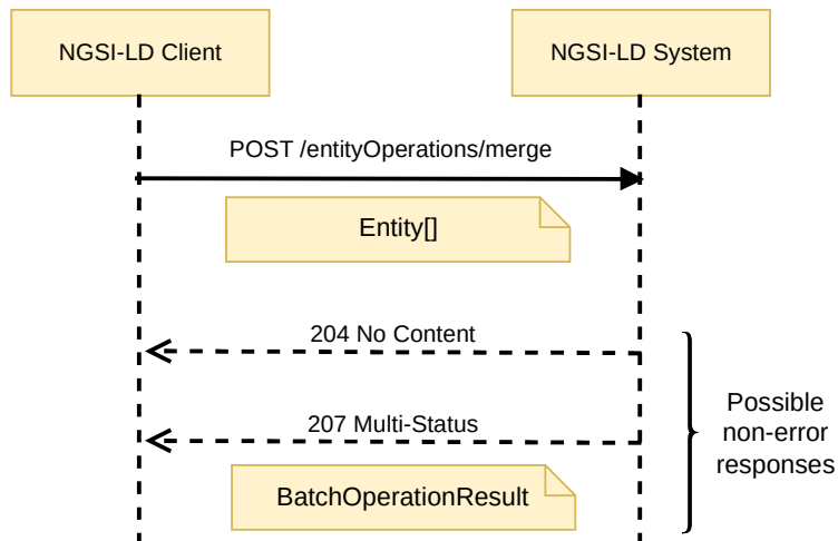
Figure 6.31.3.1-1: Batch Entity Merge interaction
