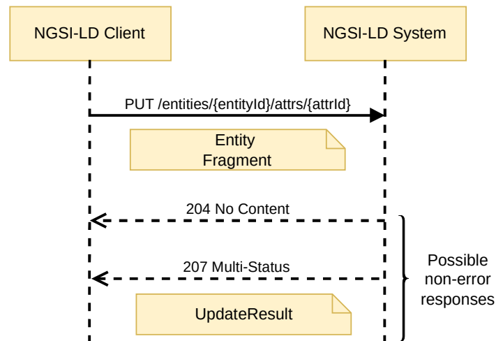
Figure 6.7.3.3-1: Replace Attribute interaction
