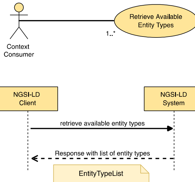
Figure 5.7.5.2-1: Retrieve Available Entity Types use case
