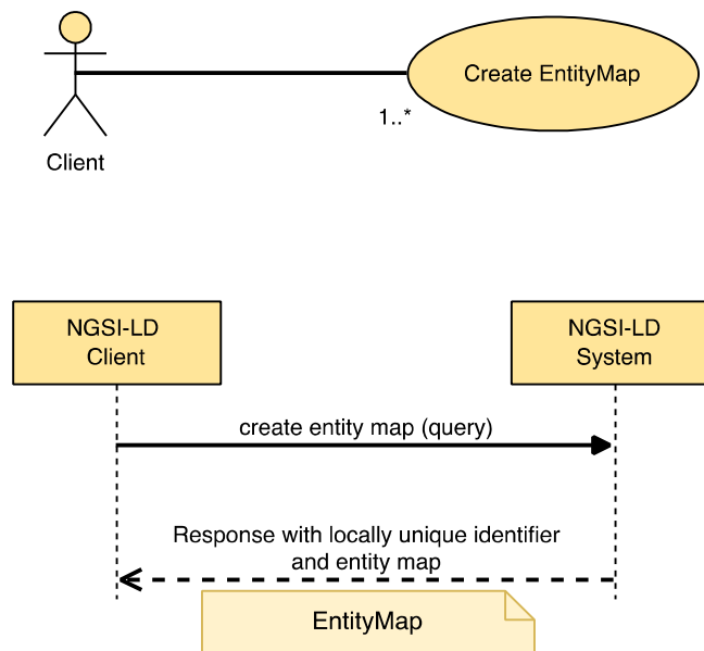
Figure 5.14.4.2-1: Query Entities for creating EntityMap use case
