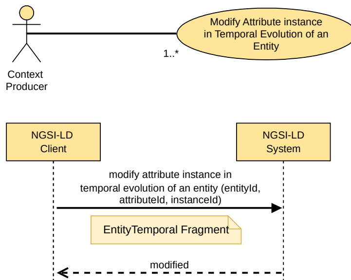
Figure 5.6.14.2-1: Modify Attribute Instance in Temporal Evolution of an Entity use case
