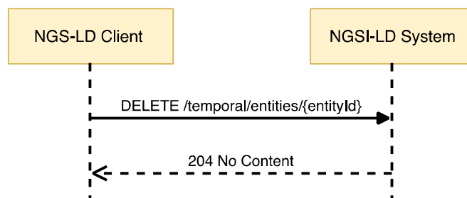
Figure 6.19.3.2-1: Delete Temporal Evolution of an Entity interaction
