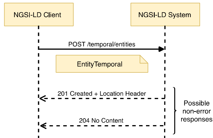
Figure 6.18.3.1-1: Create or Update Temporal Evolution of an Entity interaction
