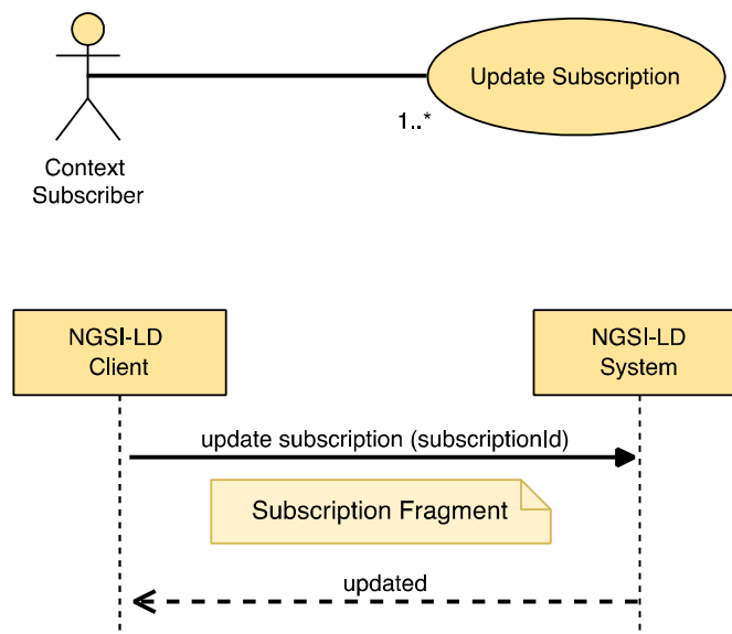
Figure 5.8.2.2-1: Update subscription use case
