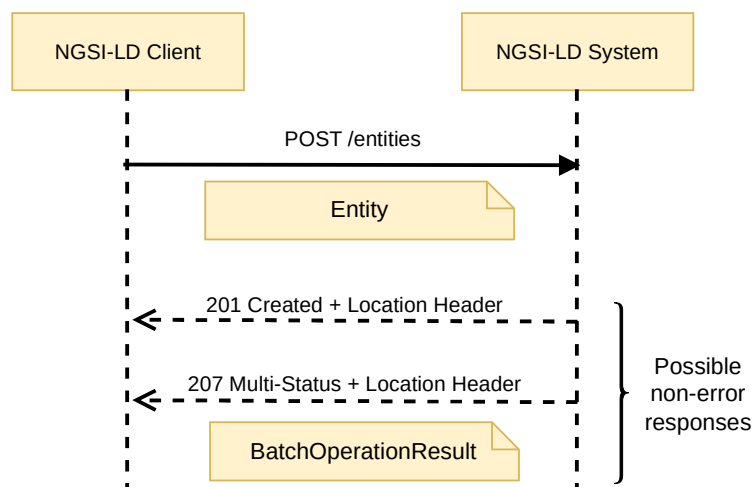
Figure 6.4.3.1-1: Create Entity interaction
