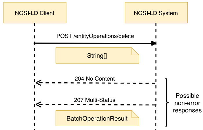
Figure 6.17.3.1-1: Batch Entity Delete interaction
