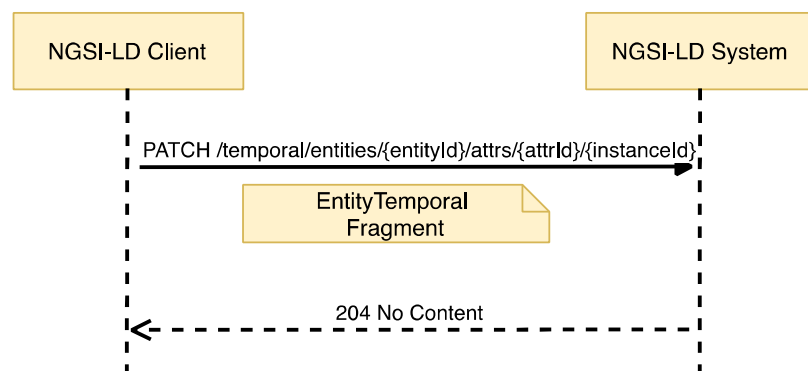
Figure 6.22.3.1-1: Modify Attribute instance from Temporal Evolution interaction
