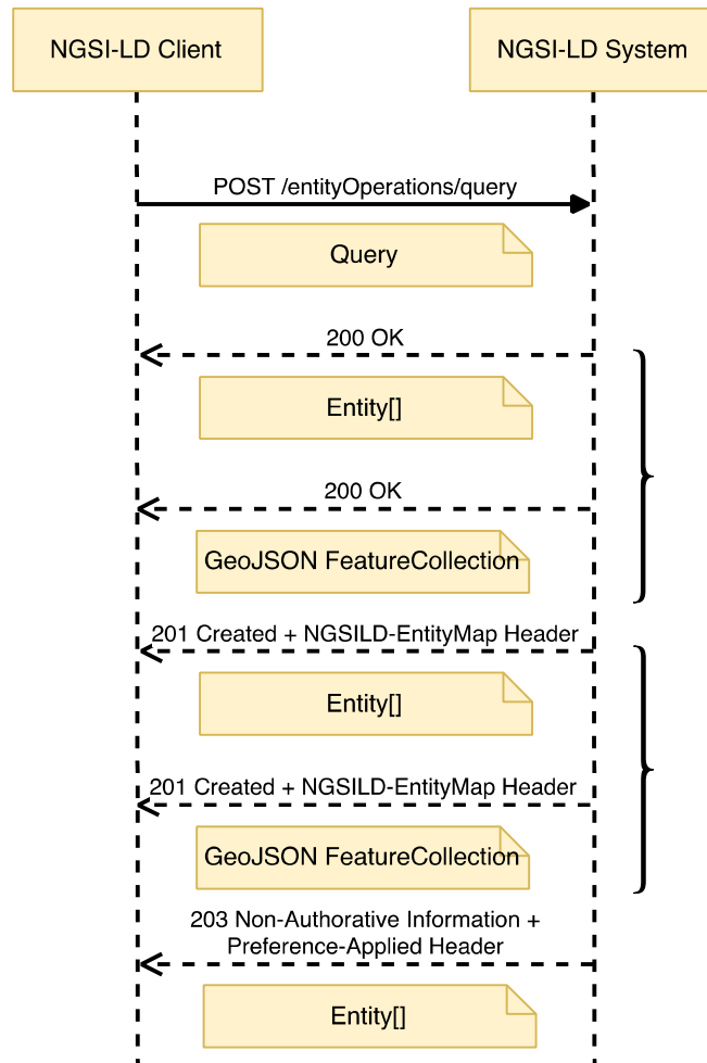
Figure 6.23.3.1-1: Query Entity via POST interaction
