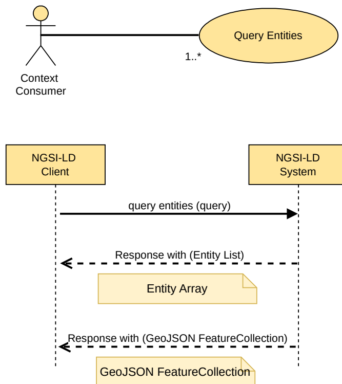
Figure 5.7.2.2-1: Query Entities use case
