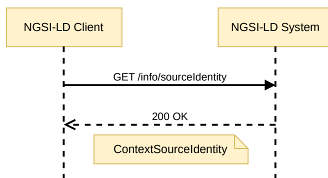
Figure 6.33.3.1-1: Retrieve Context Source Identity Information
