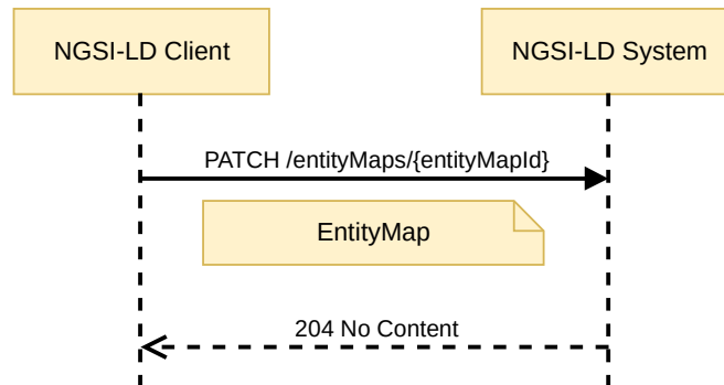
Figure 6.32.3.2-1: Update EntityMap
