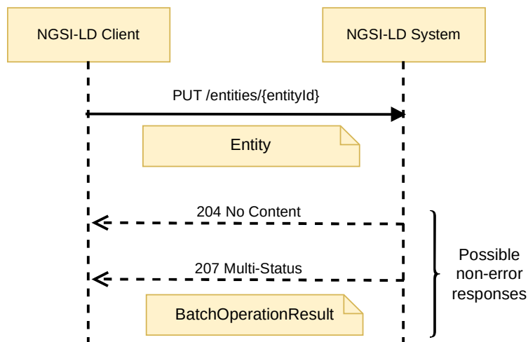
Figure 6.5.3.3-1: Replace Entity interaction
