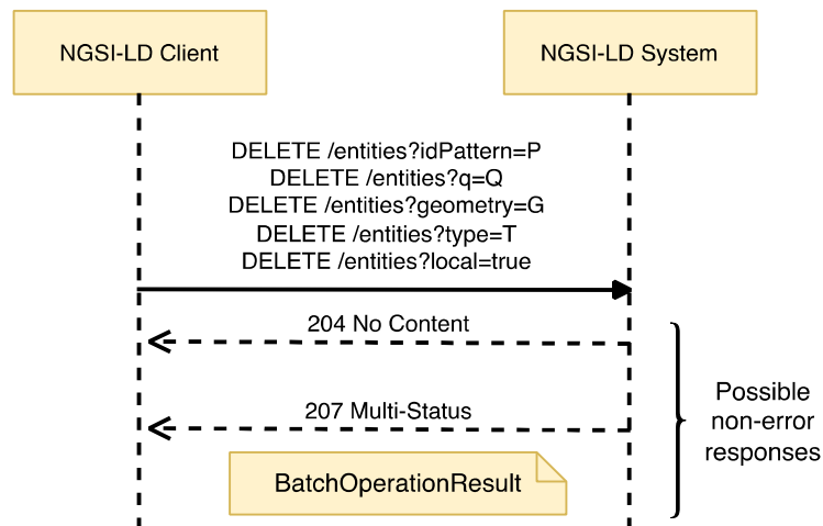
Figure 6.4.3.3-1: Purge Entities interaction
