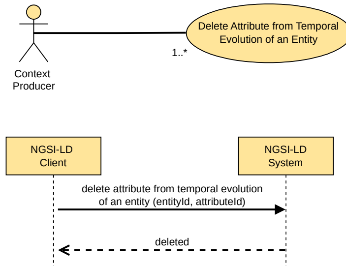
Figure 5.6.13.2-1: Delete Attribute from Temporal Evolution of an Entity use case
