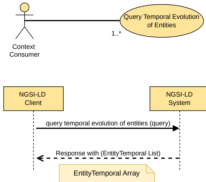
Figure 5.7.4.2-1: Query Temporal Evolution of Entities use case
