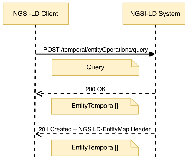
Figure 6.24.3.1-1: Temporal Query Entity via POST interaction
