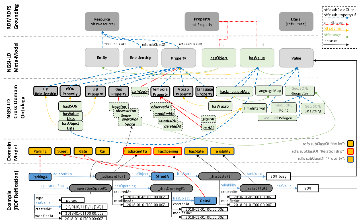
Figure 4.2.4-1: Cross-Domain Ontology and instantiation
