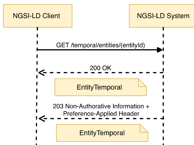
Figure 6.19.3.1-1: Retrieve Temporal Evolution of an Entity interaction
