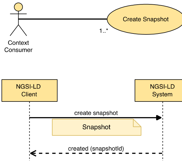
Figure 5.16.1.2-1: Create Snapshot use case
