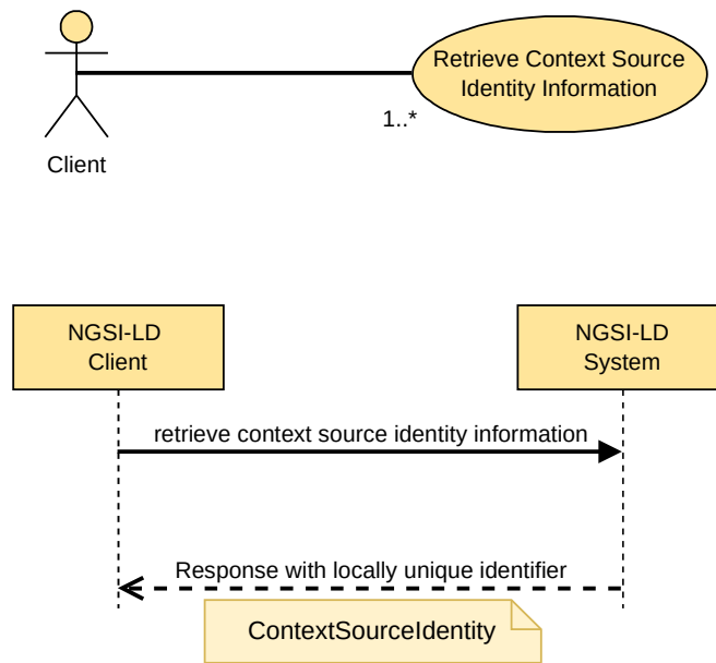
Figure 5.15.1.2-1: Retrieve Context Source Identity Information
