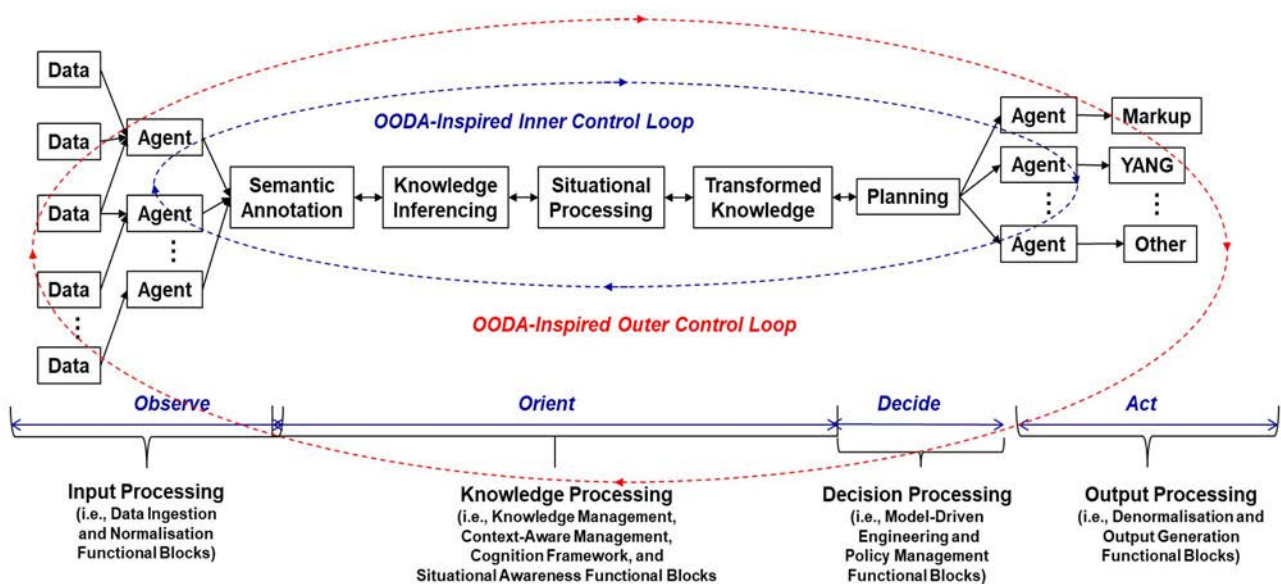
Figure 6-18: Simplified Knowledge Processing Flow
