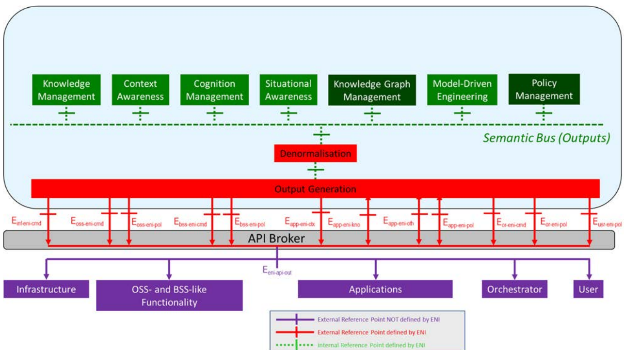
Figure 6-32: Policy Output External Reference Points
