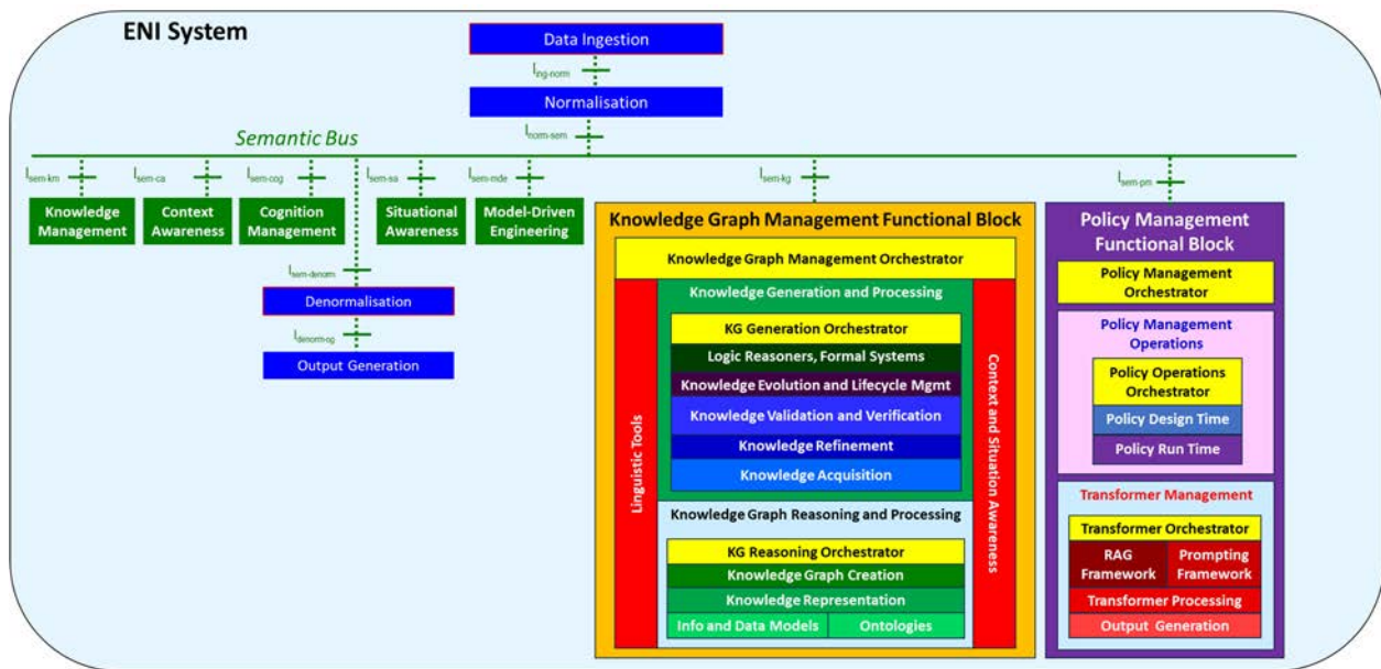
Figure 7-7: Overview of the ENI Internal Facing External Reference Points
