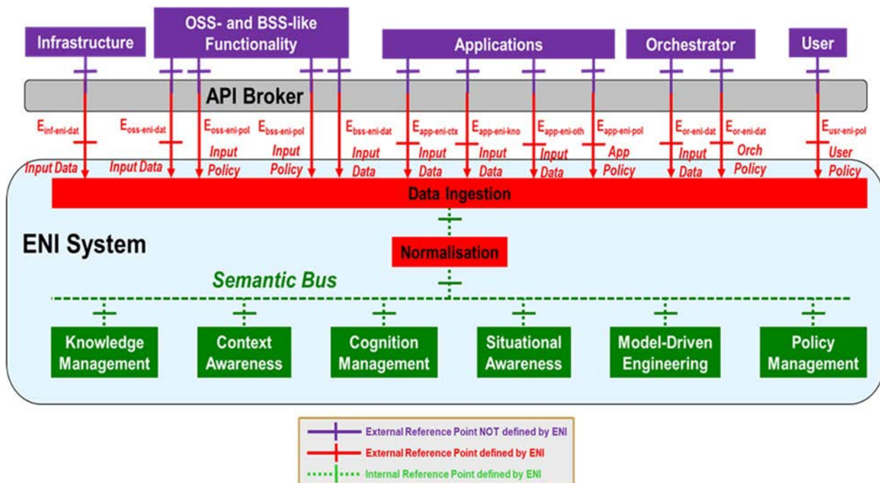
Figure 7-1: Overview of the ENI Internal Facing External Reference Points
