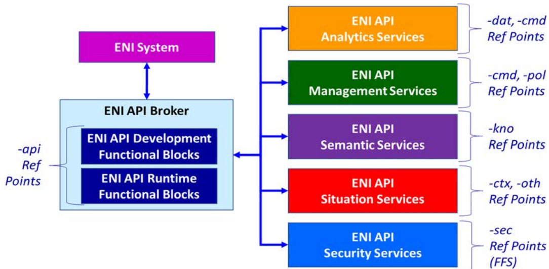
Figure 7-4: High-Level ENI API Architecture Functional Diagram
