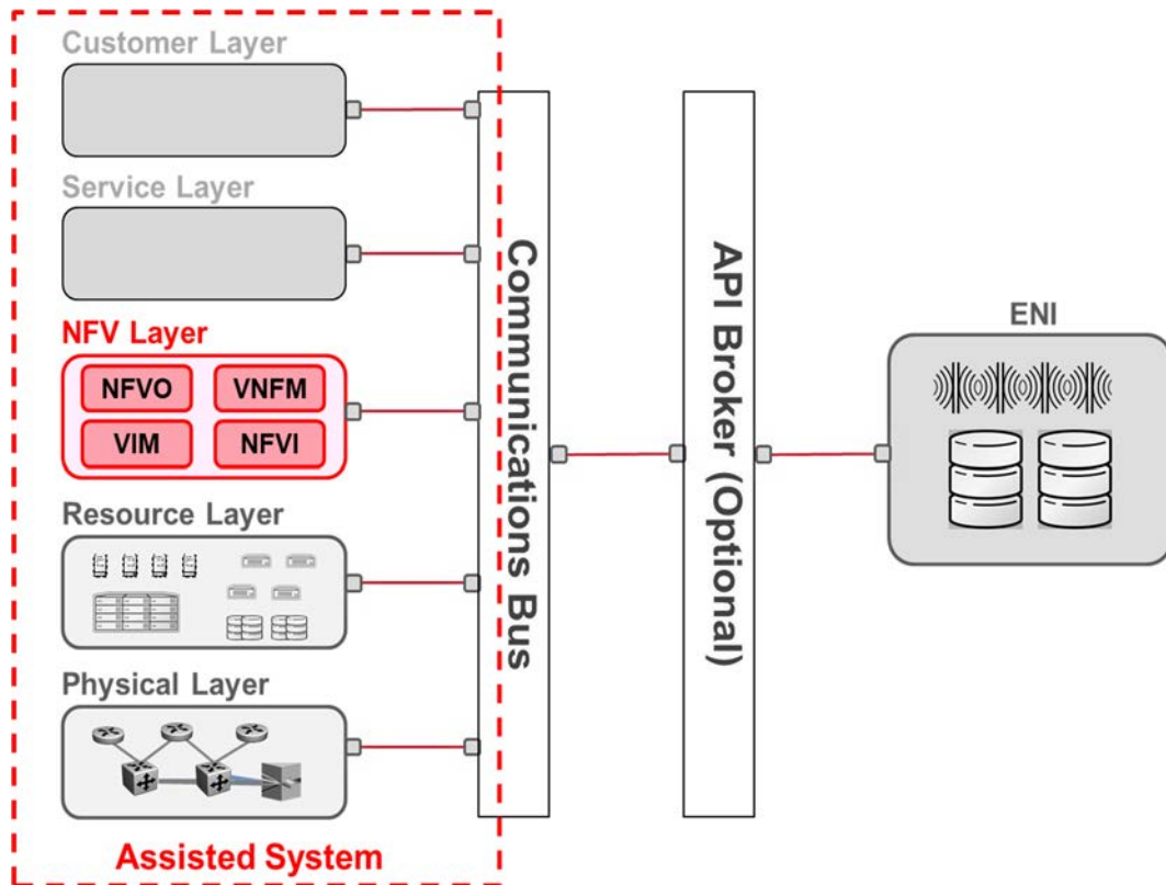
Figure 9-2: Interaction between the NFV MANO and ENI
