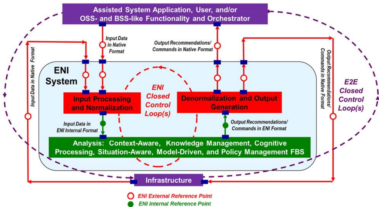
Figure 4-6: High-Level Functional Architecture of ENI When an API Broker is Not Used
