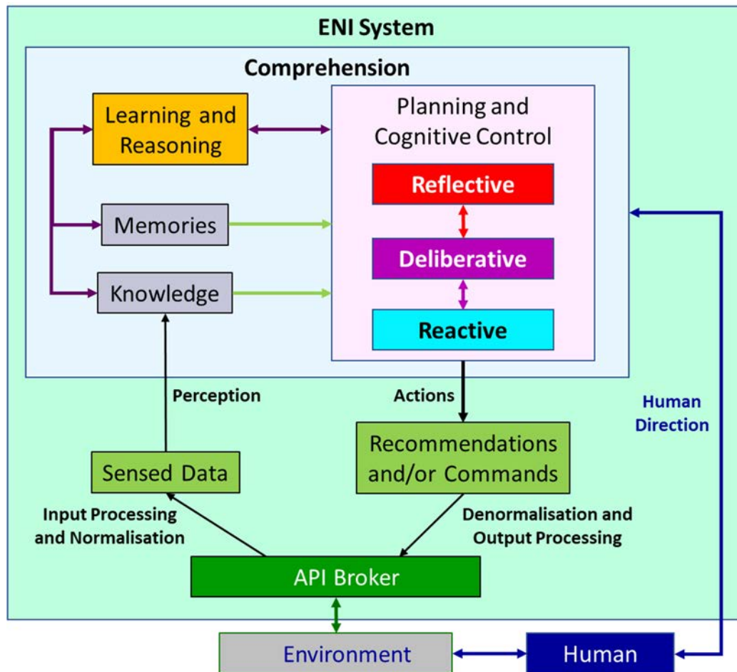
Figure 6-25: A Simplified Functional Architecture using a Cognitive Model
