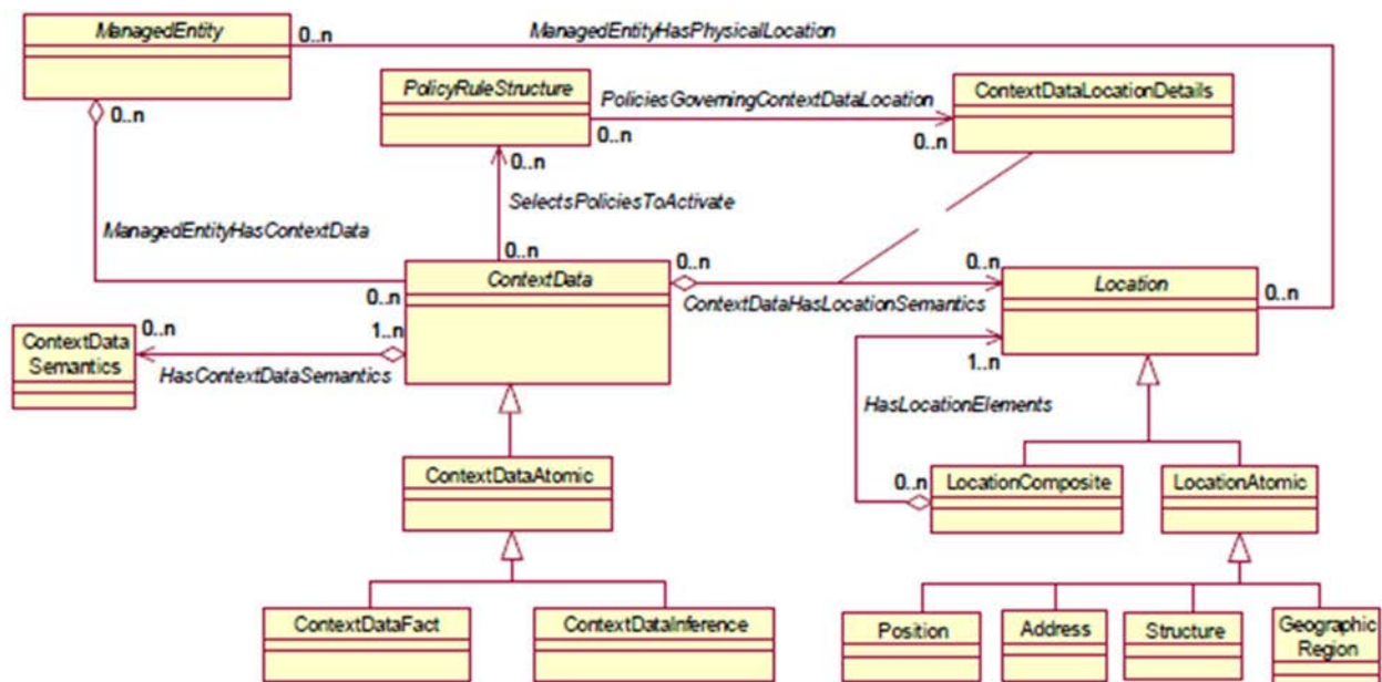
Figure 6-20: Controlling the Semantics of Location ContextData using Policies
