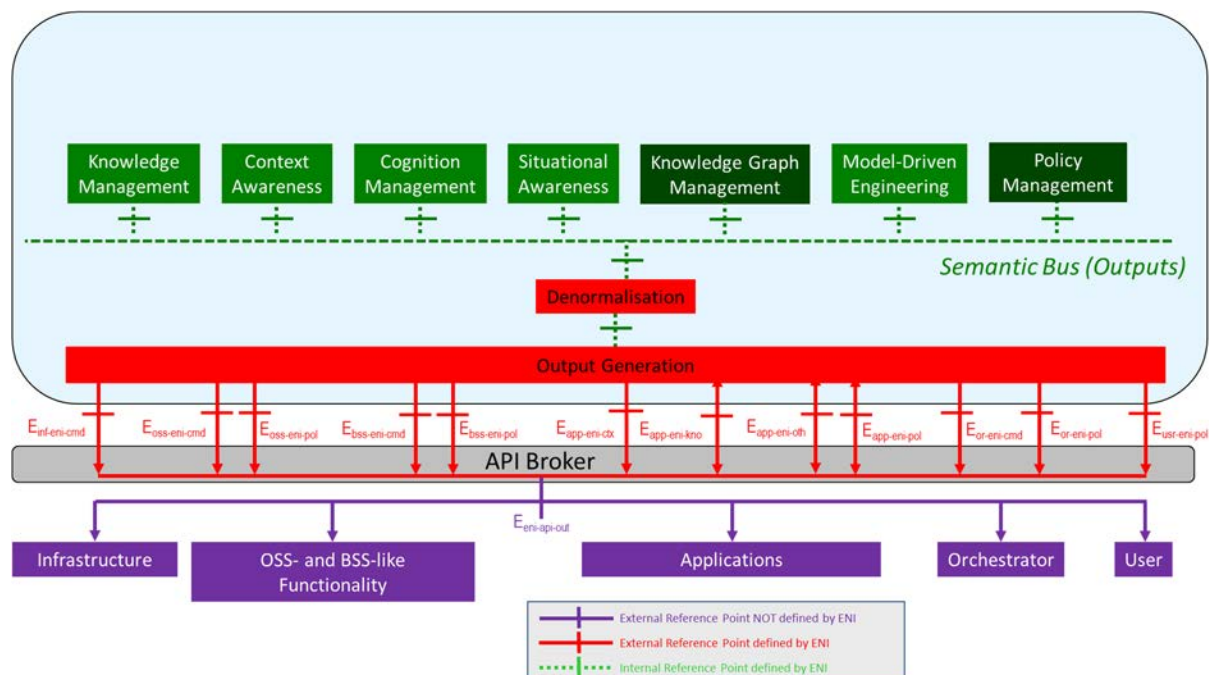
Figure 6-8: Functional Architecture with its Output Reference Points
