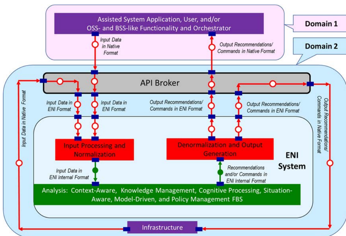
Figure 6-10a: Functional Architecture with An External Exemplary Domain
