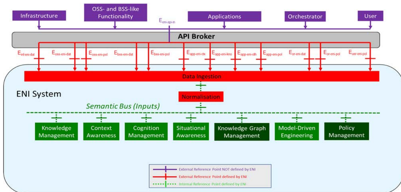
Figure 6-7: Functional Architecture with its Input Reference Points
