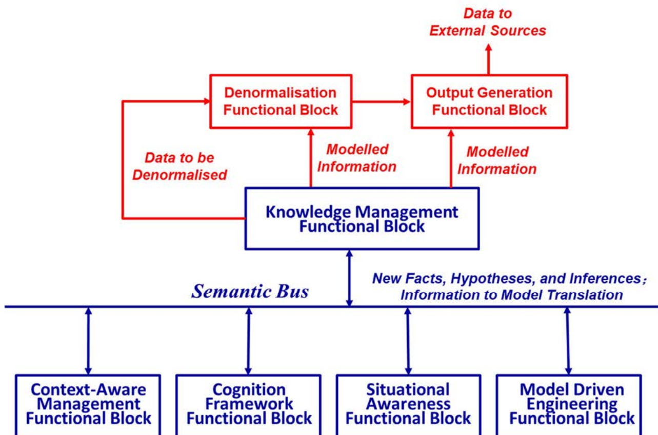
Figure 6-37: Data Denormalization Operation
