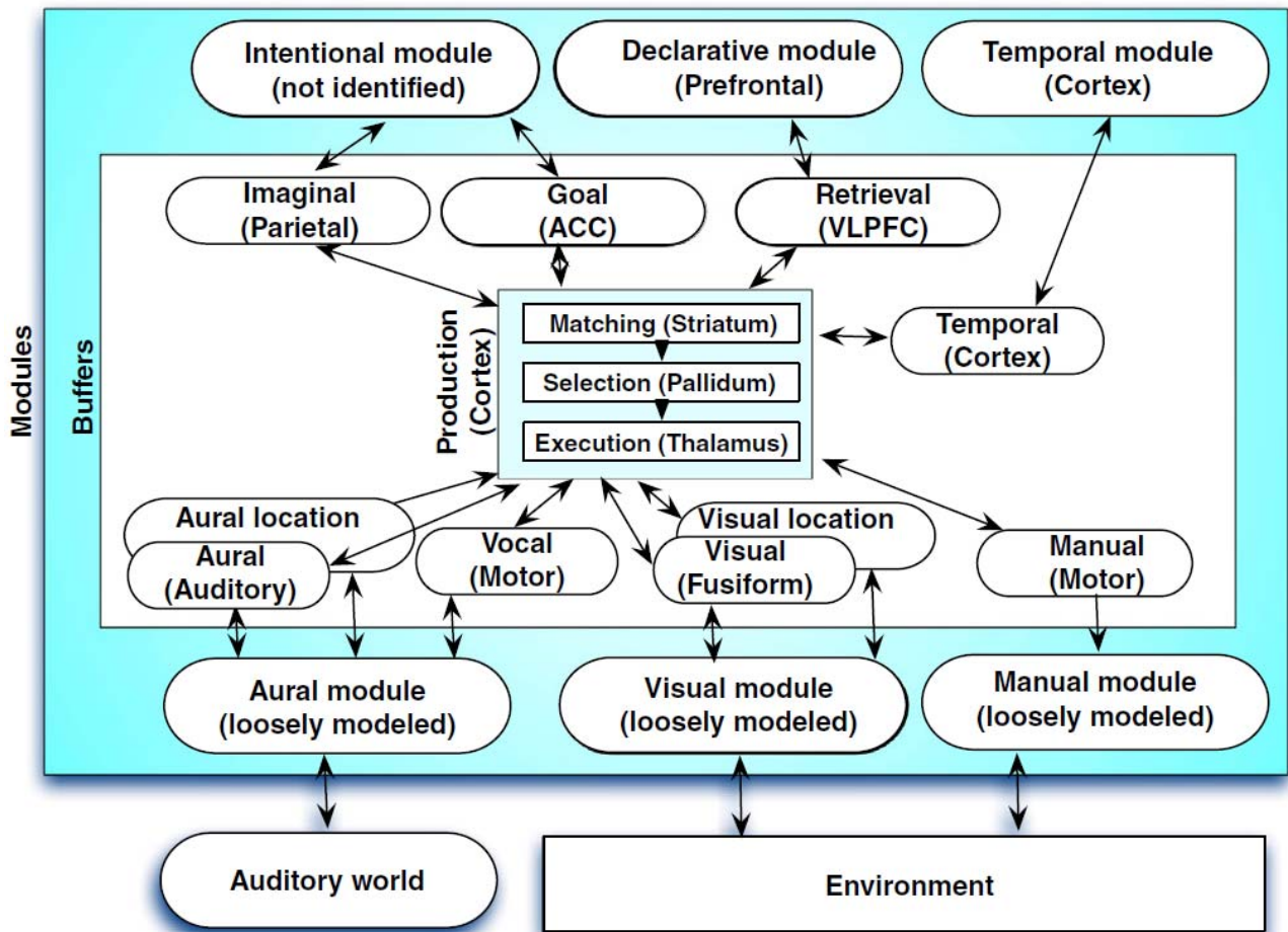
Figure 6-23: The ACT-R Cognitive Architecture
