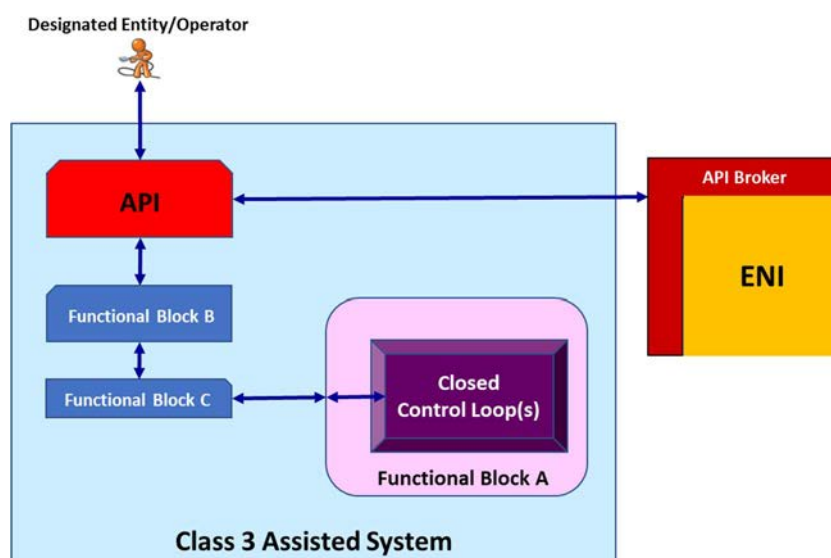
Figure 6-4: API of Single Class 3 Assisted System Indirectly Affect Closed Control Loop
