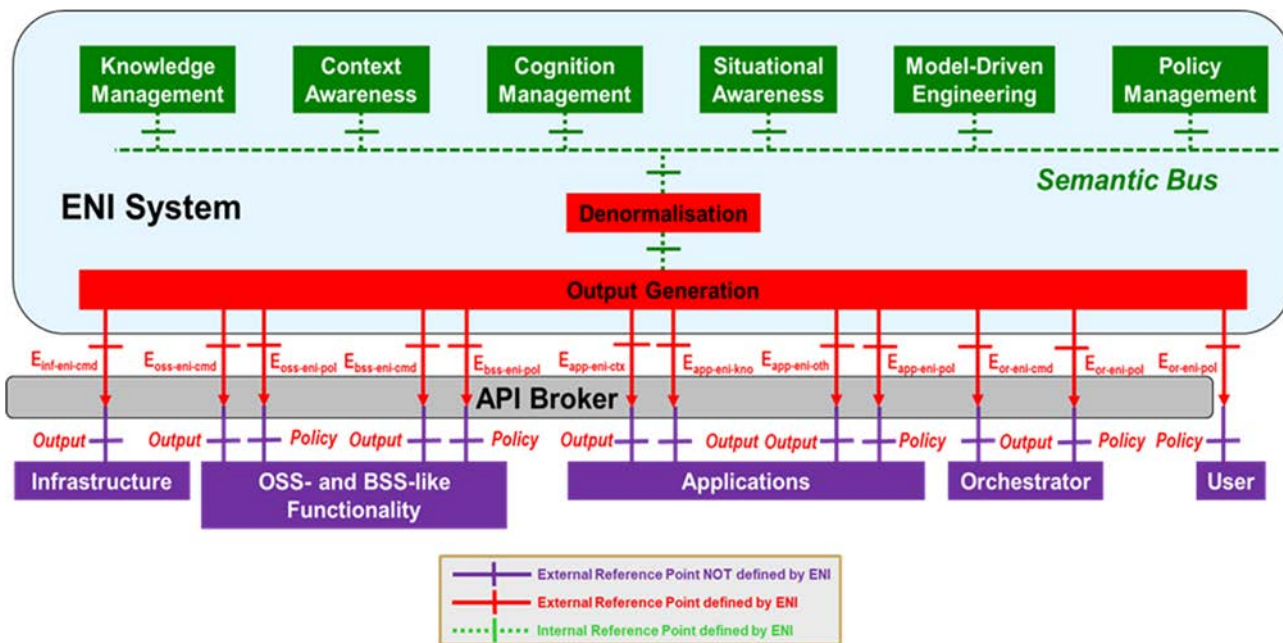
Figure 7-2: Overview of the ENI External Facing External Reference Points
