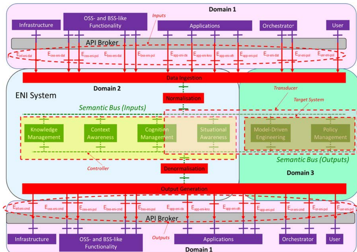
Figure 6-12: Functional Architecture with Exemplary Domains and Control Loops
