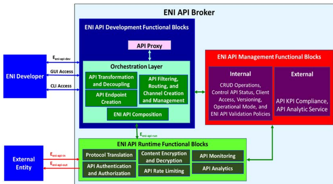
Figure 7-6: Overview of the ENI API Broker Internal Architecture
