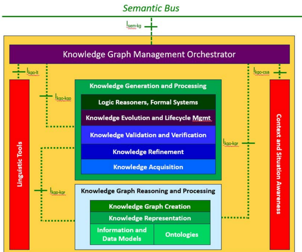
Figure 7-8: Second-Level Knowledge Graph Internal Reference Points
