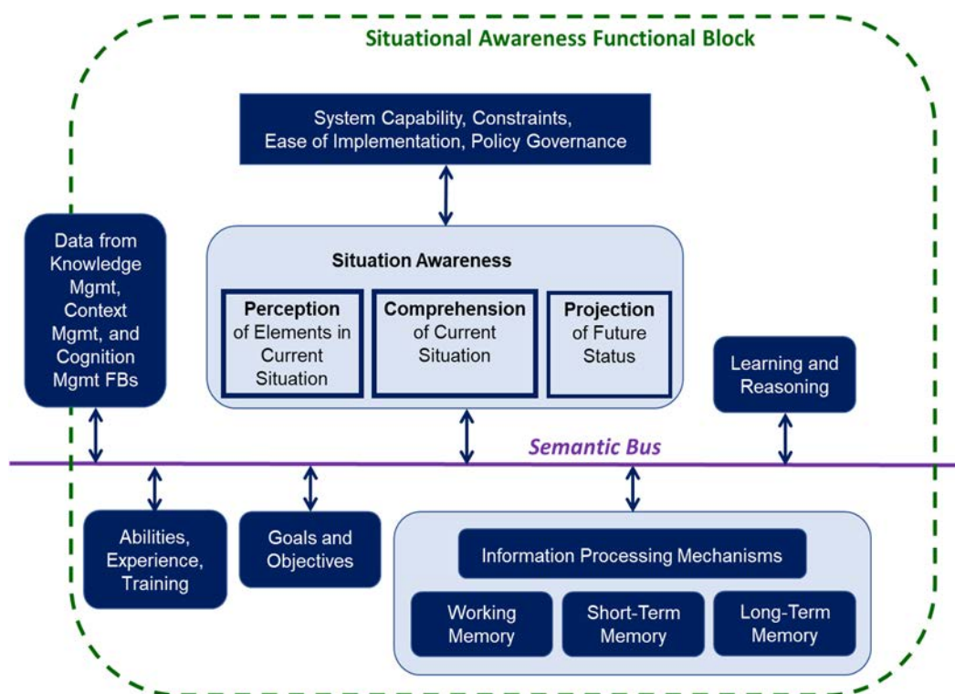
Figure 6-27: A Simplified Cognitive Processing Architecture using Neural Networks
