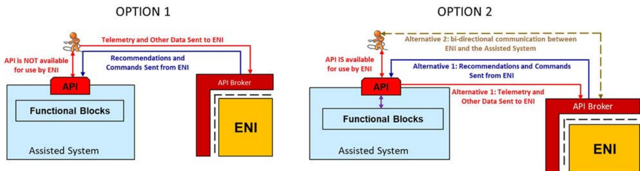
Figure 4-1: Two Common Communication Options of Classes of the Assisted System
