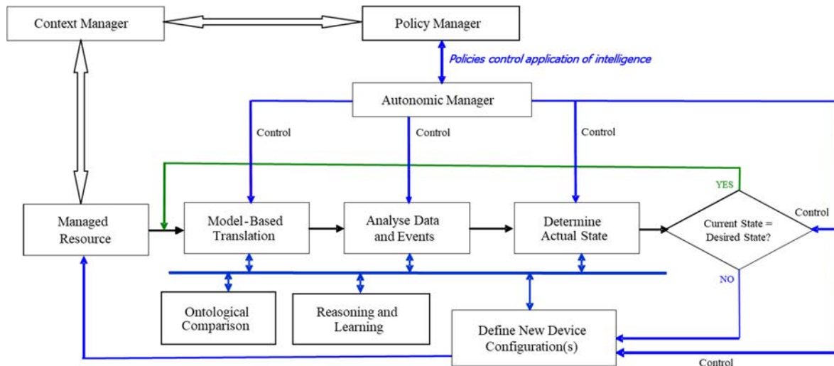
Figure 6-36: Simplified Functional Block Diagram of the FOCAL Architecture
