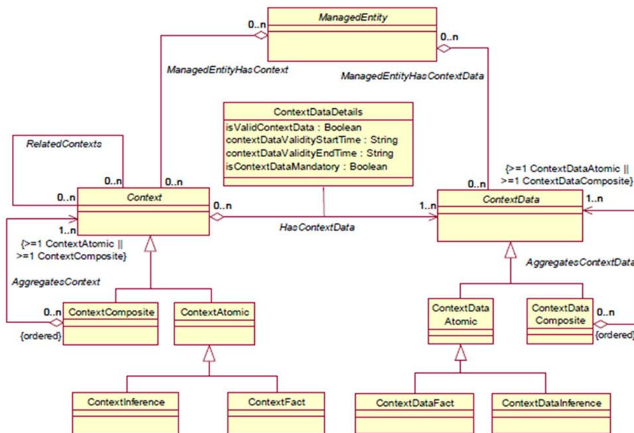
Figure 6-19: Foundation of the DEN-ng Context Model
