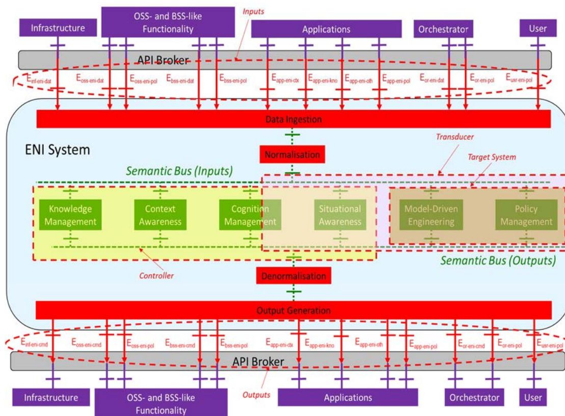
Figure 6-11: Functional Architecture with Exemplary Control Loops
