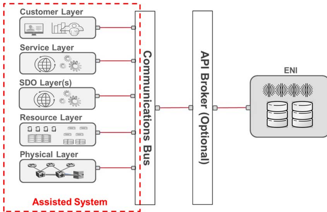
Figure 9-1: Overall view of System Interaction of ENI
