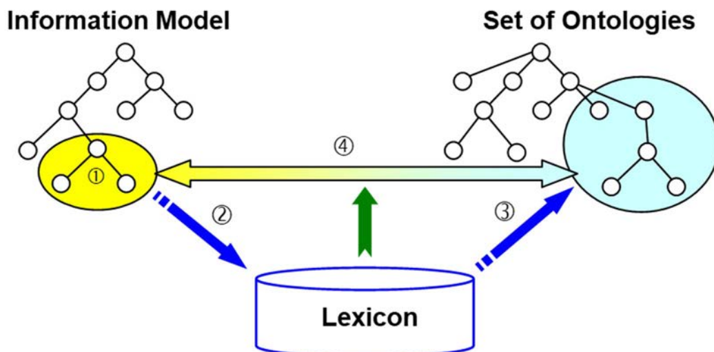
Figure 6-15: Knowledge Representation and Enhancement
