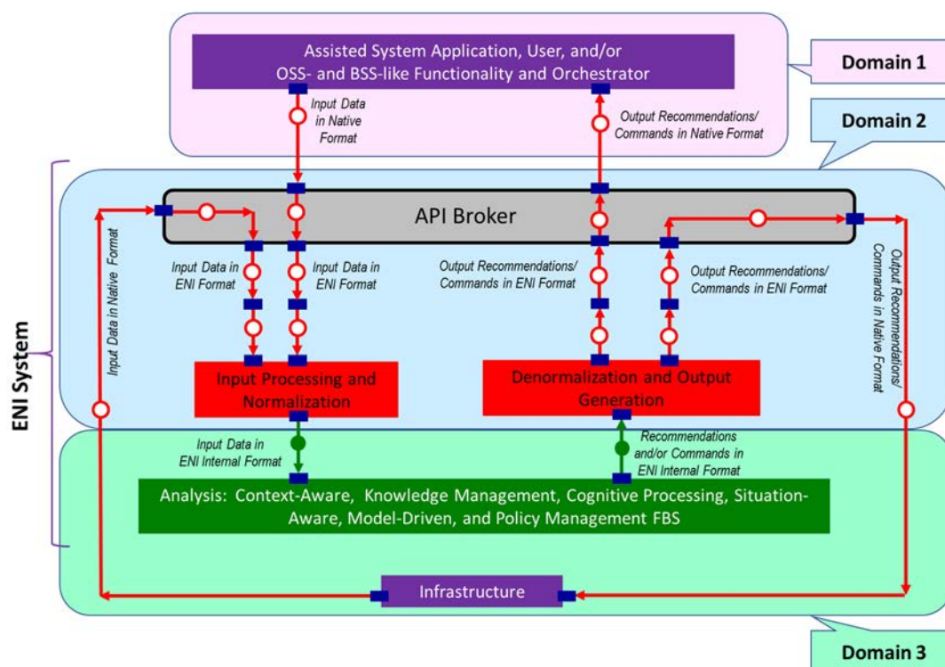
Figure 6-10b: Functional Architecture with Exemplary Internal Domains
