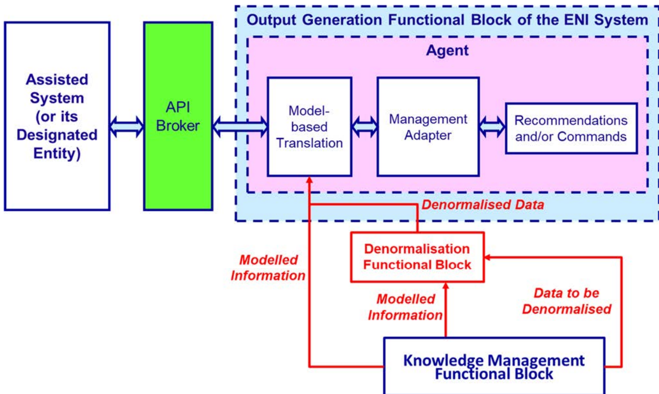
Figure 6-38: Output Generation Operation
