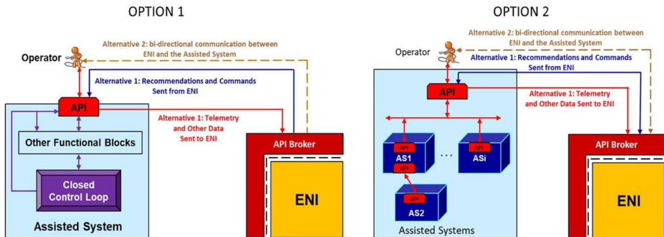
Figure 4-4: Class 3: Assisted System with AI in the Control Loop
