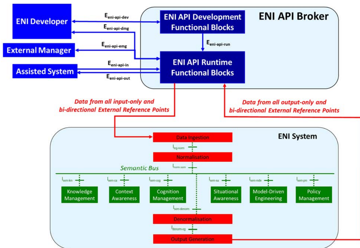
Figure 7-5: ENI API Broker Interaction
