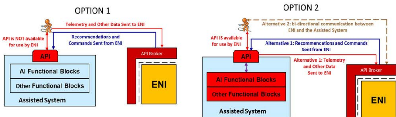
Figure 4-3: Class 2: Assisted System with AI, but Not in the Control Loop
