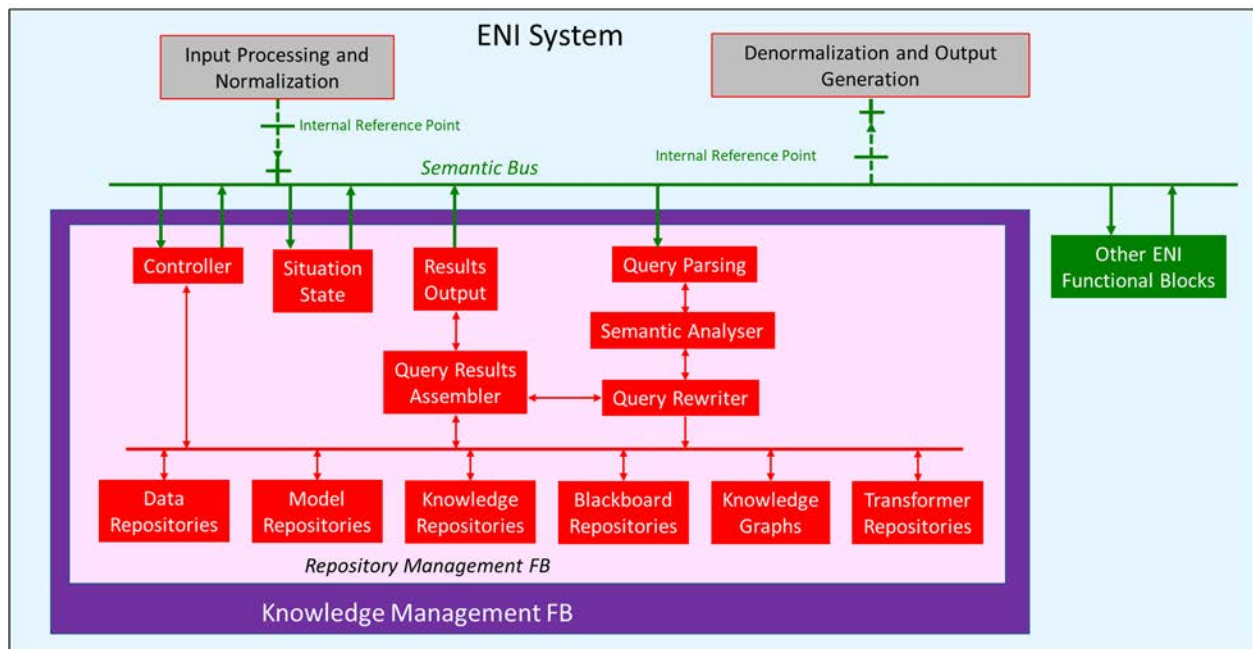
Figure 6-16: Repository Management Functional Block
