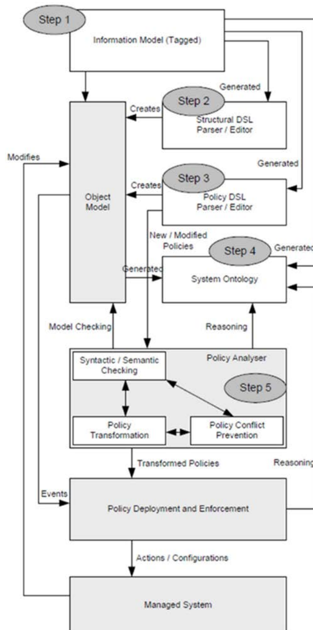
Figure 6-35: Model-Driven Engineering using Policies
