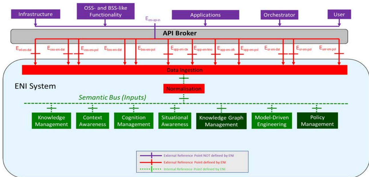
Figure 6-31: Policy Input External Reference Points
