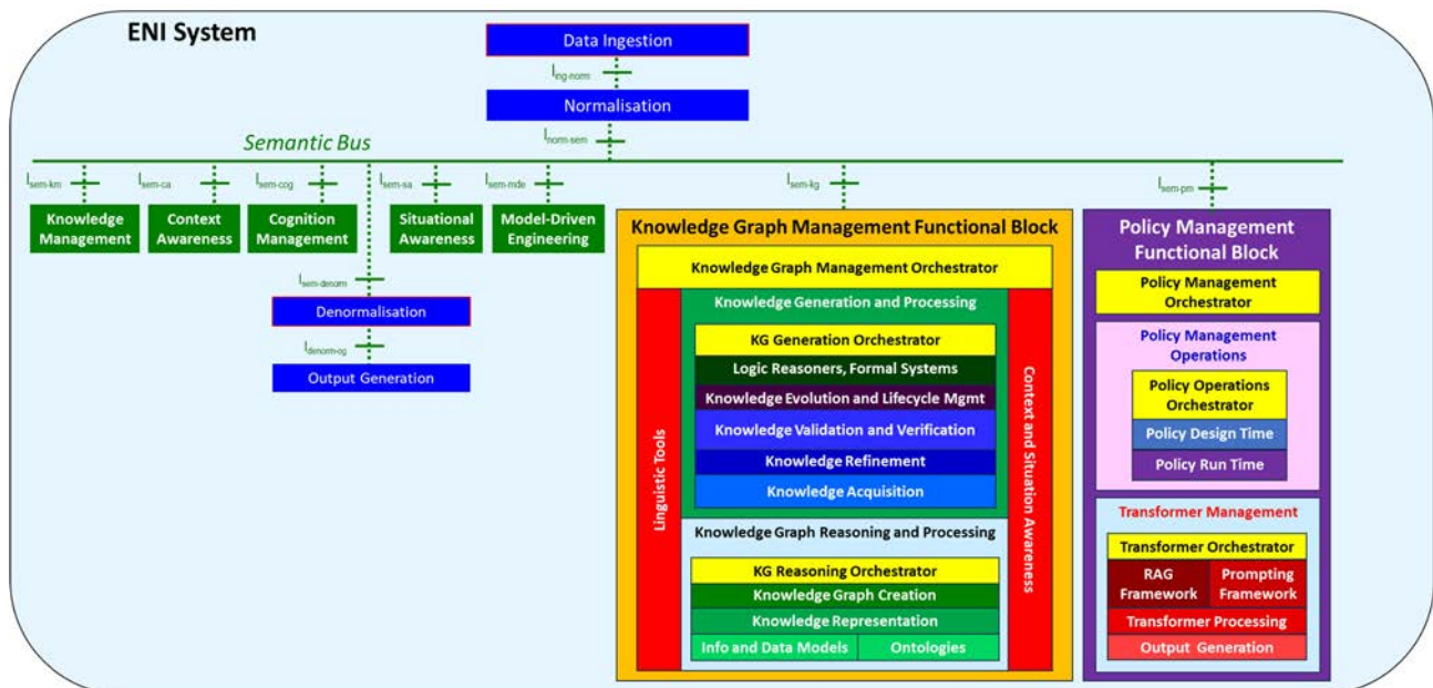
Figure 6-40: Functional Block Diagram of a Cognitive Assistant
