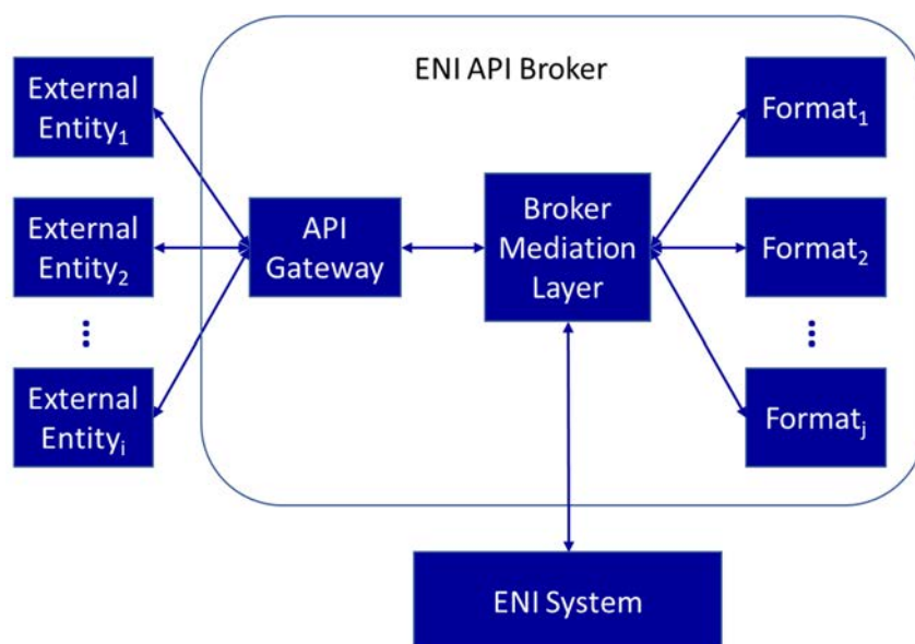
Figure 6-41: Function of the ENI API Broker
