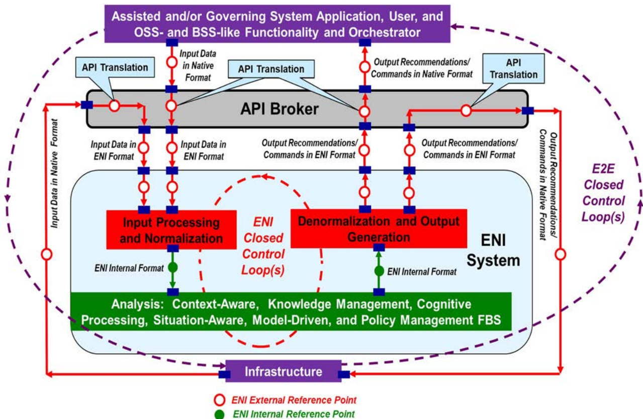
Figure 4-5: High-Level Functional Architecture of ENI When an API Broker Is Used
