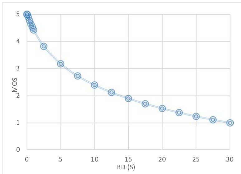
Figure 25: Mapping between IBD and MOS for cloud VR video
