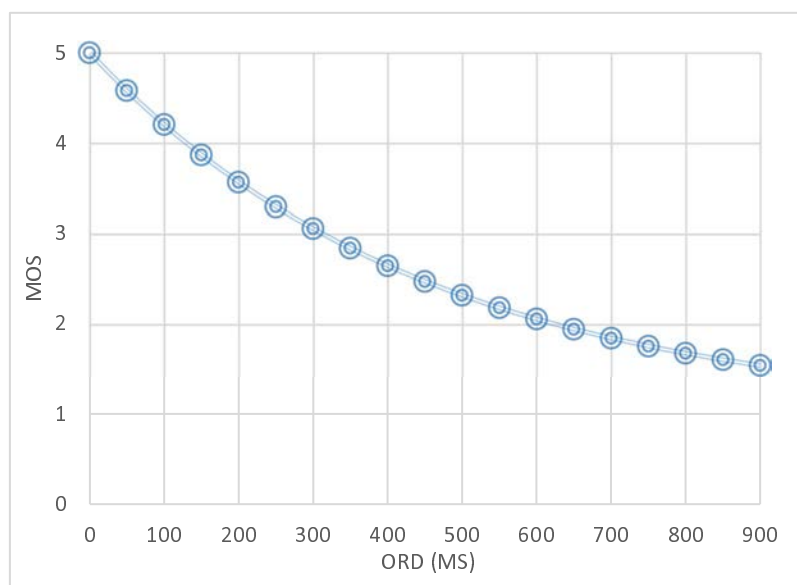
Figure 21: Mapping between the Operation Response Delay (ORD) and MOS
