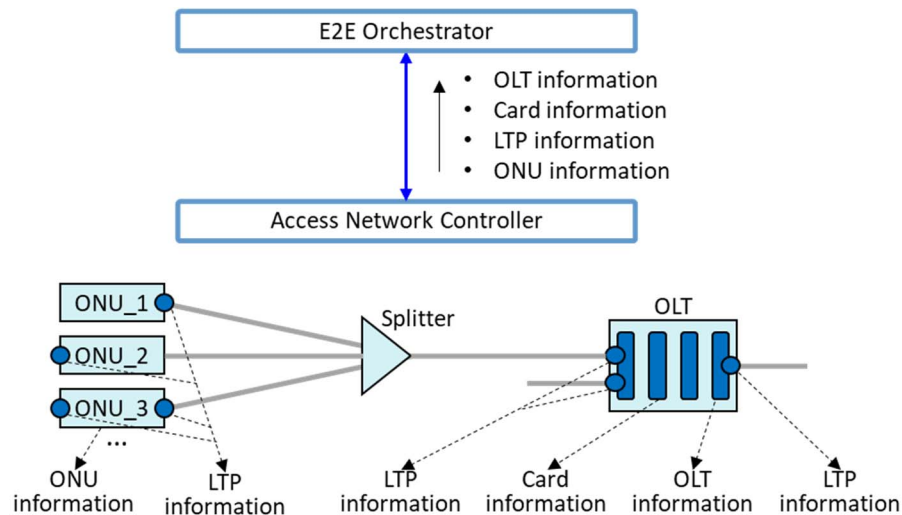
Figure 18: Report of Access Network topology and inventory information
