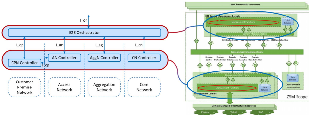
Figure 2: Relationship between the F5G Advanced E2E management and control architecture and the ZSM architecture
