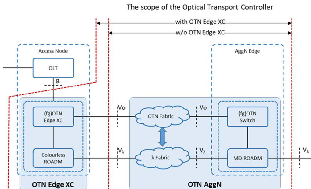
Figure 6: The scope of the Optical Transport Network
