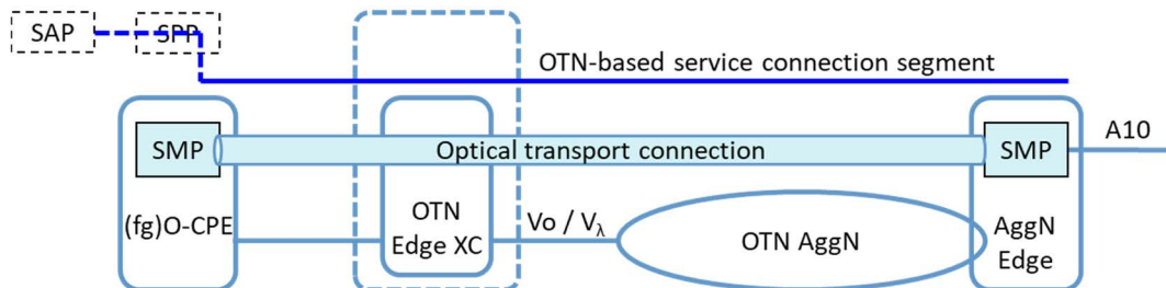
Figure 9: Case 3 - Optical transport connection between CPE and AggN Edge
