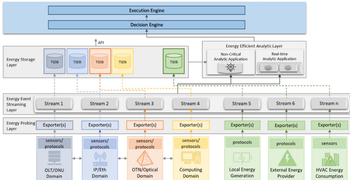
Figure 29: Key components of distributed energy efficiency management system
