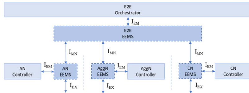
Figure 28: F5G-A distributed energy efficiency management system
