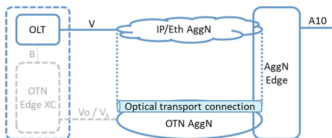
Figure 7: Case 1 - Optical transport connection inside OTN AggN
