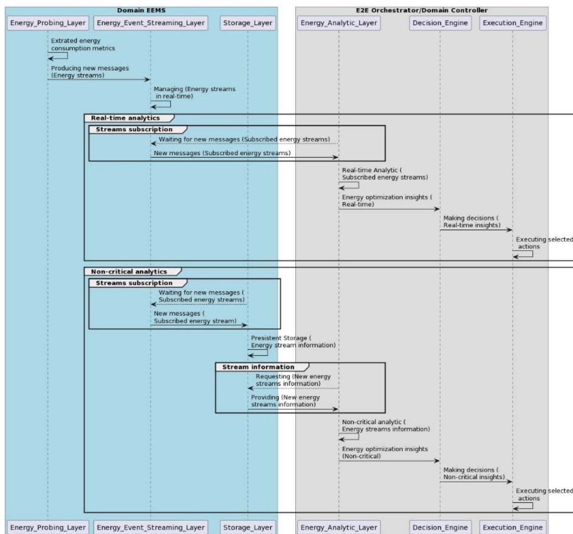
Figure 30: The diagram represents the workflow of monitored information in Scenario 1
