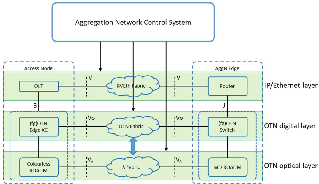
Figure 13: Aggregation Network Controller for multi-layer AggN
