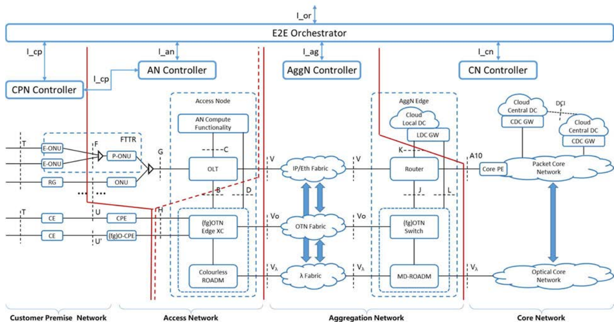
Figure 1: F5G Advanced E2E management and control architecture
