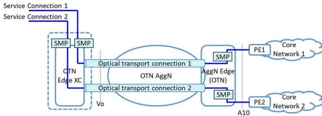
Figure 11: Examples of mapping service connections into optical transport connections
