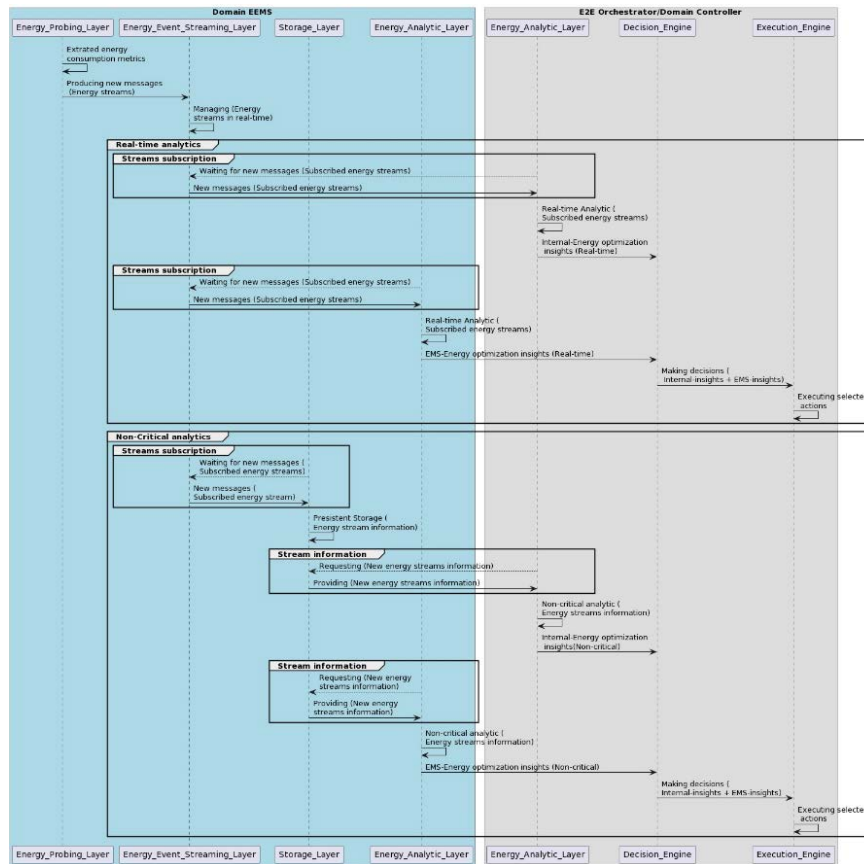
Figure 32: The diagram represents the workflow of monitored information in Scenario 3
