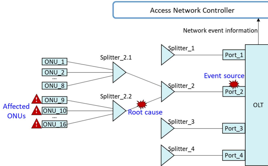
Figure 5: Example of incident-based fault monitoring and troubleshooting
