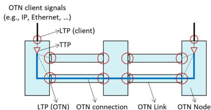
Figure 23: Example OTN network topology
