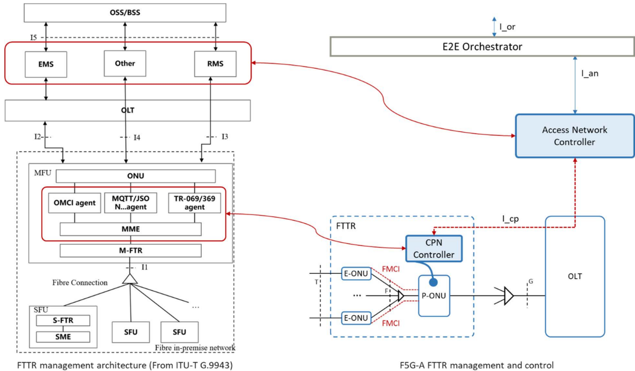
Figure 3: F5G-A FTTR management and control, and the relationship with ITU-T G.9943 [10]
