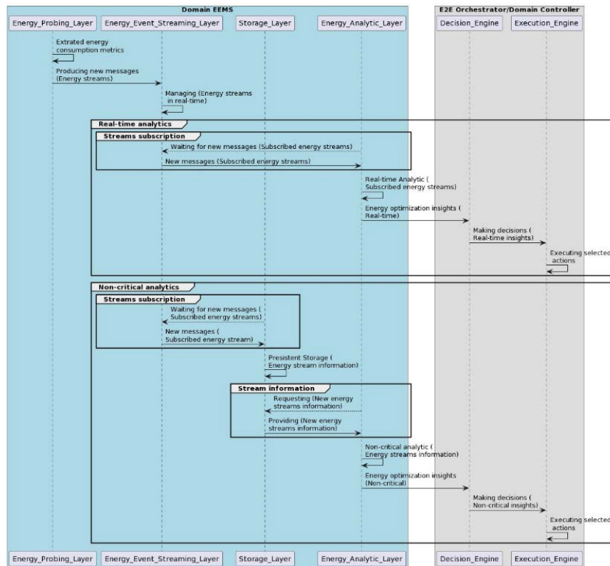
Figure 31: The diagram represents the workflow of monitored information in Scenario 2
