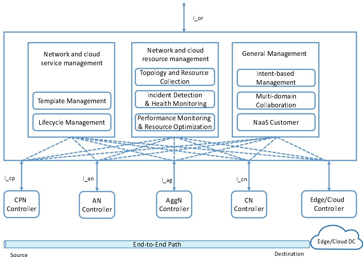
Figure 16: Overview of the E2E Orchestrator
