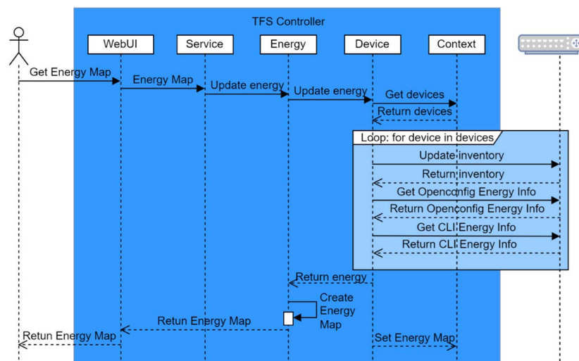
Figure A.1: Energy Map on Demand workflow
