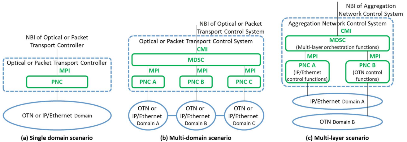
Figure 15: Relationship between the Aggregation Network Controller and the ACTN architecture
