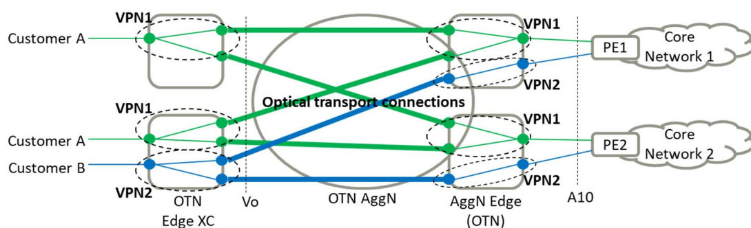
Figure 10: Example VPN configuration
