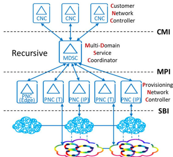
Figure 14: ACTN architecture
