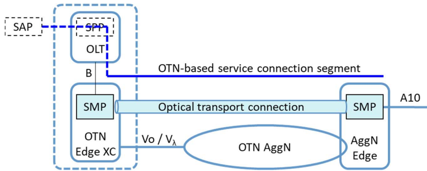
Figure 8: Case 2 - Optical transport connection between Access Network and AggN Edge
