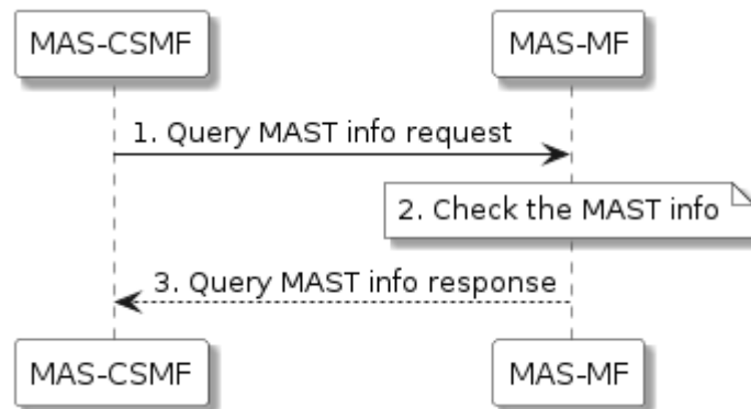
Figure 9.2.4-1: Query MEC Application Slice Template
