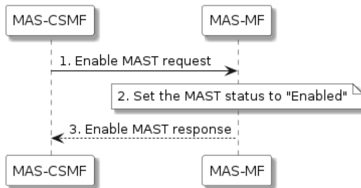
Figure 9.2.3-1: Enable MEC Application Slices template
