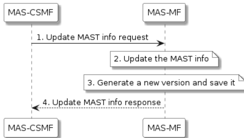
Figure 9.2.5-1: Update MEC Application Slice Template
