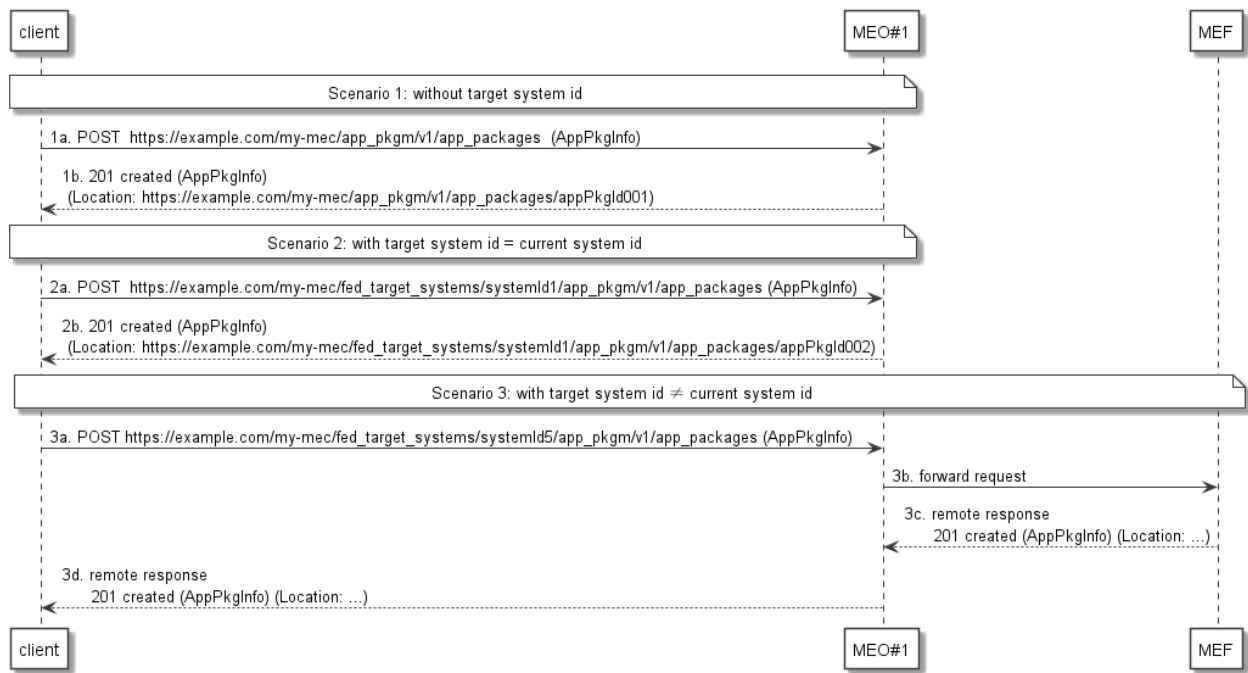
Figure D.2-1: Example scenarios on "create resource"
