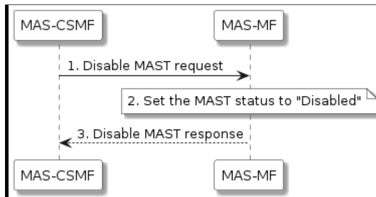
Figure 9.2.2-1: Disable MEC Application Slice Template
