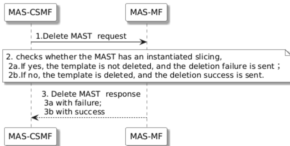
Figure 9.2.6-1: Delate MEC Application Slice Template
