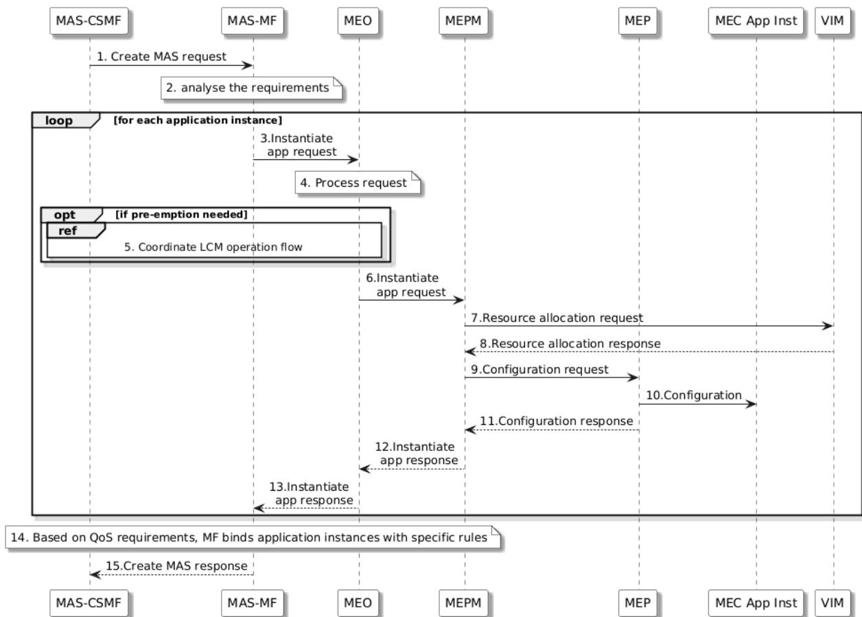
Figure 9.3.2-1: MAS creation flow
