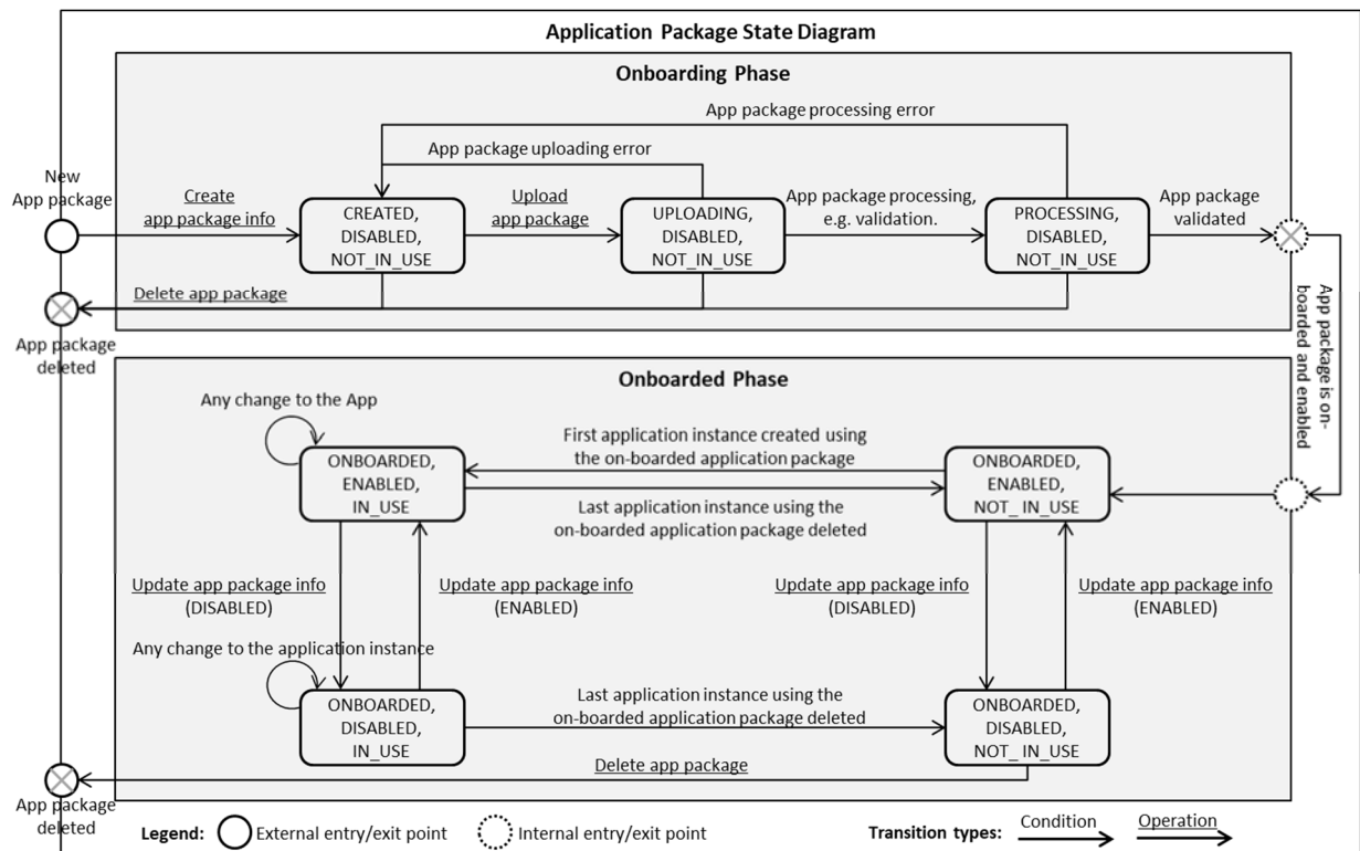
Figure A.2-1: Application package state model
