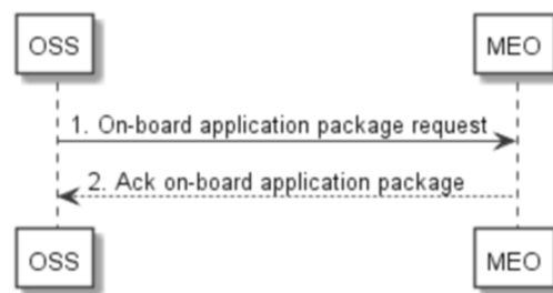
Figure 5.2.2-1: On-board application package
