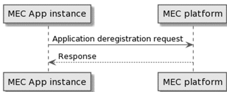
Figure 5.2.13.4-1: Flow of MEC application deregistration
